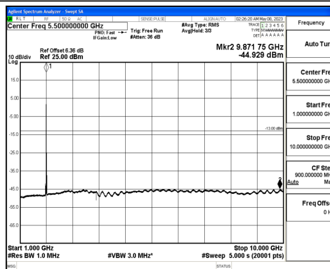
Band2-15MHz-16QAM-19125-1RB#0-Range5:10000~20000MHz
