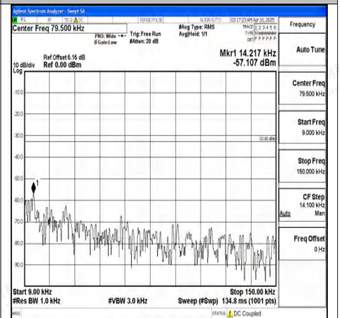
Band5_3MHz_16QAM_20635_1RB#0_0.009~0.15_0.009~0.15
