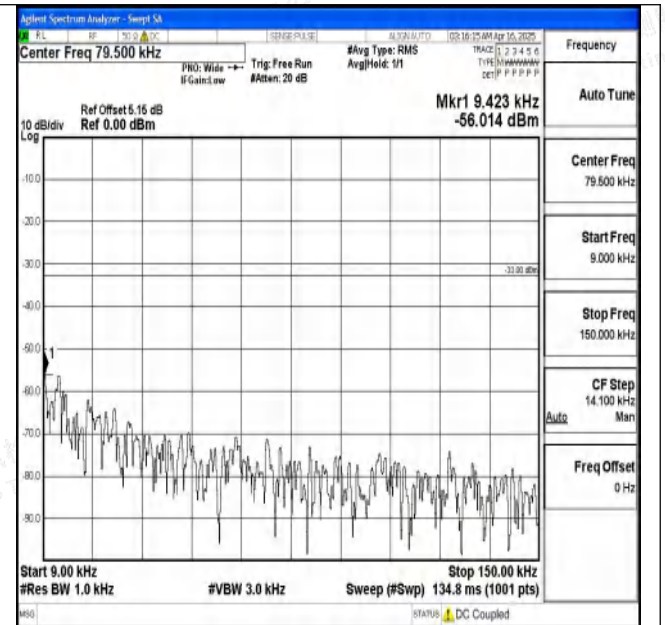
Band5_3MHz_16QAM_20525_1RB#0_0.009~0.15_0.009~0.15
