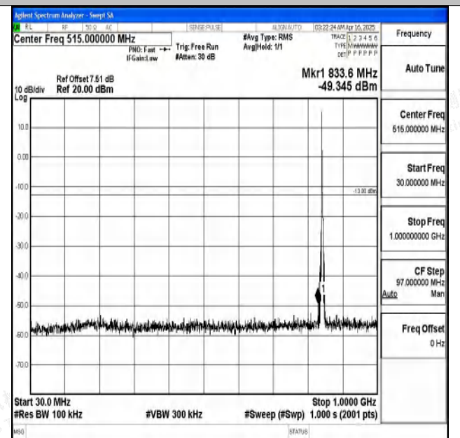
Band5_5MHz_16QAM_20625_1RB#0_30~1000_30~1000
