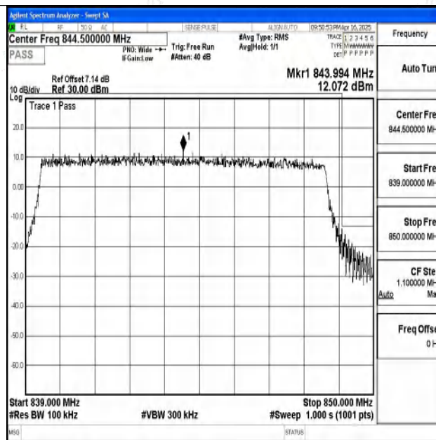
Band5_10MHz_QPSK_20600_50RB#0
