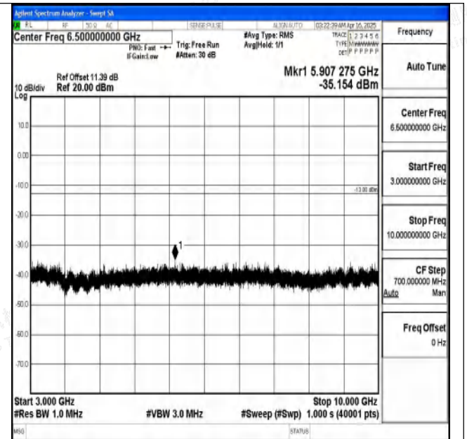
Band5_5MHz_16QAM_20625_1RB#0_3000~10000_3000~10000
