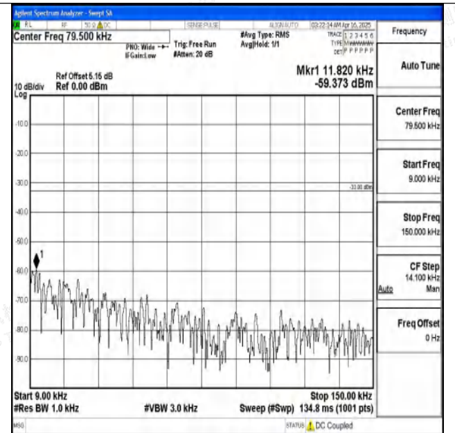
Band5_5MHz_16QAM_20625_1RB#0_0.009~0.15_0.009~0.15
