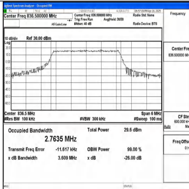
Band5-3MHz-16QAM-20525-15RB#0-PASS
