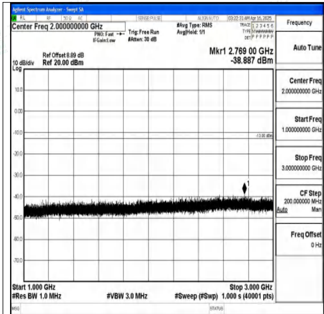
Band5_5MHz_16QAM_20625_1RB#0_1000~3000_1000~3000
