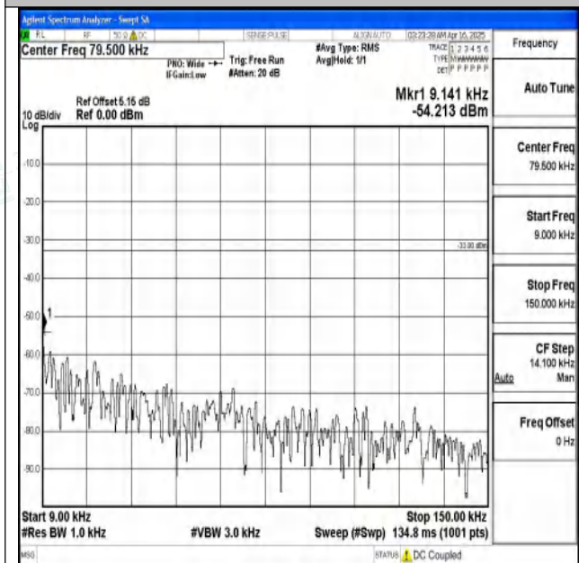
Band5_10MHz_QPSK_20450_1RB#0_0.009~0.15_0.009~0.15
