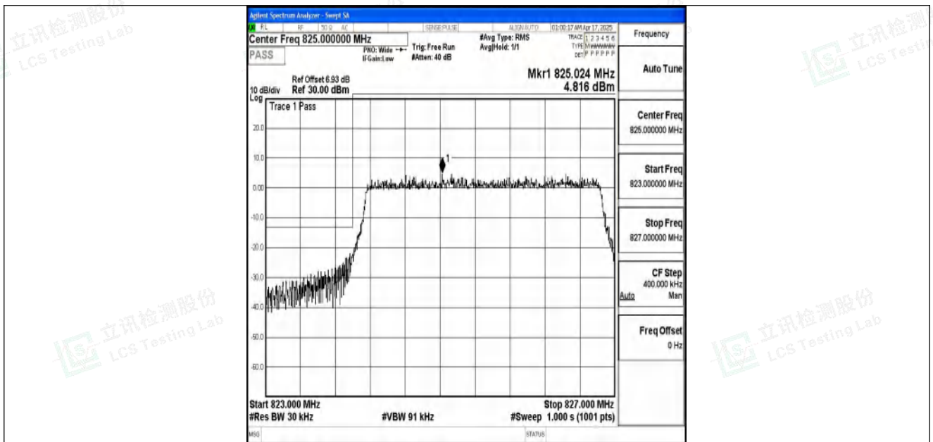
Band5_3MHz_16QAM_20415_15RB#0
