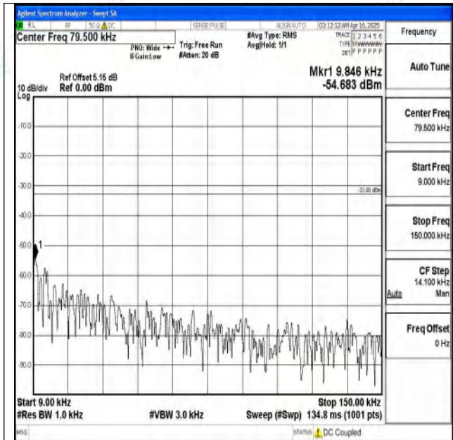
Band5_1.4MHz_QPSK_20643_1RB#0_0.009~0.15_0.009~0.15
