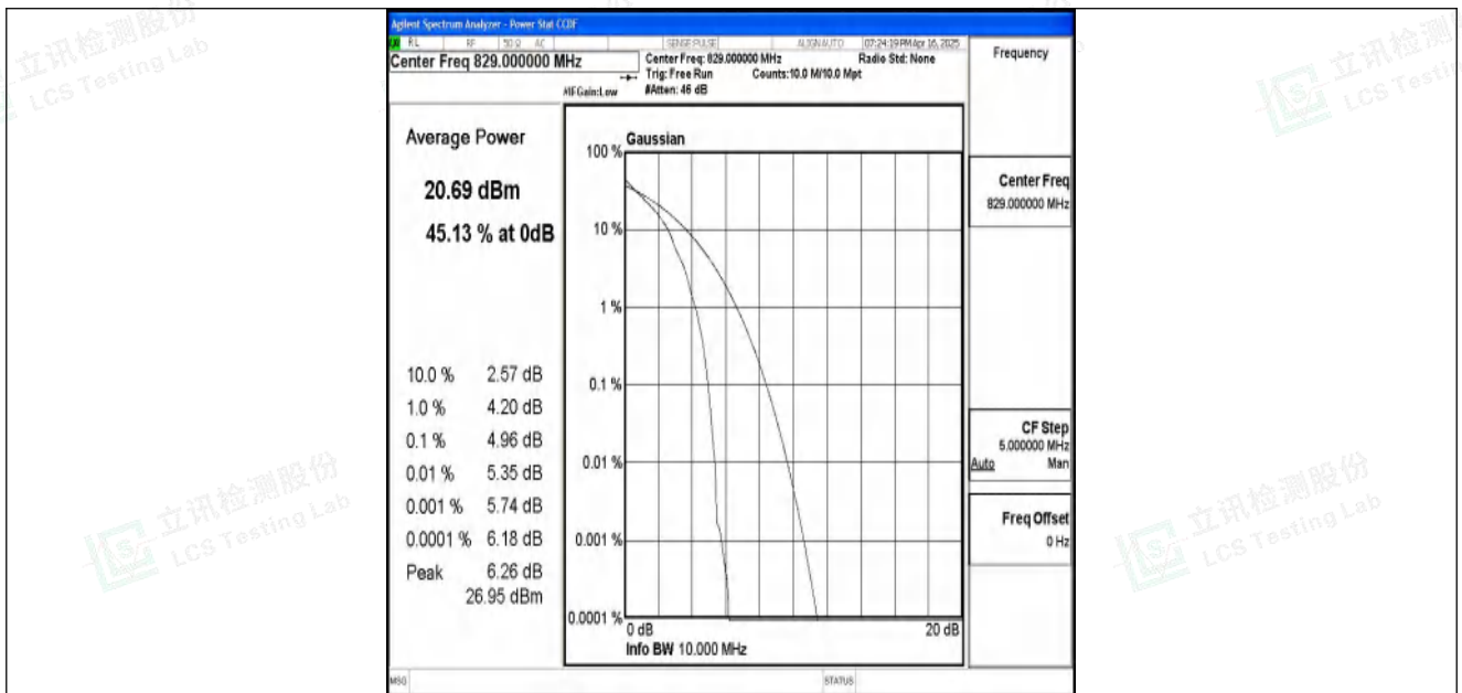
Band5-10MHz-QPSK-20450-1RB#0-PASS
