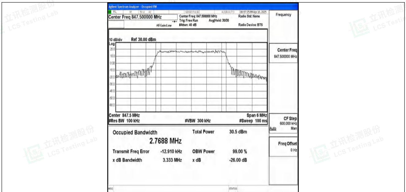
Band5-3MHz-QPSK-20635-15RB#0-PASS
