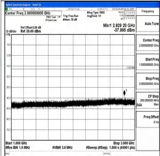
Band5_3MHz_16QAM_20415_1RB#0_1000~3000_1000~3000
