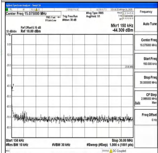
Band5_3MHz_16QAM_20525_1RB#0_0.15~30_0.15~30
