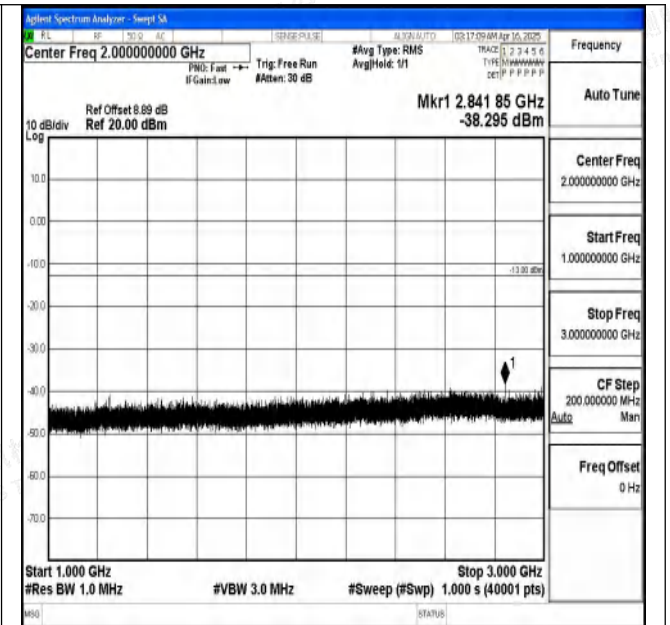
Band5_3MHz_QPSK_20635_1RB#0_1000~3000_1000~3000
