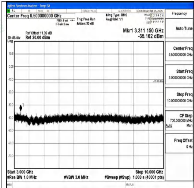
Band5_3MHz_QPSK_20525_1RB#0_3000~10000_3000~10000
