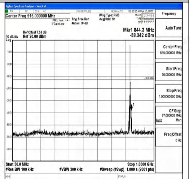
Band5_3MHz_16QAM_20525_1RB#0_30~1000_30~1000
