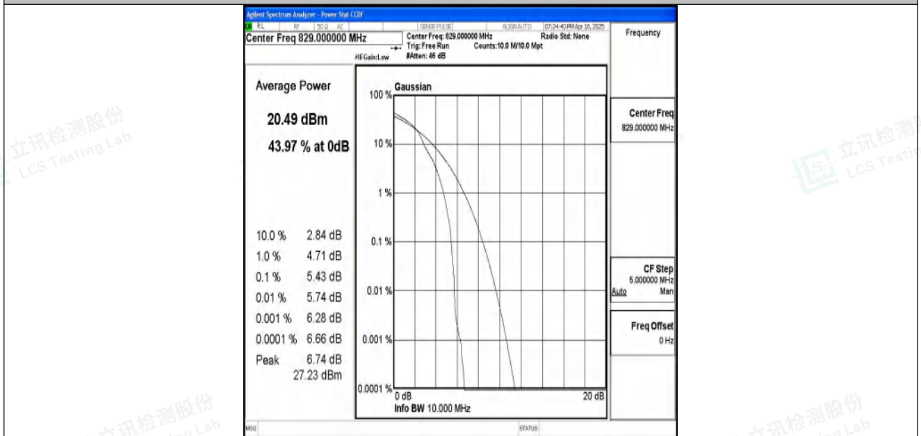
Band5-10MHz-16QAM-20450-1RB#0-PASS
