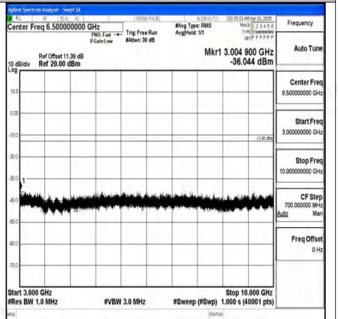
Band5_3MHz_16QAM_20415_1RB#0_3000~10000_3000~10000
