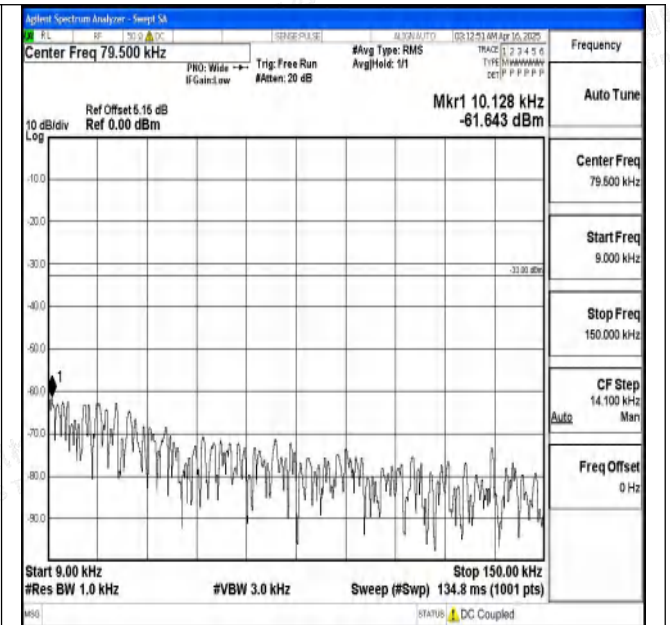
Band5_1.4MHz_16QAM_20643_1RB#0_0.009~0.15_0.009 ~0.15
