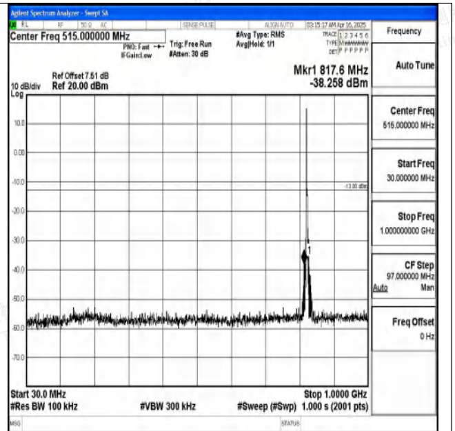
Band5_3MHz_16QAM_20415_1RB#0_30~1000_30~1000
