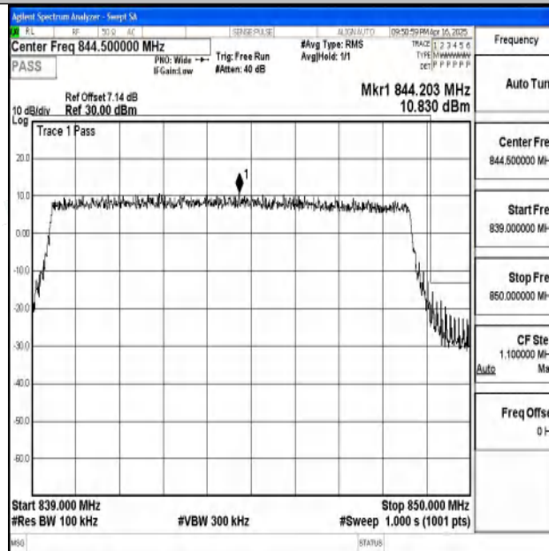
Band5_10MHz_16QAM_20600_50RB#0
