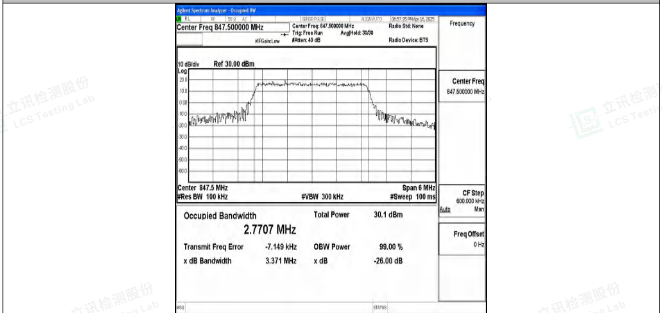
Band5-3MHz-16QAM-20635-15RB#0-PASS
