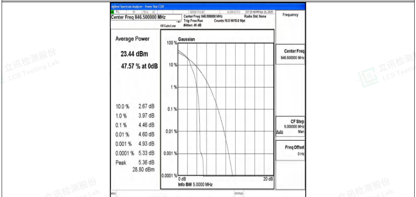
Band5-5MHz-16QAM-20625-1RB#0-PASS
