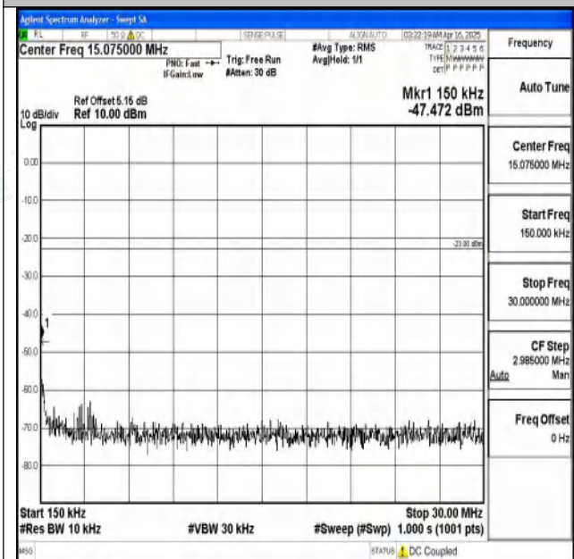
Band5_5MHz_16QAM_20625_1RB#0_0.15~30_0.15~30
