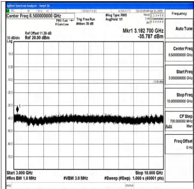
Band5_5MHz_QPSK_20625_1RB#0_3000~10000_3000~10000
