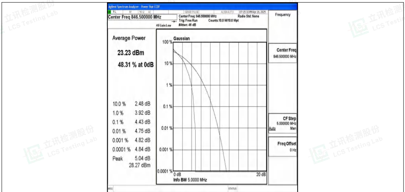
Band5-5MHz-QPSK-20625-1RB#0-PASS
