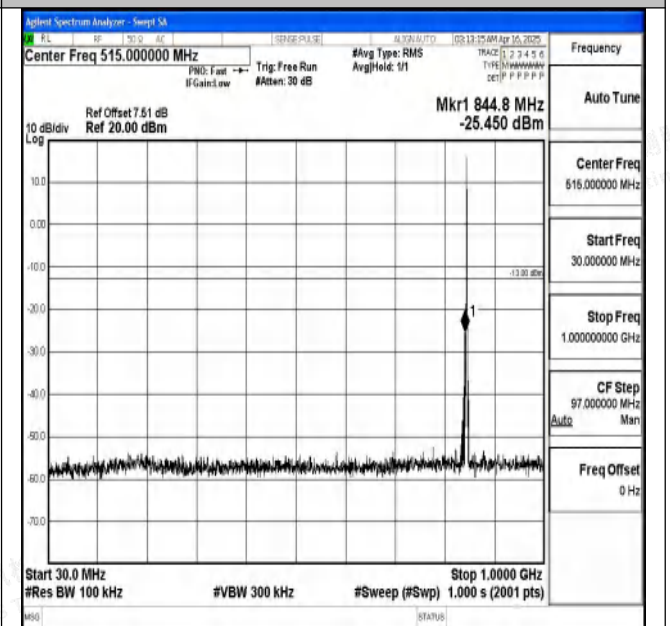
Band5_1.4MHz_16QAM_20643_1RB#0_30~1000_30~100 0
