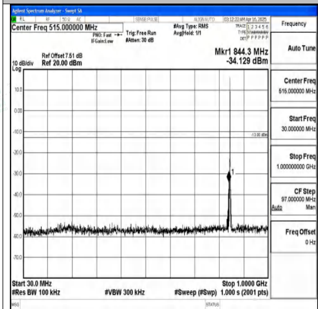
Band5_1.4MHz_QPSK_20643_1RB#0_30~1000_30~1000 0
