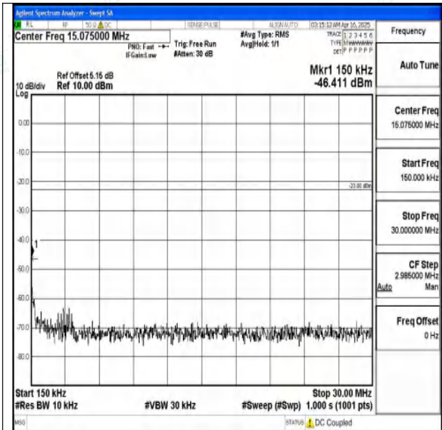
Band5_3MHz_16QAM_20415_1RB#0_0.15~30_0.15~30
