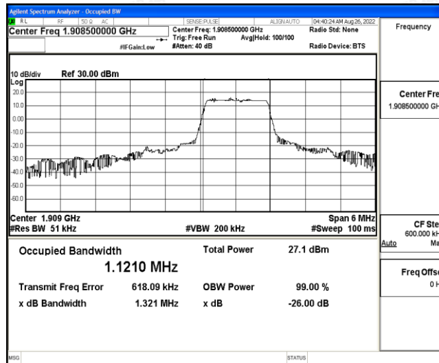
Band2-3MHz-16QAM-19185-6-0-High-1.1210-1.321-PASS
