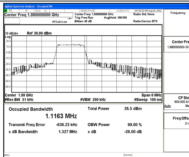
Band2-3MHz-QPSK-18900-6-0-Low-1.1163-1.327-PASS
