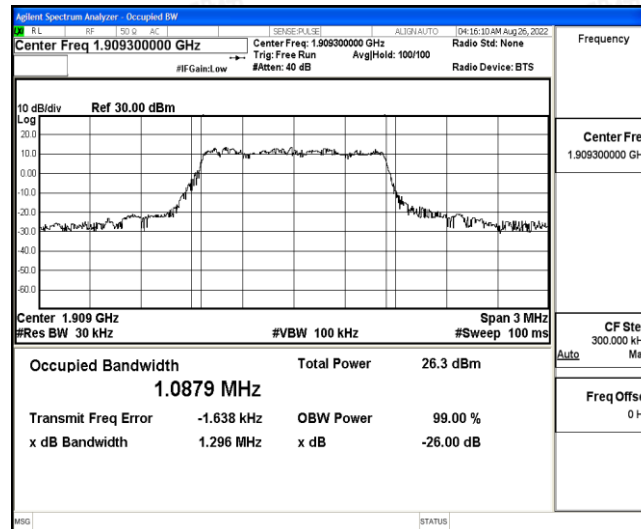
Band2-1.4MHz-16QAM-19193-6-0-High-1.0879-1.296-PASS
