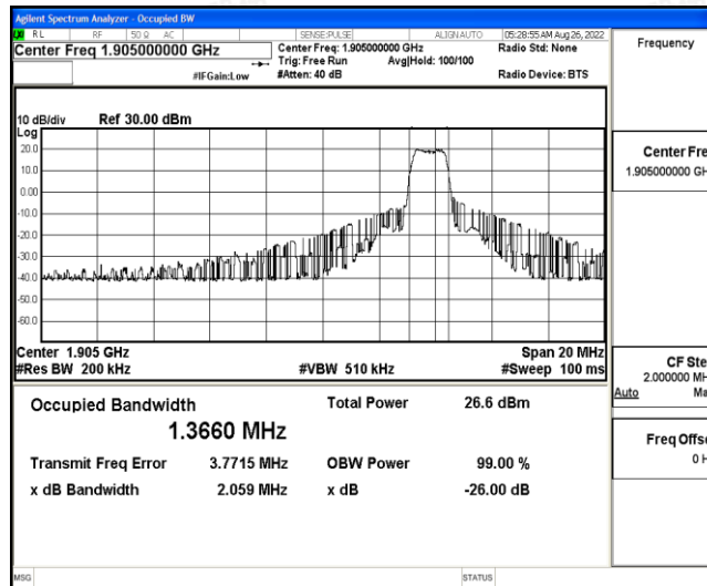
Band2-10MHz-QPSK-19150-6-0-High-1.3660-2.059-PASS
