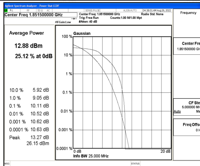
Band2-3MHz-16QAM-18615-6-0-Low-10.11-&lt;=13-PASS
