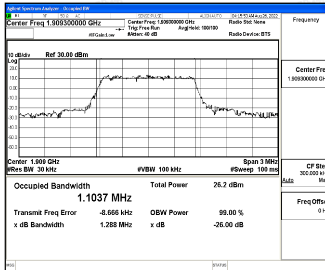
Band2-1.4MHz-QPSK-19193-6-0-High-1.1037-1.288-PASS
