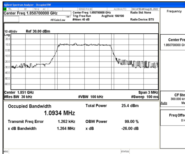
Band2-1.4MHz-16QAM-18607-6-0-Low-1.0934-1.264-PASS
