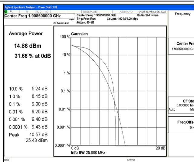
Band2-3MHz-16QAM-19185-6-0-High-9.00-&lt;=13-PASS
