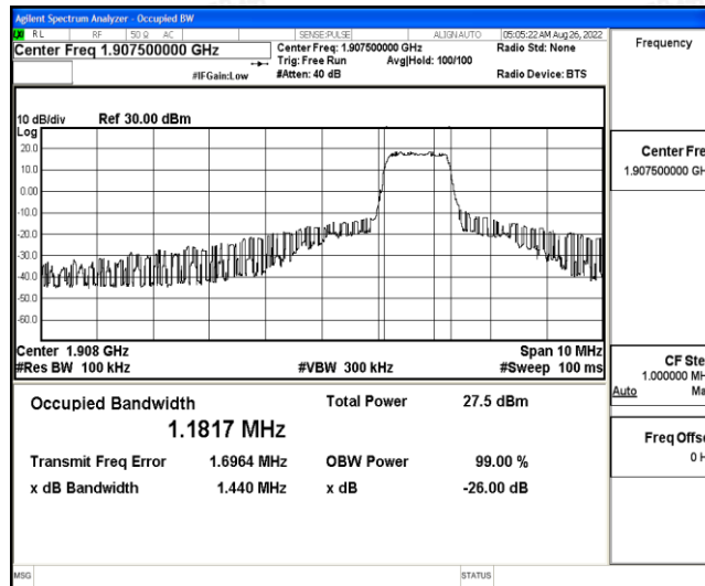
Band2-5MHz-16QAM-19175-6-0-High-1.1817-1.440-PASS
