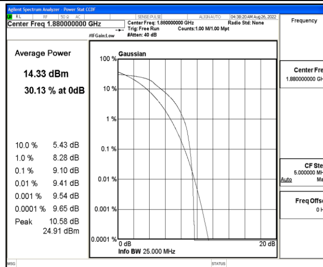
Band2-3MHz-16QAM-18900-6-0-Low-9.10-&lt;=13-PASS
