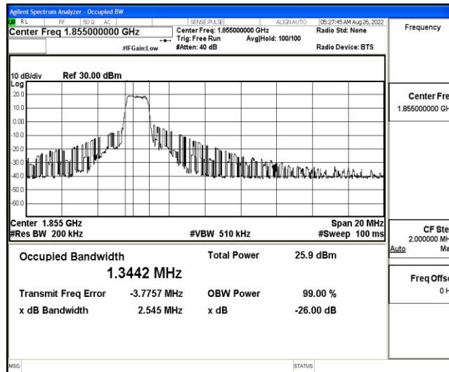
Band2-10MHz-QPSK-18650-6-0-Low-1.3442-2.545-PASS
