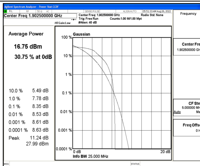
Band2-15MHz-QPSK-19125-6-0-High-8.35-&lt;=13-PASS
