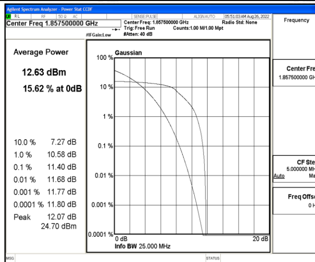
Band2-15MHz-16QAM-18675-6-0-Low-11.40-&lt;=13-PASS
