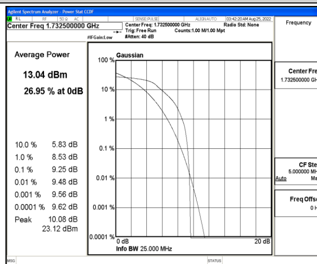
Band4-10MHz-QPSK-20175-6-0-Low-9.25-13-PASS
