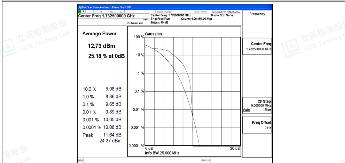
Band4-5MHz-QPSK-20175-6-0-Low-9.65-&lt;=13-PASS
