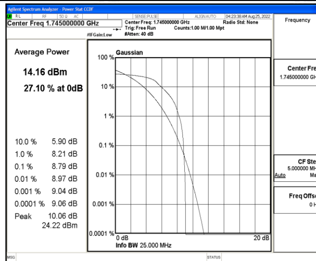
Band4-20MHz-QPSK-20300-6-0-High-8.79-&lt;=13-PASS
