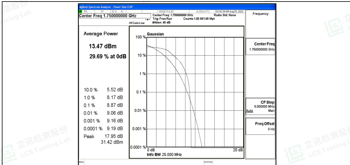
Band4-10MHz-QPSK-20350-6-0-High-8.87-&lt;=13-PASS
