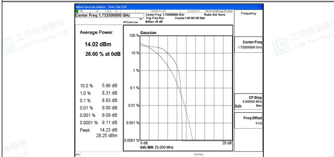
Band4-20MHz-QPSK-20175-6-0-Low-8.83-&lt;=13-PASS
