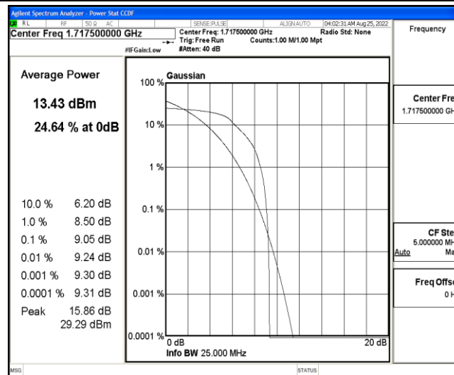
Band4-15MHz-16QAM-20025-6-0-Low-9.05-&lt;=13-PASS
