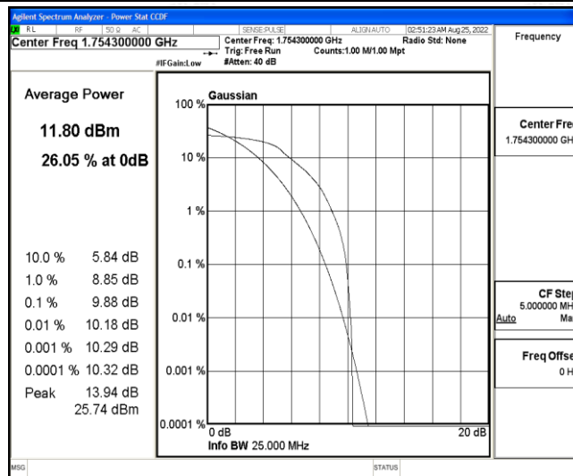
Band4-1.4MHz-16QAM-20393-6-0-High-9.88-&lt;=13-PASS
