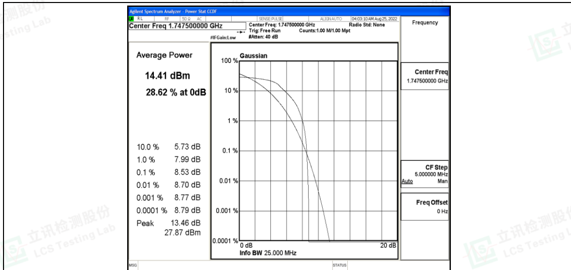
Band4-15MHz-16QAM-20325-6-0-High-8.53-&lt;=13-PASS
