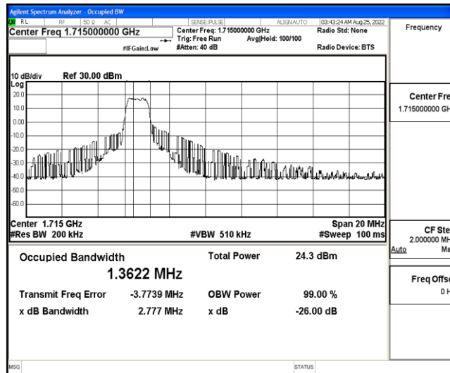
Band4-10MHz-16QAM-20000-6-0-Low-1.3622-2.777-PASS
