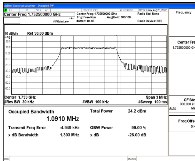
Band4-1.4MHz-QPSK-20175-6-0-Low-1.0910-1.303-PASS
