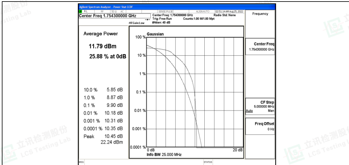
Band4-1.4MHz-QPSK-20393-6-0-High-9.90-&lt;=13-PASS
