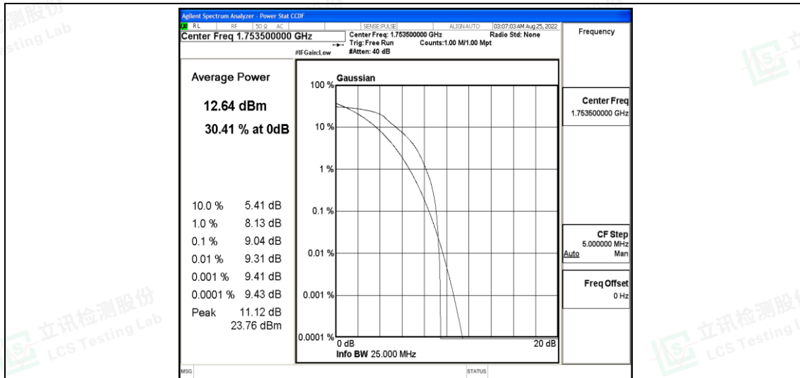
Band4-3MHz-16QAM-20385-6-0-High-9.04-&lt;=13-PASS
