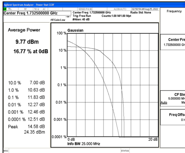
Band4-1.4MHz-QPSK-20175-6-0-Low-11.83-&lt;=13-PASS
