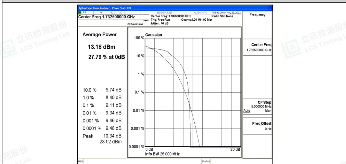
Band4-10MHz-16QAM-20175-6-0-Low-9.11-&lt;=13-PASS
