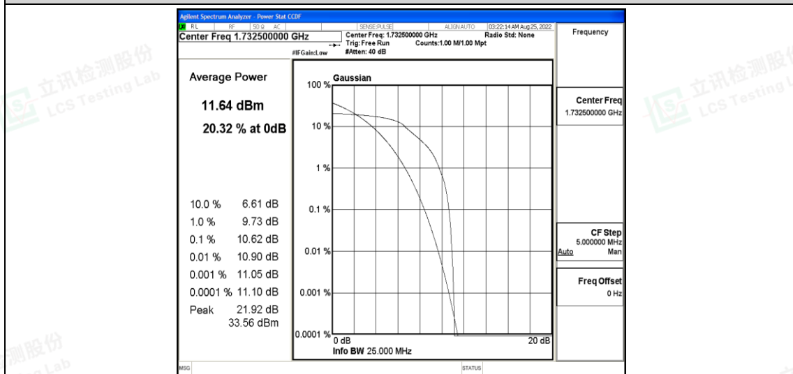
Band4-5MHz-16QAM-20175-6-0-Low-10.62-&lt;=13-PASS
