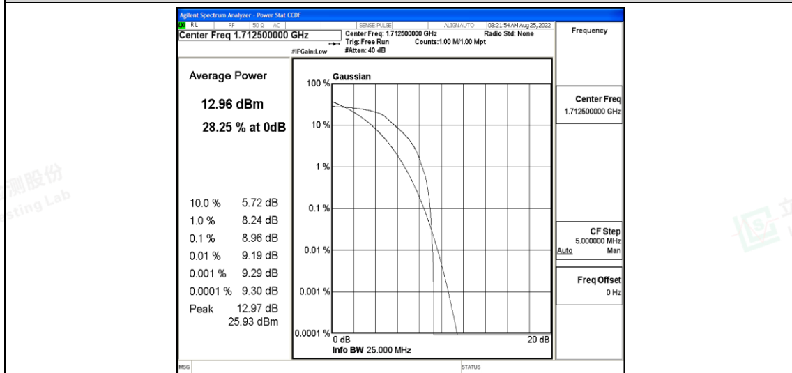
Band4-5MHz-16QAM-19975-6-0-Low-8.96-&lt;=13-PASS
