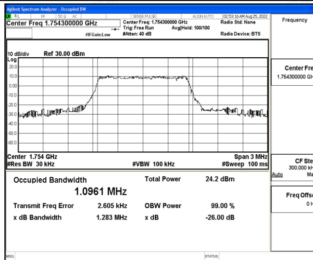
Band4-1.4MHz-16QAM-20393-6-0-High-1.0961-1.283-PASS
