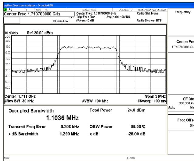
Band4-1.4MHz-QPSK-19957-6-0-Low-1.1036-1.290-PASS
