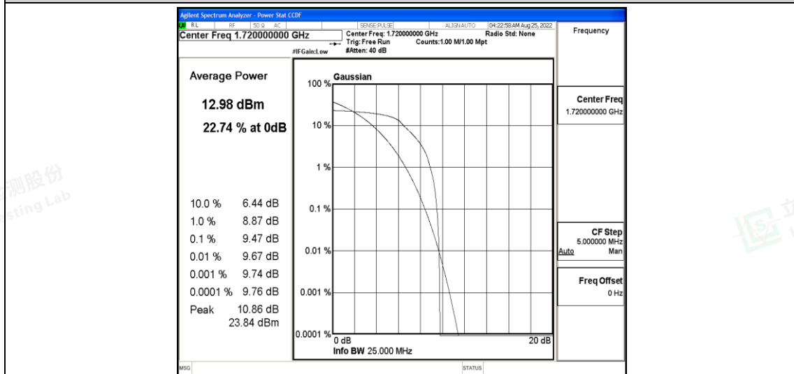
Band4-20MHz-QPSK-20050-6-0-Low-9.47-&lt;=13-PASS
