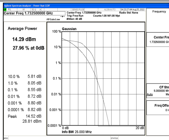
Band4-20MHz-16QAM-20175-6-0-Low-8.55-&lt;=13-PASS
