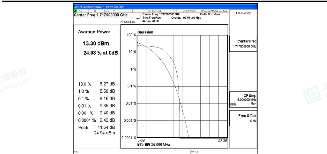
Band4-15MHz-QPSK-20025-6-0-Low-9.16-&lt;=13-PASS
