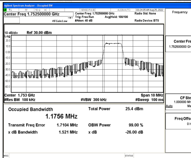
Band4-5MHz-QPSK-20375-6-0-High-1.1756-1.521-PASS
