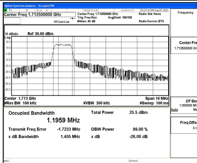
Band4-5MHz-16QAM-19975-6-0-Low-1.1959-1.405-PASS
