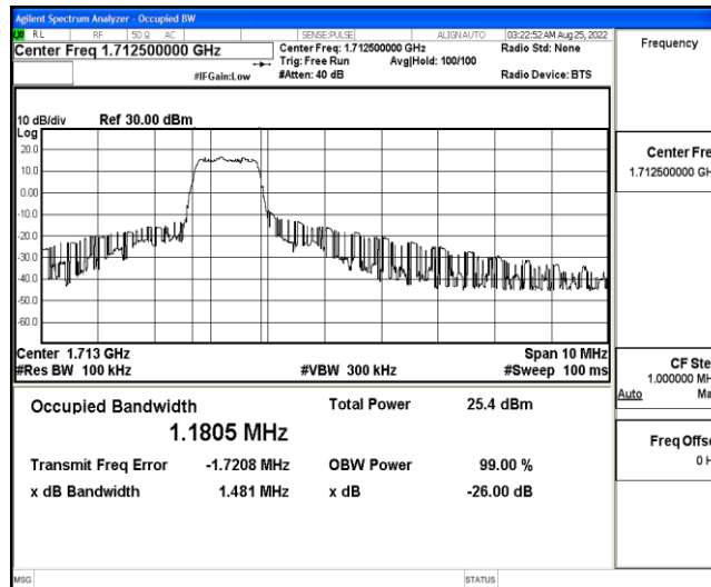
Band4-5MHz-QPSK-19975-6-0-Low-1.1805-1.481-PASS
