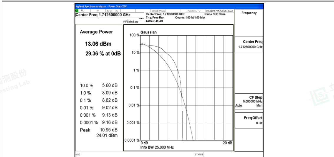
Band4-5MHz-QPSK-19975-6-0-Low-8.82-&lt;=13-PASS
