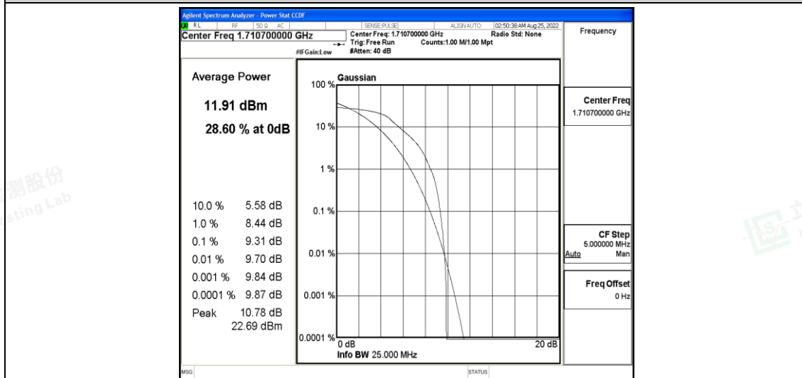
Band4-1.4MHz-16QAM-19957-6-0-Low-9.31-&lt;=13-PASS
