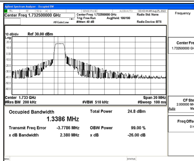
Band4-10MHz-QPSK-20175-6-0-Low-1.3386-2.380-PASS
