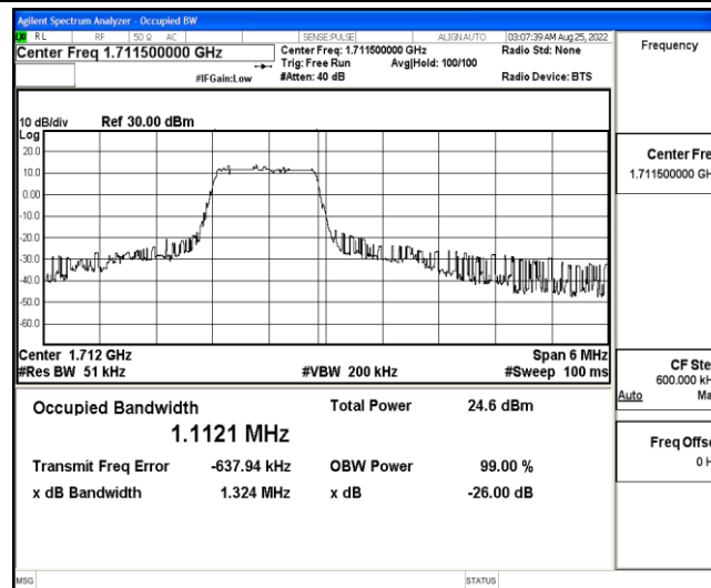
Band4-3MHz-16QAM-19965-6-0-Low-1.1121-1.324-PASS
