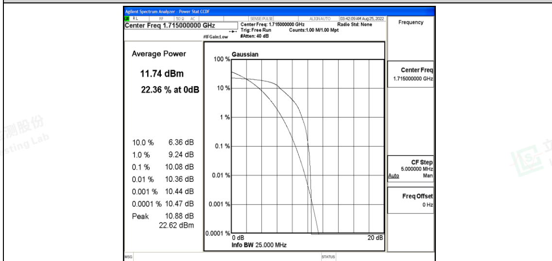
Band4-10MHz-16QAM-20000-6-0-Low-10.08-&lt;=13-PASS
