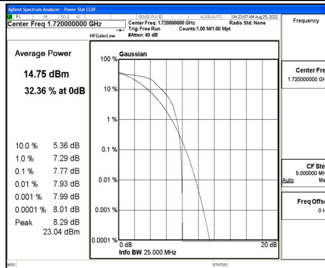
Band4-20MHz-16QAM-20050-6-0-Low-7.77-&lt;=13-PASS
