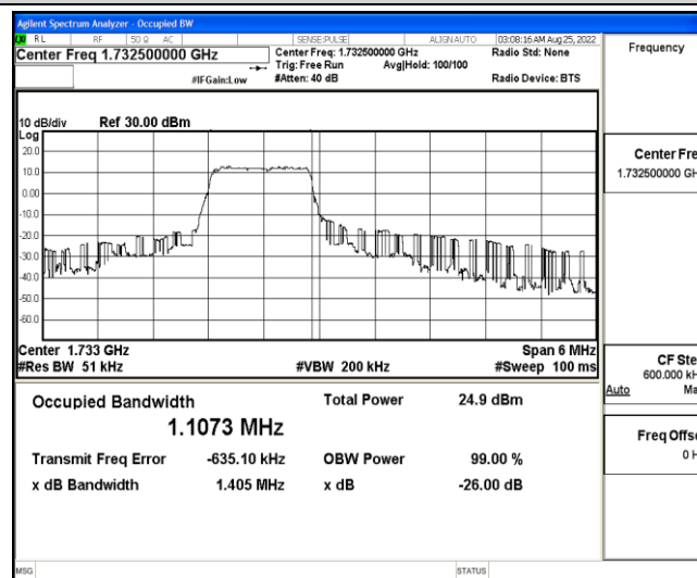
Band4-3MHz-16QAM-20175-6-0-Low-1.1073-1.405-PASS
