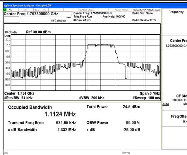
Band4-3MHz-16QAM-20385-6-0-High-1.1124-1.332-PASS
