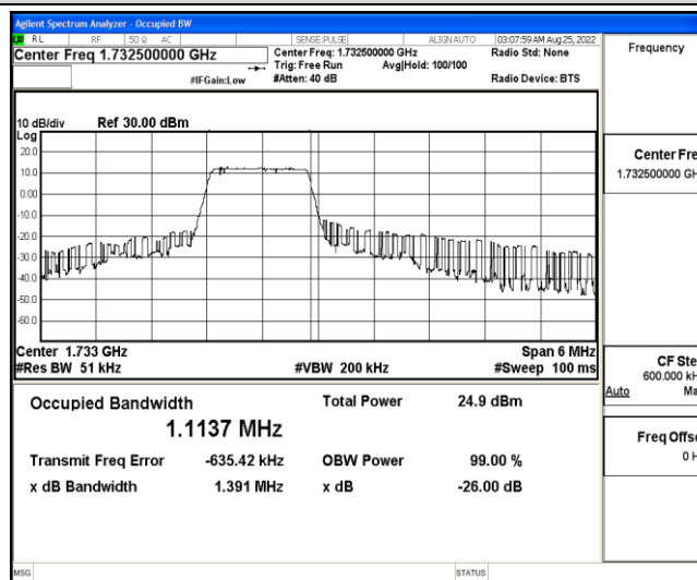
Band4-3MHz-QPSK-20175-6-0-Low-1.1137-1.391-PASS
