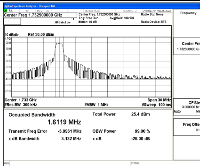
Band4-15MHz-QPSK-20175-6-0-Low-1.6119-3.132-PASS
