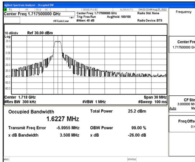
Band4-15MHz-QPSK-20025-6-0-Low-1.6227-3.508-PASS
