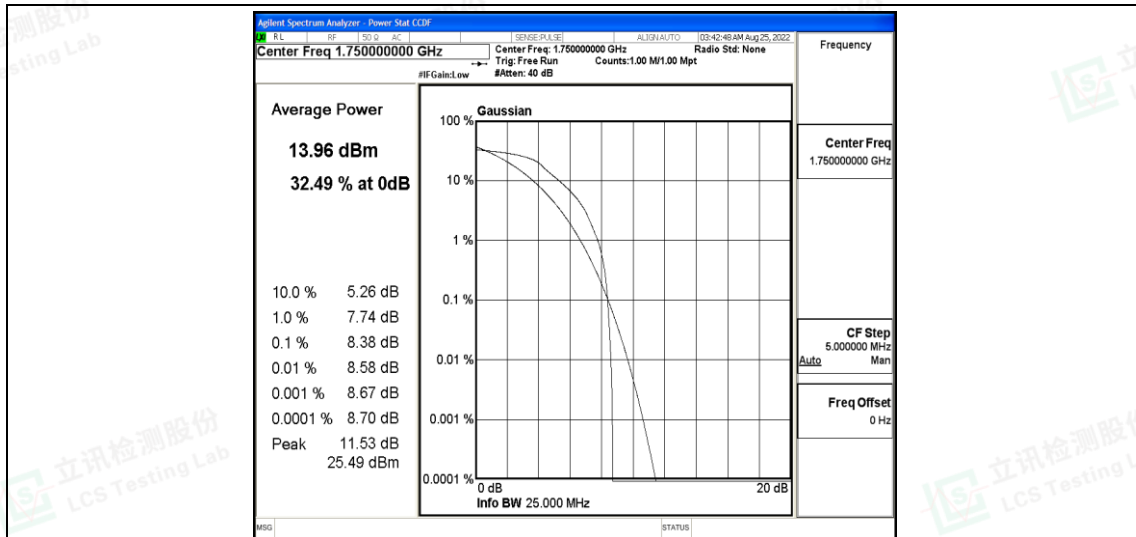
Band4-10MHz-16QAM-20350-6-0-High-8.38-&lt;=13-PASS
