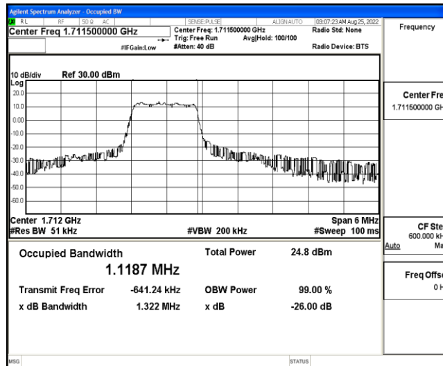
Band4-3MHz-QPSK-19965-6-0-Low-1.1187-1.322-PASS
