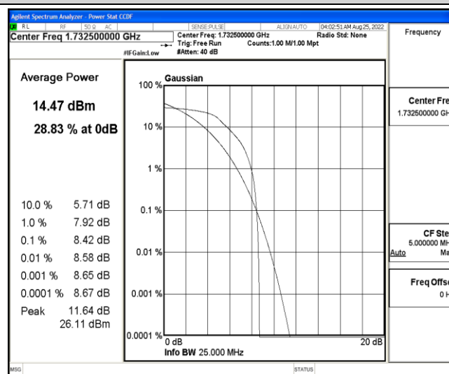
Band4-15MHz-16QAM-20175-6-0-Low-8.42-&lt;=13-PASS
