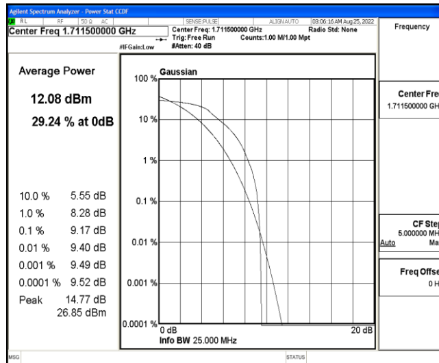
Band4-3MHz-QPSK-19965-6-0-Low-9.17-&lt;=13-PASS
