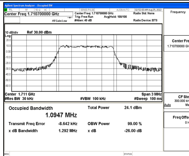
Band4-1.4MHz-16QAM-19957-6-0-Low-1.0947-1.292-PASS
