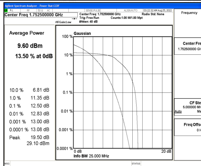
Band4-5MHz-16QAM-20375-6-0-High-12.50-13-PASS
