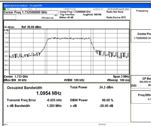
Band4-1.4MHz-16QAM-20175-6-0-Low-1.0954-1.283-PASS
