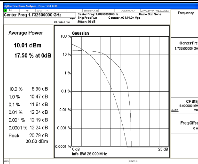
Band4-3MHz-QPSK-20175-6-0-Low-11.61-&lt;=13-PASS
