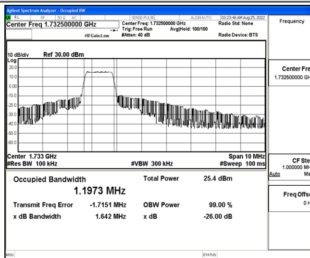
Band4-5MHz-16QAM-20175-6-0-Low-1.1973-1.642-PASS
