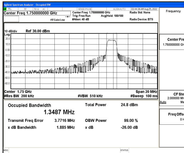
Band4-10MHz-16QAM-20350-6-0-High-1.3487-1.885-PASS
