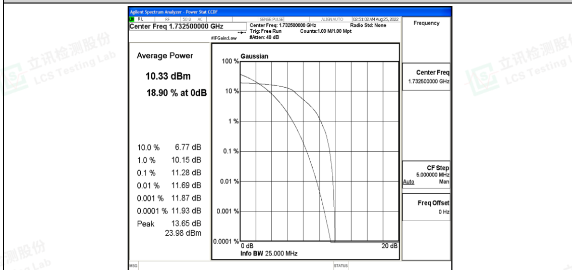
Band4-1.4MHz-16QAM-20175-6-0-Low-11.28-&lt;=13-PASS
