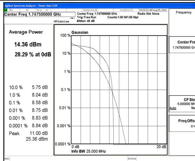
Band4-15MHz-QPSK-20325-6-0-High-8.58-&lt;=13-PASS
