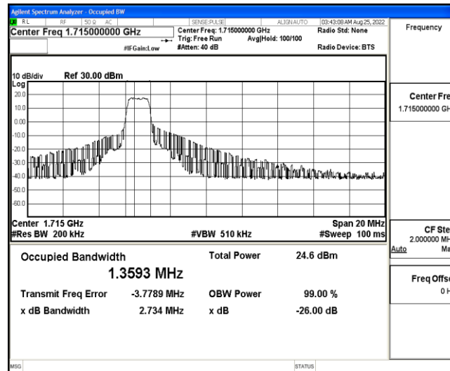
Band4-10MHz-QPSK-20000-6-0-Low-1.3593-2.734-PASS
