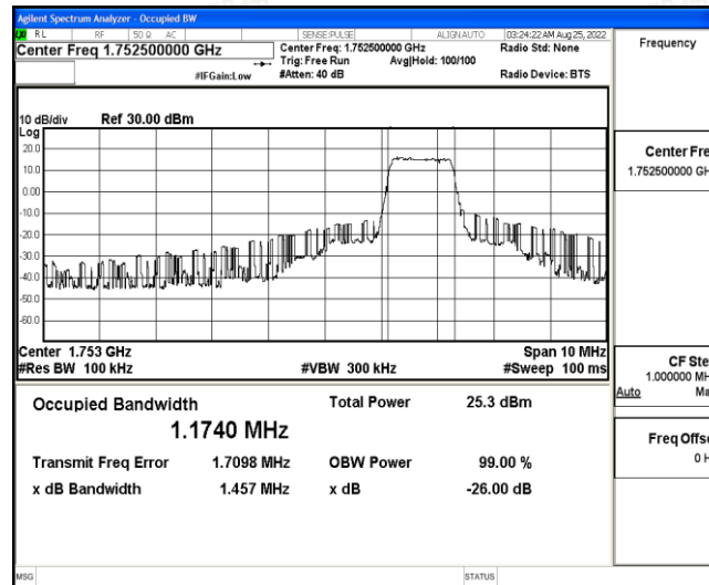
Band4-5MHz-16QAM-20375-6-0-High-1.1740-1.457-PASS
