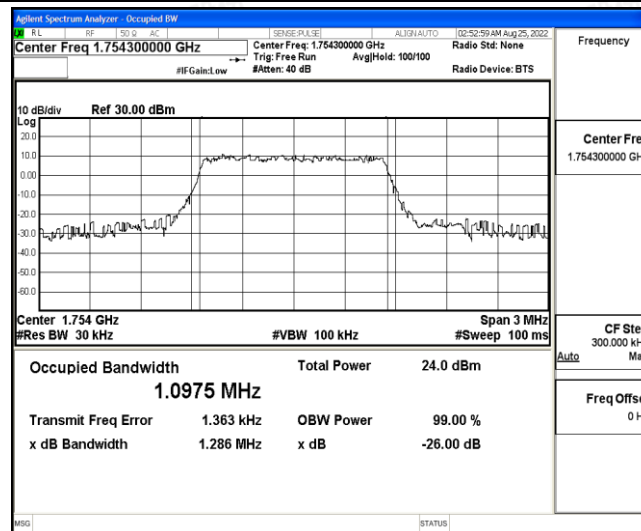
Band4-1.4MHz-QPSK-20393-6-0-High-1.0975-1.286-PASS
