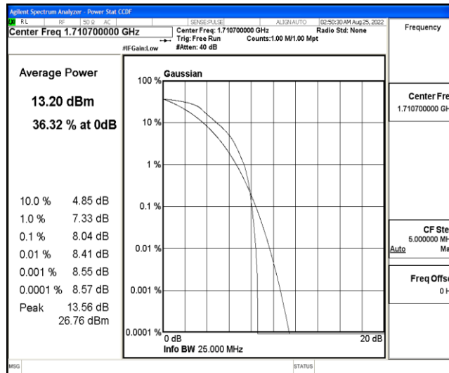
Band4-1.4MHz-QPSK-19957-6-0-Low-8.04-&lt;=13-PASS
