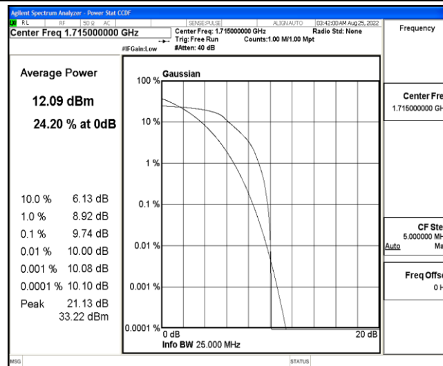
Band4-10MHz-QPSK-20000-6-0-Low-9.74-13-PASS
