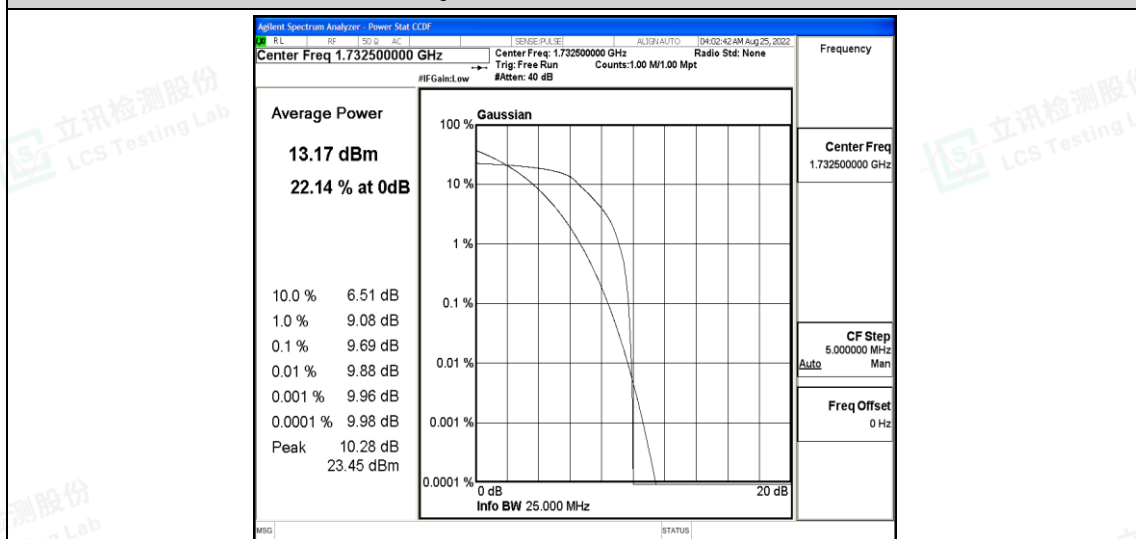
Band4-15MHz-QPSK-20175-6-0-Low-9.69-&lt;=13-PASS
