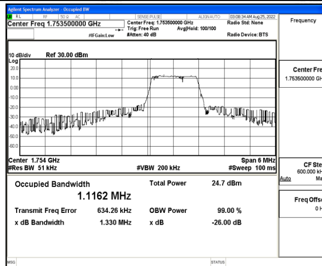
Band4-3MHz-QPSK-20385-6-0-High-1.1162-1.330-PASS
