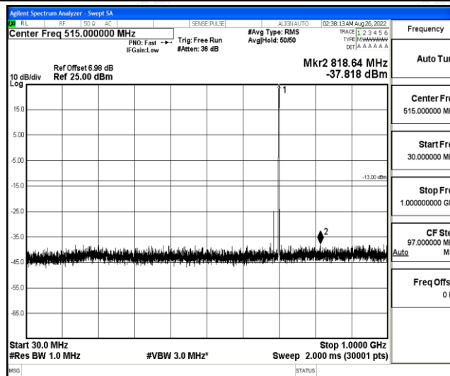
Band12-1.4MHz-QPSK-23095-1-0-Low-30-1000--37.82-PASS
