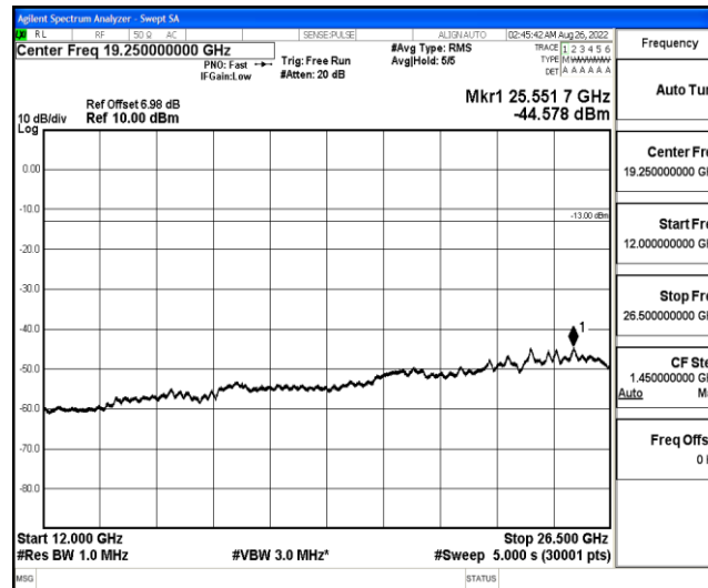
Band12-1.4MHz-16QAM-23173-1-0-High-12000-26500--44.58-PASS
