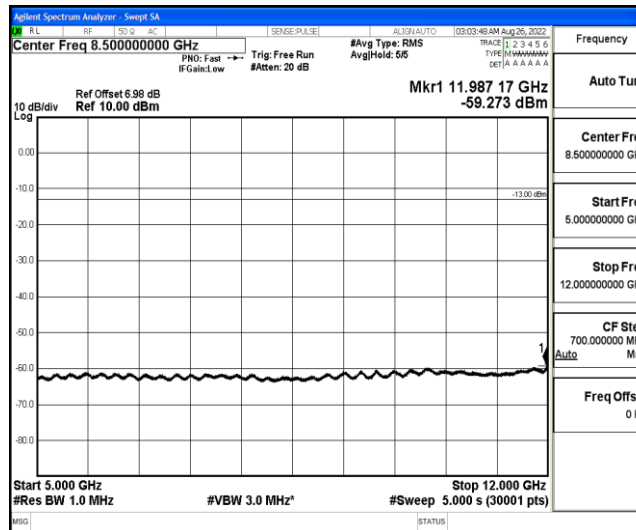
Band12-3MHz-16QAM-23025-1-0-Low-5000-12000--59.27-PASS
