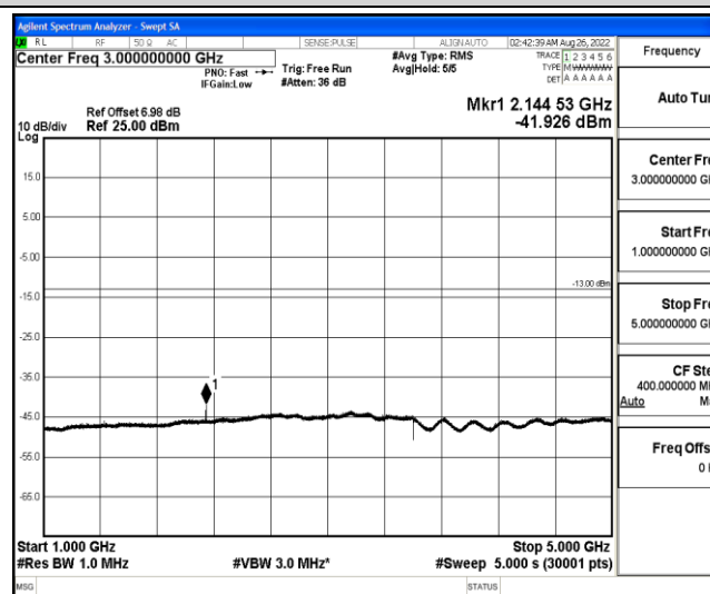
Band12-1.4MHz-QPSK-23173-1-0-High-1000-5000--41.93-PASS
