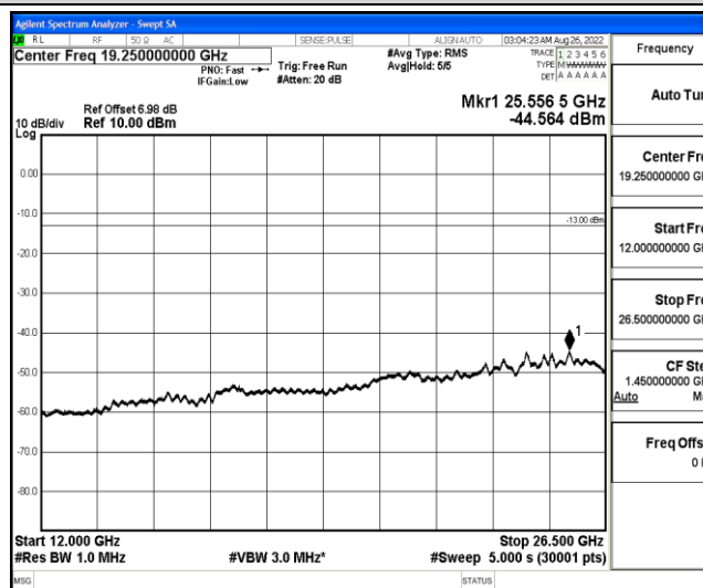
Band12-3MHz-16QAM-23025-1-0-Low-12000-26500--44.56-PASS
