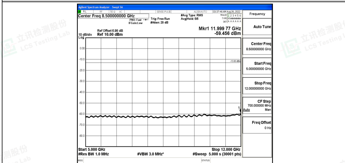
Band12-5MHz-16QAM-23095-1-0-Low-5000-12000--59.46-PASS
