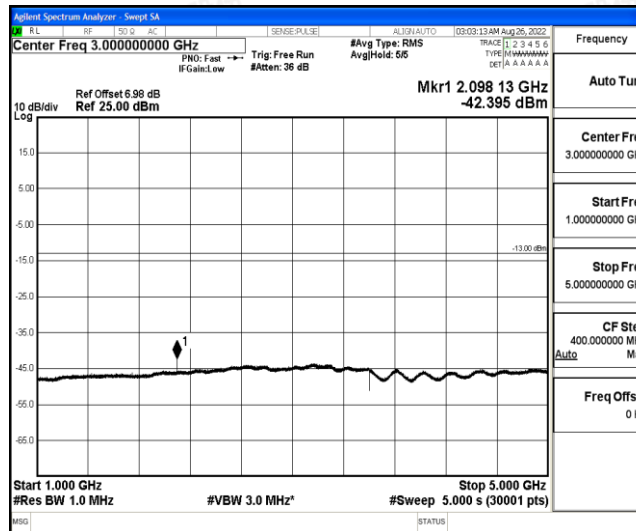
Band12-3MHz-16QAM-23025-1-0-Low-1000-5000--42.4-PASS
