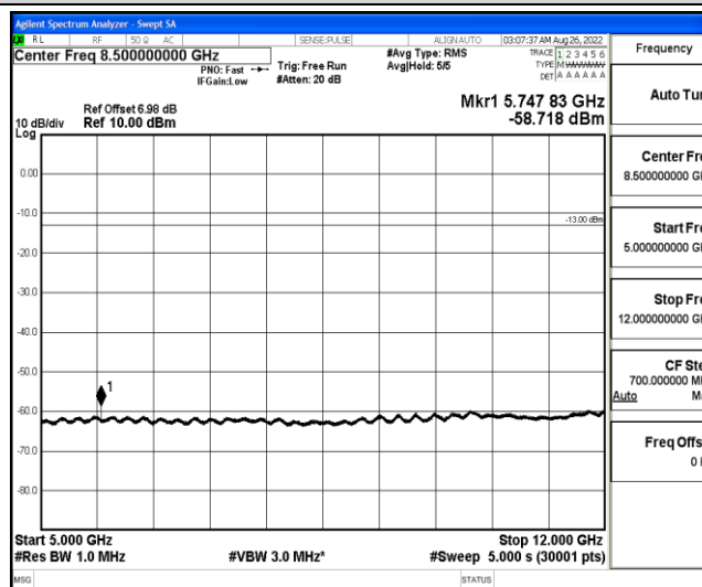
Band12-3MHz-16QAM-23095-1-0-Low-5000-12000--58.72-PASS
