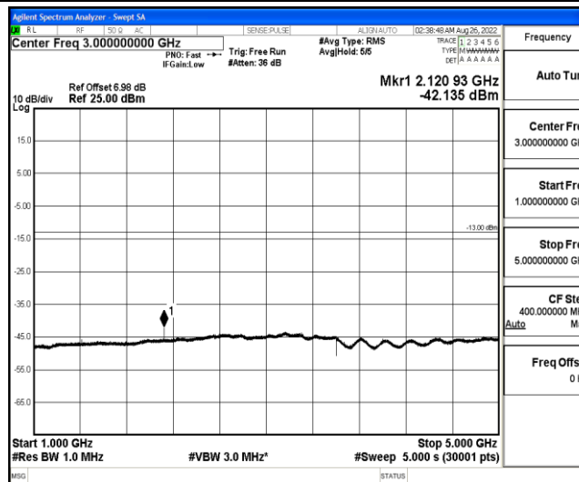
Band12-1.4MHz-QPSK-23095-1-0-Low-1000-5000--42.14-PASS
