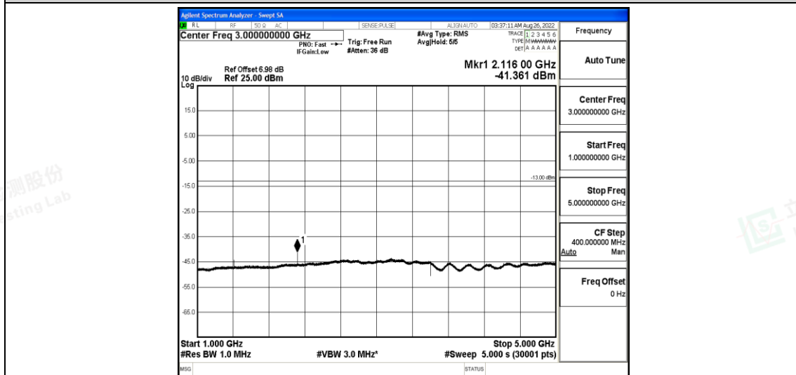
Band12-5MHz-16QAM-23095-1-0-Low-1000-5000--41.36-PASS
