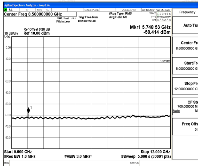
Band12-5MHz-16QAM-23155-1-0-High-5000-12000--58.41-PASS
