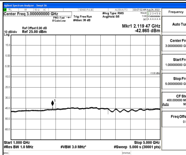
Band12-3MHz-16QAM-23095-1-0-Low-1000-5000--42.87-PASS
