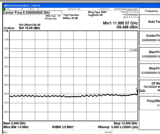
Band12-5MHz-QPSK-23095-1-0-Low-5000-12000--59.47-PASS
