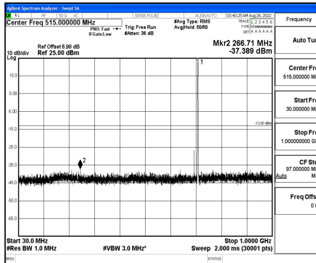
Band12-5MHz-16QAM-23155-1-0-High-30-1000--37.39-PASS
