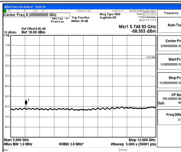
Band12-1.4MHz-QPSK-23095-1-0-Low-5000-12000--58.55-PASS
