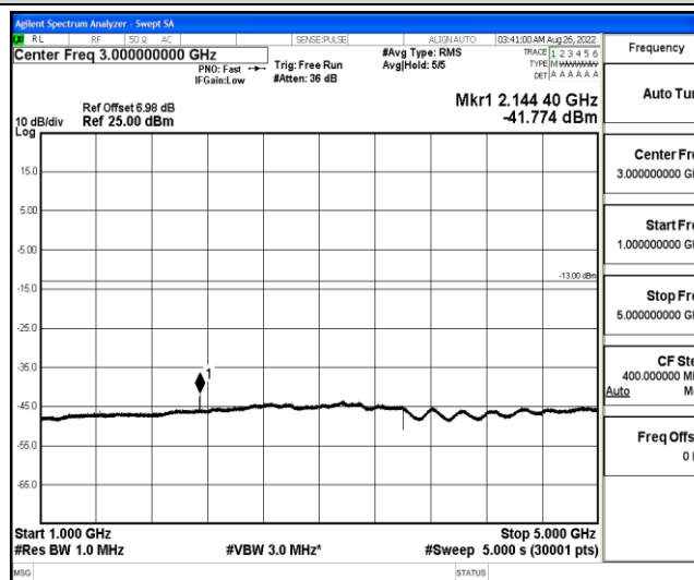
Band12-5MHz-16QAM-23155-1-0-High-1000-5000--41.77-PASS
