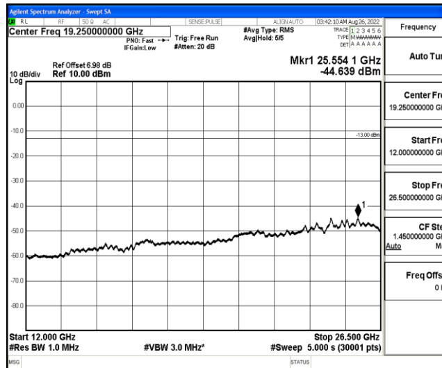
Band12-5MHz-16QAM-23155-1-0-High-12000-26500--44.64-PASS
