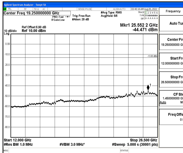
Band12-5MHz-QPSK-23155-1-0-High-12000-26500--44.47-PASS
