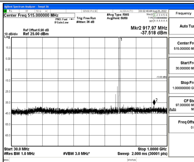
Band12-5MHz-16QAM-23035-1-0-Low-30-1000--37.52-PASS
