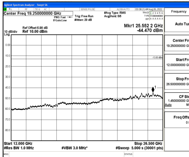
Band12-5MHz-16QAM-23095-1-0-Low-12000-26500--44.47-PASS
