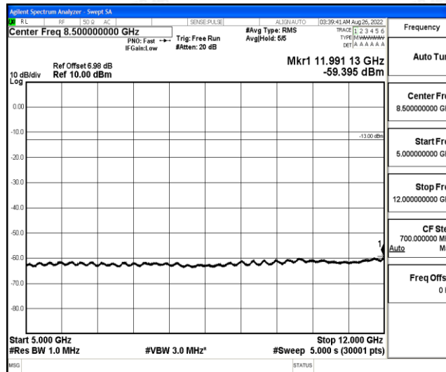
Band12-5MHz-QPSK-23155-1-0-High-5000-12000--59.4-PASS
