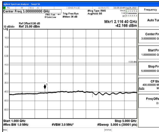
Band12-5MHz-QPSK-23095-1-0-Low-1000-5000--42.17-PASS
