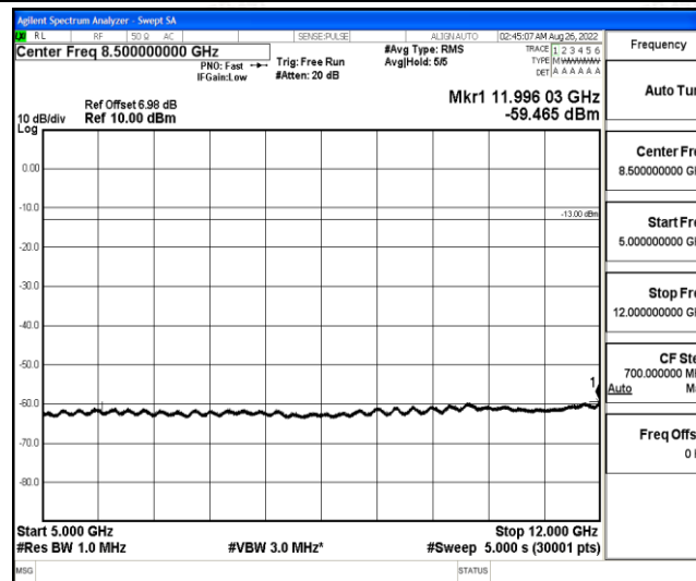
Band12-1.4MHz-16QAM-23173-1-0-High-5000-12000--59.47-PASS
