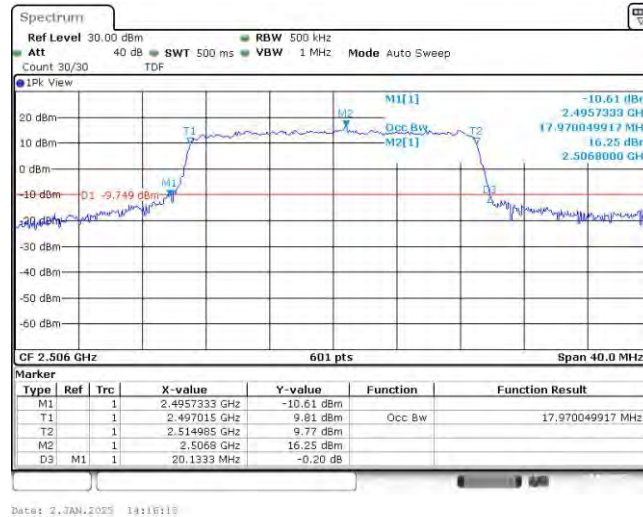
Band41-20MHz-16QAM-40690-100RB#0
