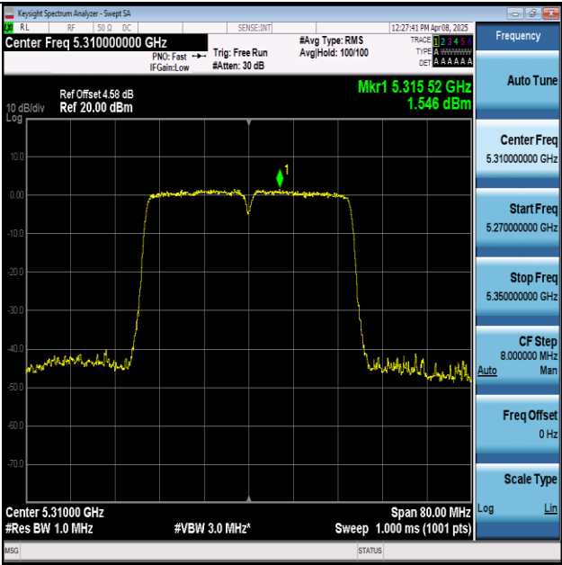
11AC40MIMO-Ant1-5310-PASS
