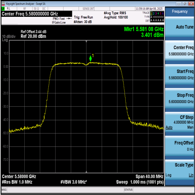
11N20MIMO-Ant1-5580-PASS
