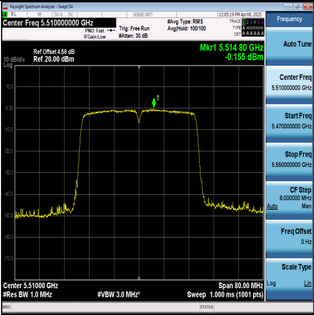
11N40MIMO-Ant1-5510-PASS
