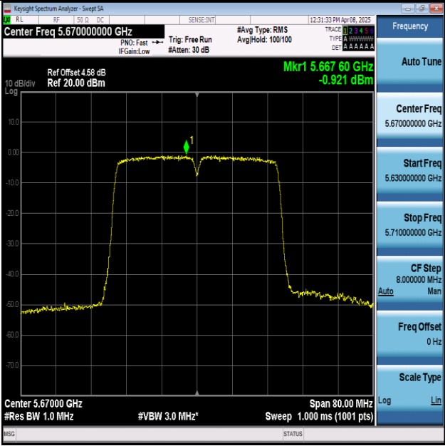
11AC40MIMO-Ant1-5670-PASS
