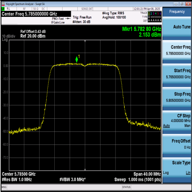
11N20MIMO-Ant1-5785-PASS
