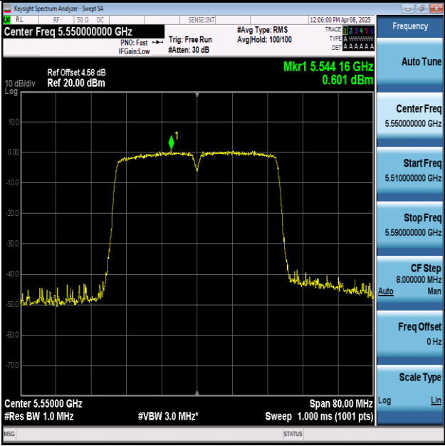
11N40MIMO-Ant1-5550-PASS
