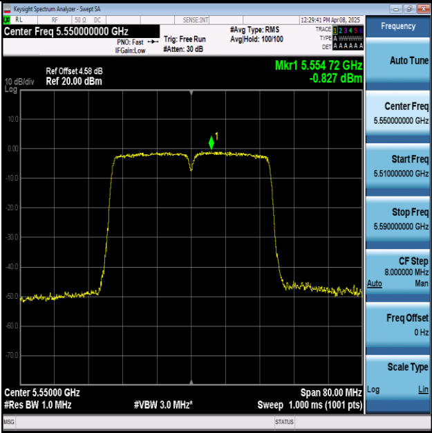
11AC40MIMO-Ant1-5550-PASS
