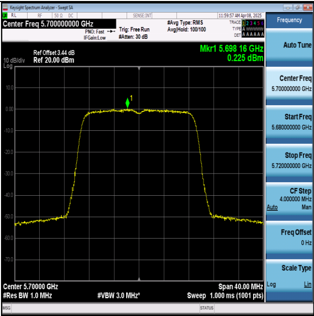
11N20MIMO-Ant1-5700-PASS
