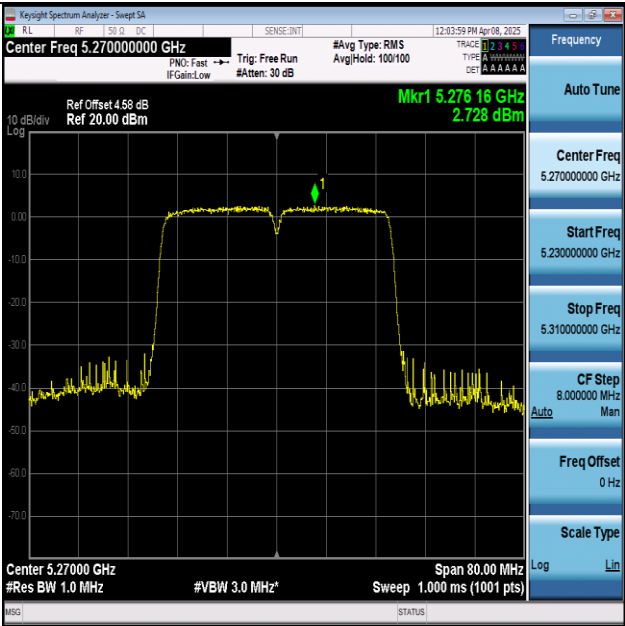
11N40MIMO-Ant1-5270-PASS
