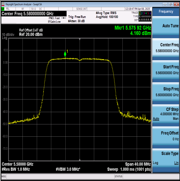
11AC20MIMO-Ant1-5580-PASS
