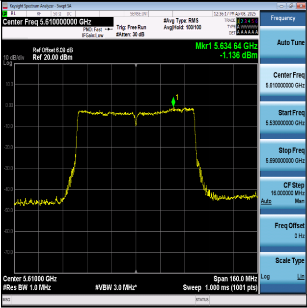
11AC80MIMO-Ant1-5610-PASS
