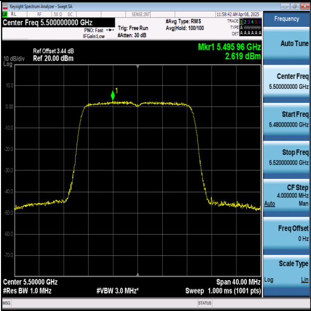
11N20MIMO-Ant1-5500-PASS
