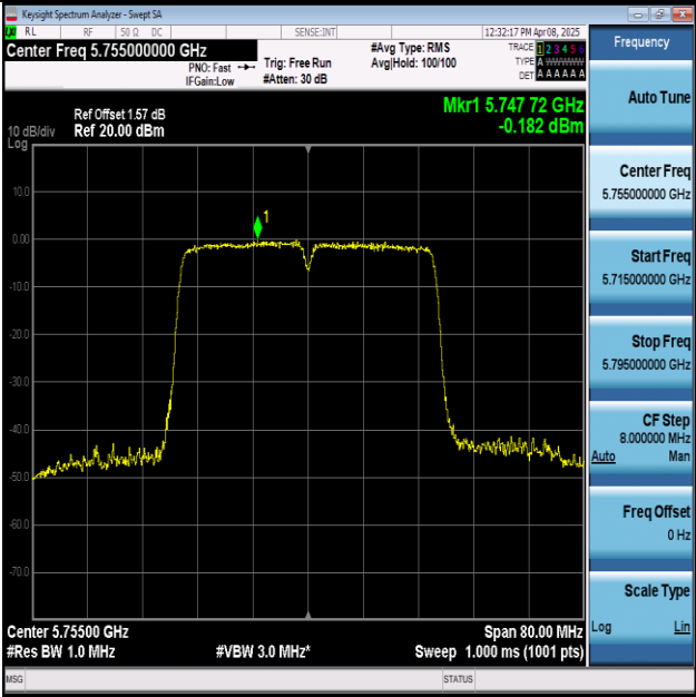
11AC40MIMO-Ant1-5755-PASS
