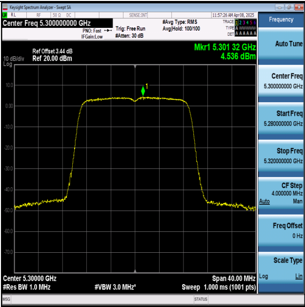
11N20MIMO-Ant1-5300-PASS
