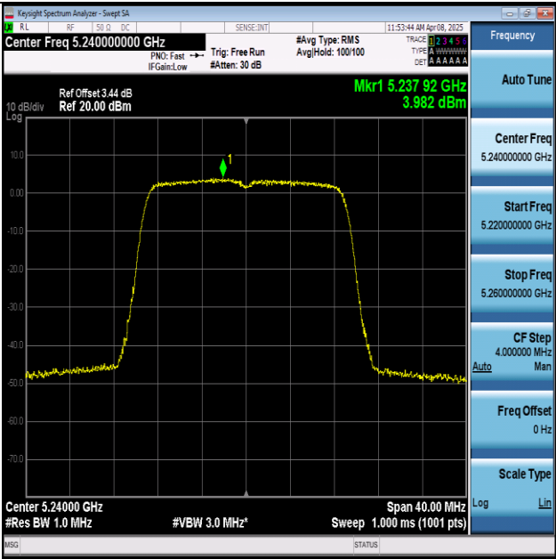
11N20MIMO-Ant1-5240-PASS
