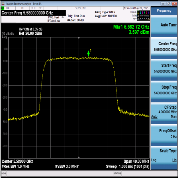
11AX20MIMO-Ant1-5580-PASS
