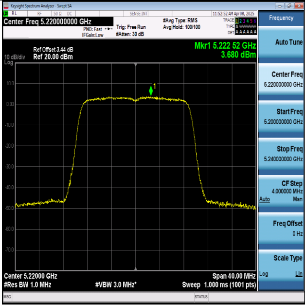
11N20MIMO-Ant1-5220-PASS
