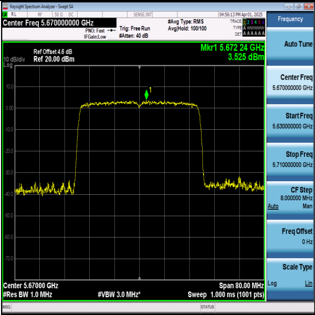
11AX40SISO-Ant1-5670-PASS
