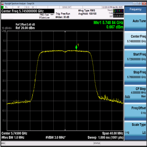
11AC20MIMO-Ant1-5745-PASS
