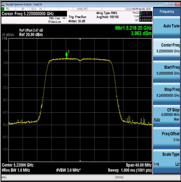
11AC20MIMO-Ant1-5220-PASS
