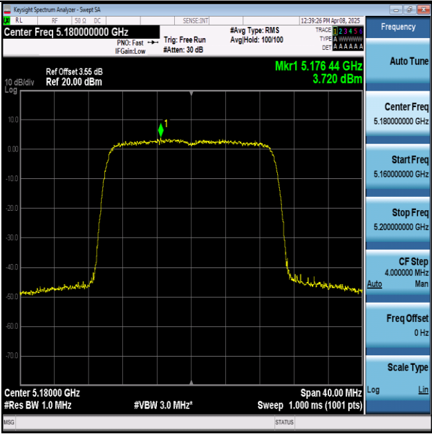
11AX20MIMO-Ant1-5180-PASS
