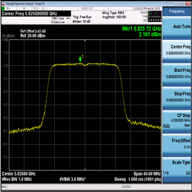
11N20MIMO-Ant1-5825-PASS
