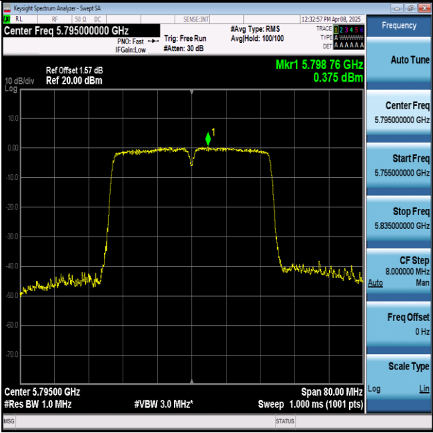
11AC40MIMO-Ant1-5795-PASS
