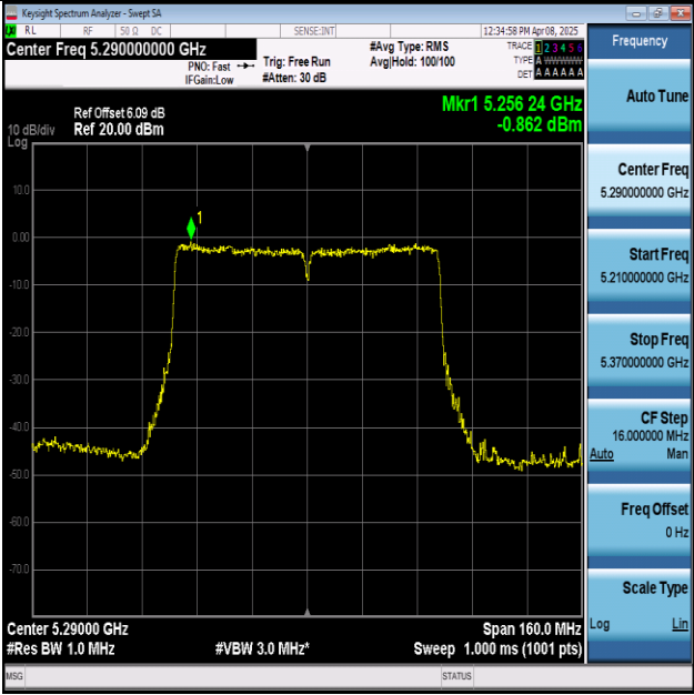
11AC80MIMO-Ant1-5290-PASS
