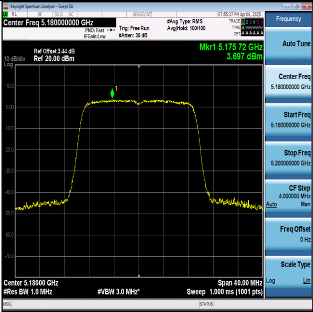
11N20MIMO-Ant1-5180-PASS
