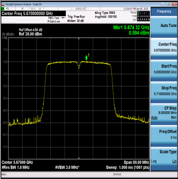
11N40MIMO-Ant1-5670-PASS
