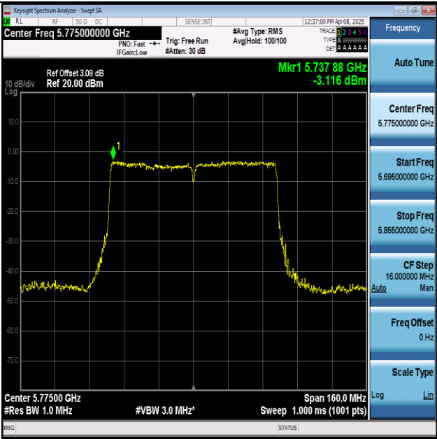
11AC80MIMO-Ant1-5775-PASS
