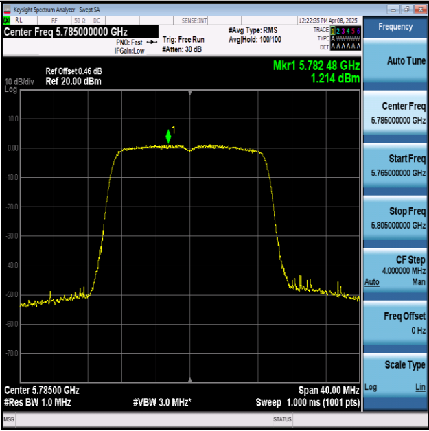
11AC20MIMO-Ant1-5785-PASS
