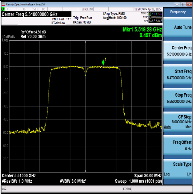
11AC40MIMO-Ant1-5510-PASS
