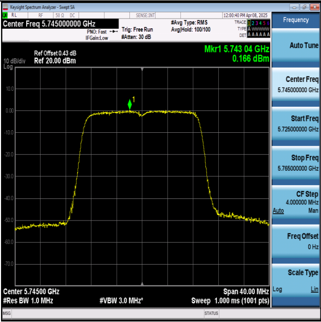
11N20MIMO-Ant1-5745-PASS
