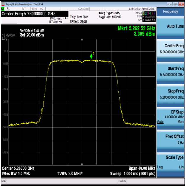
11N20MIMO-Ant1-5260-PASS
