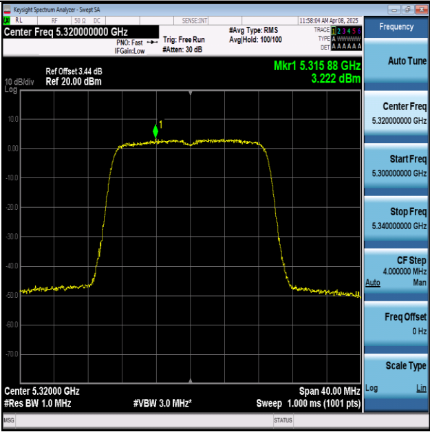
11N20MIMO-Ant1-5320-PASS
