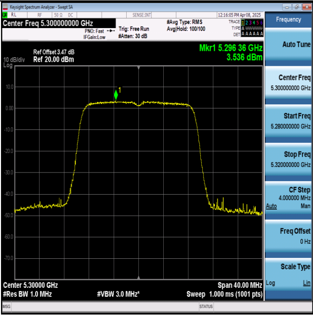
11AC20MIMO-Ant1-5300-PASS
