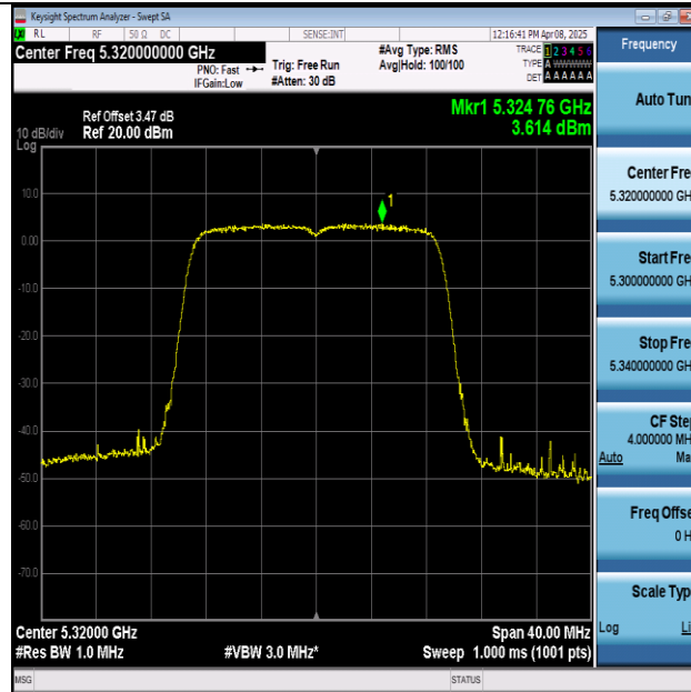
11AC20MIMO-Ant1-5320-PASS
