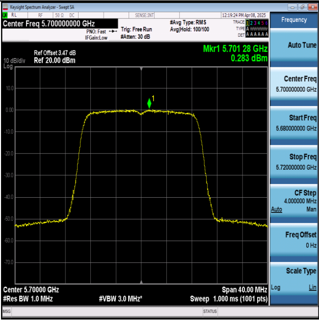
11AC20MIMO-Ant1-5700-PASS
