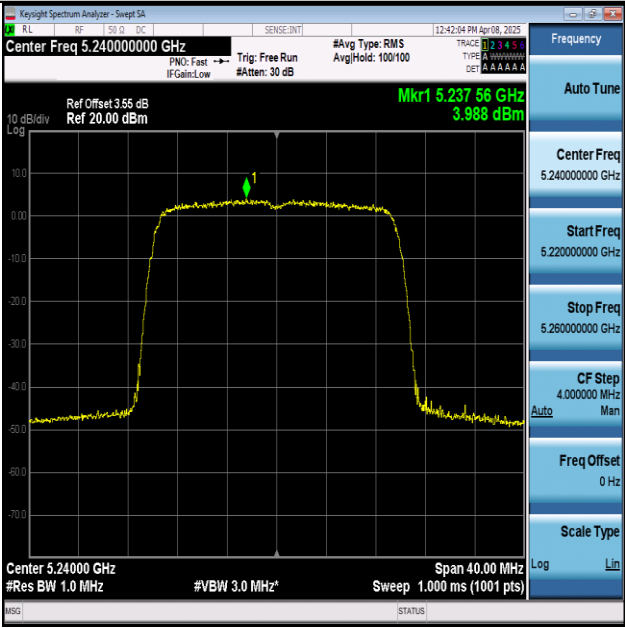
11AX20MIMO-Ant1-5240-PASS
