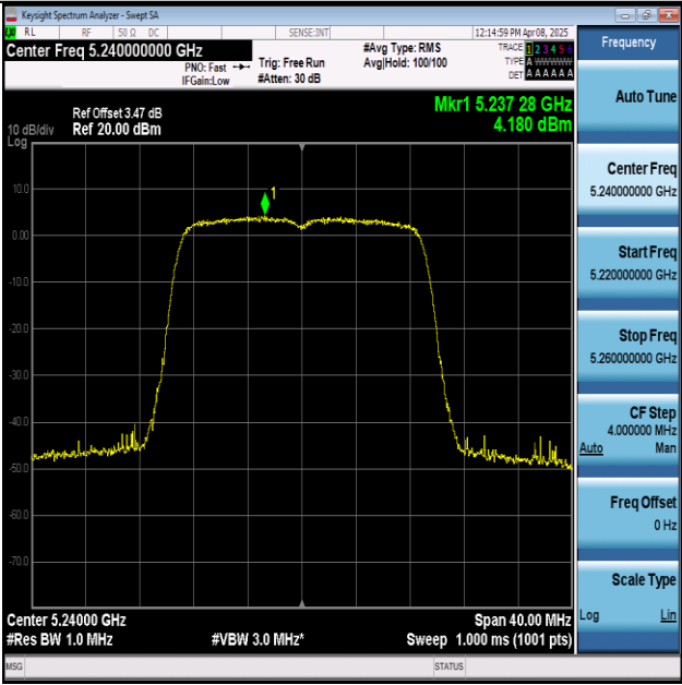
11AC20MIMO-Ant1-5240-PASS
