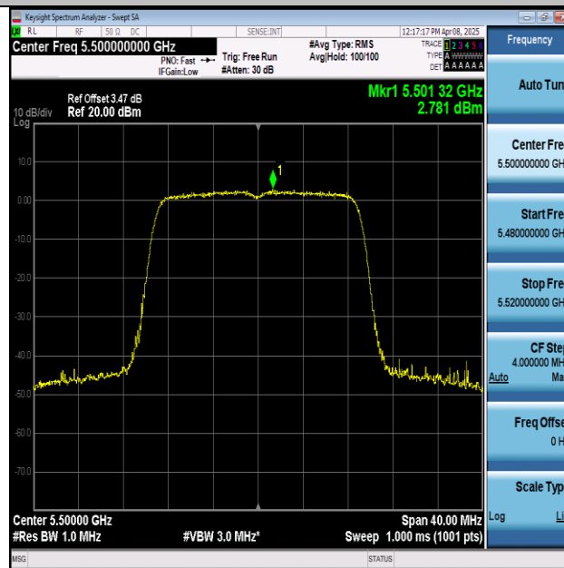
11AC20MIMO-Ant1-5500-PASS
