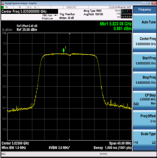
11AC20MIMO-Ant1-5825-PASS
