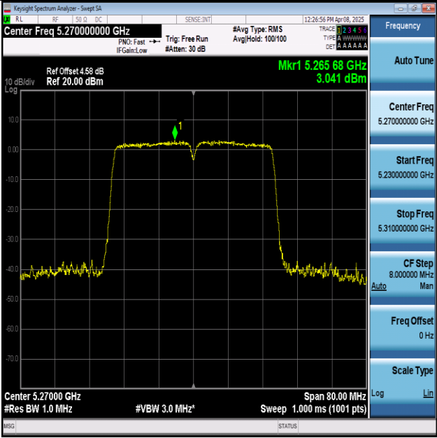
11AC40MIMO-Ant1-5270-PASS
