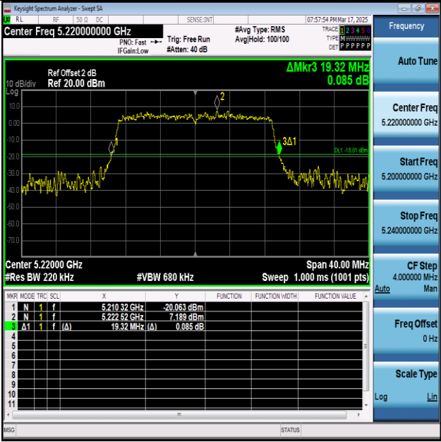
11N20SISO-Ant1-5220
