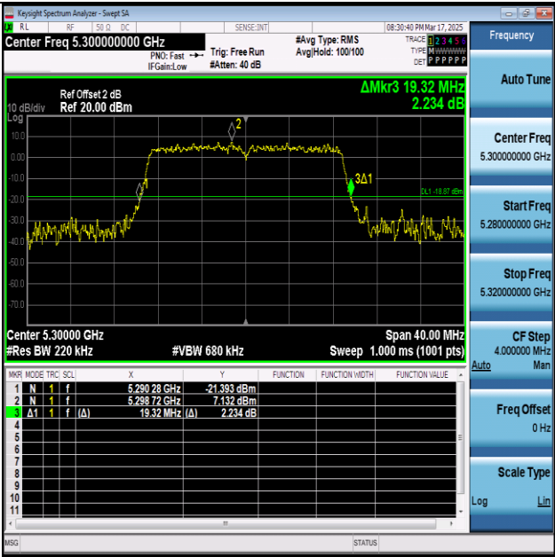
11N20SISO-Ant1-5300
