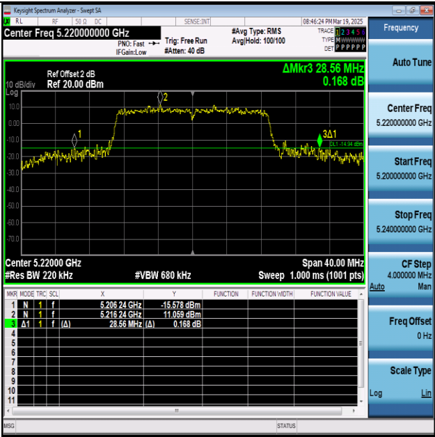
11AC20SISO-Ant1-5220
