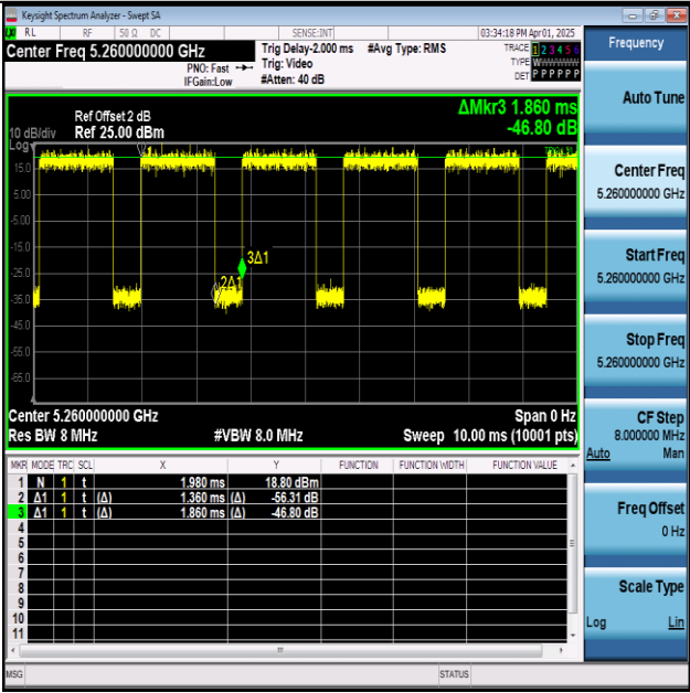
NTVN-11A-Ant1-5260
