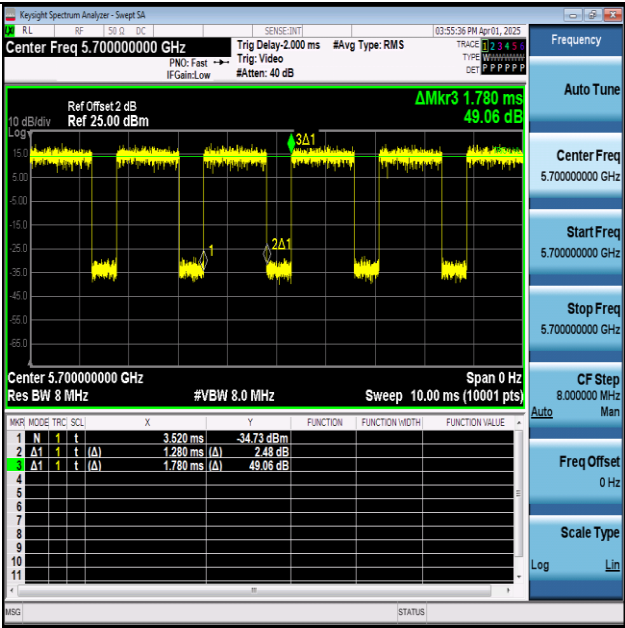
NTVN-11N20SISO-Ant1-5700
