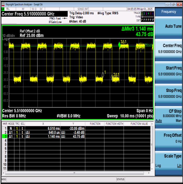
NTVN-11N40SISO-Ant1-5510
