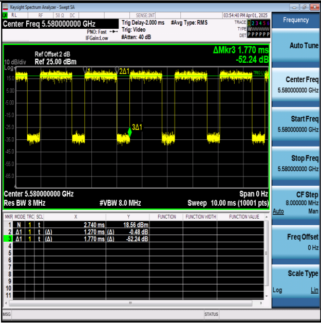
NTVN-11N20SISO-Ant1-5580
