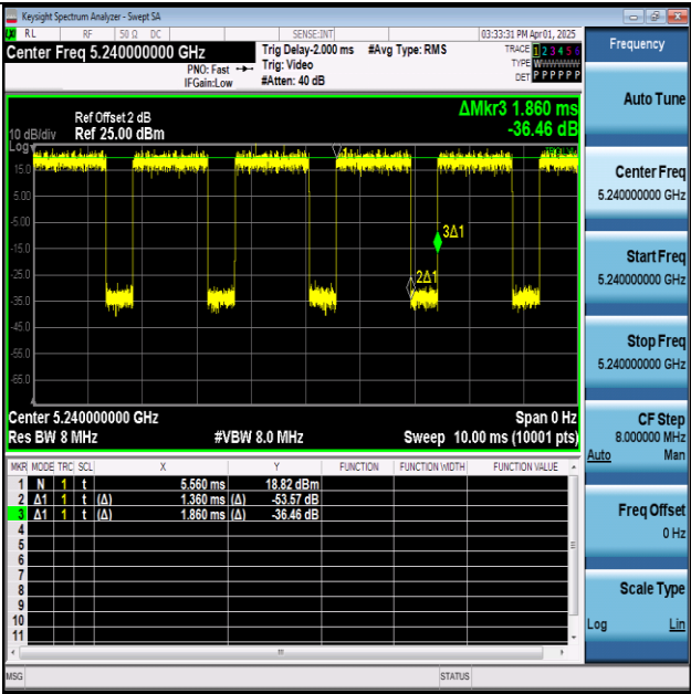
NTVN-11A-Ant1-5240
