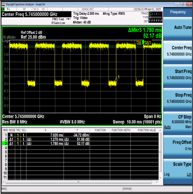
NTVN-11N20SISO-Ant1-5745
