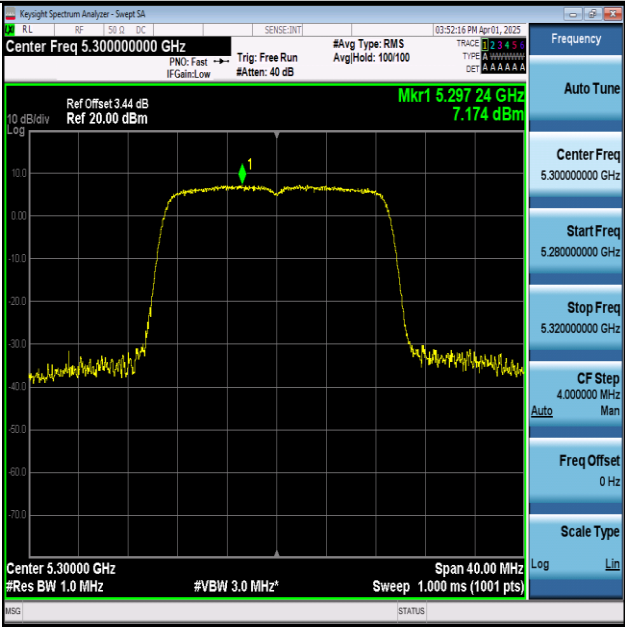
11N20SISO-Ant1-5300-PASS
