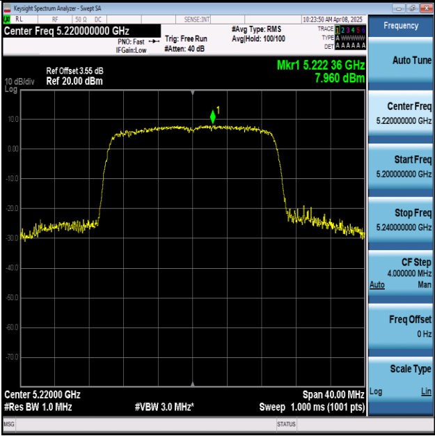
11AX20SISO-Ant1-5220-PASS
