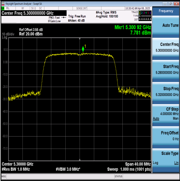
11AX20SISO-Ant1-5300-PASS
