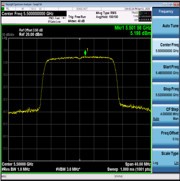
11AX20SISO-Ant1-5500-PASS
