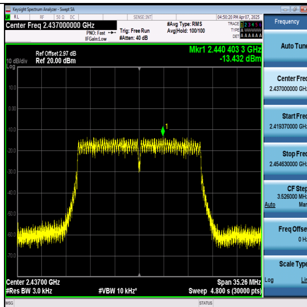
11N20MIMO-Ant1+2-2437-PASS
