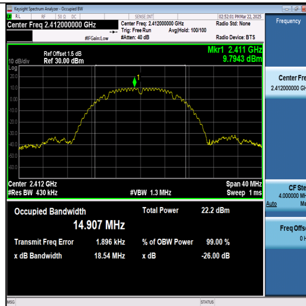
11B-Ant1-2412
