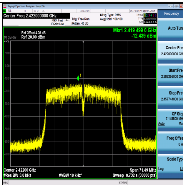
11N40MIMO-Ant1+2-2422-PASS
