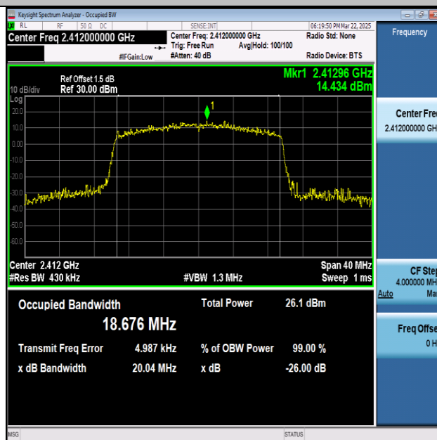
11AX20SISO-Ant1-2412
