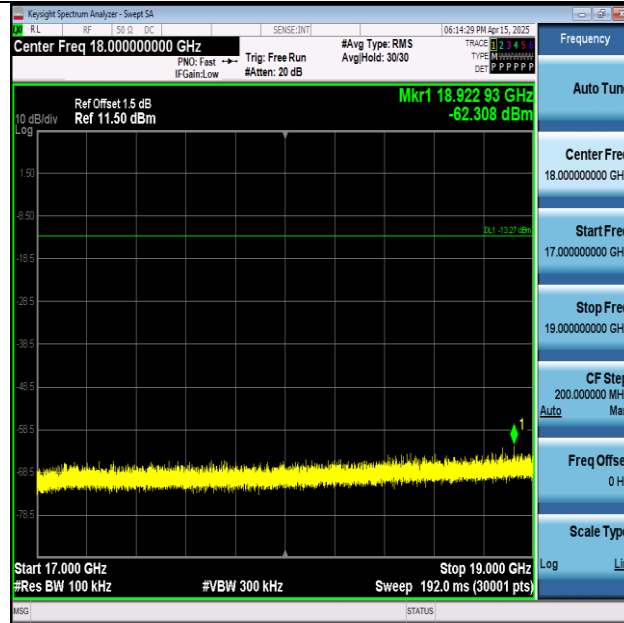
11N40SISO-Ant1-2422-17000~19000-PASS
