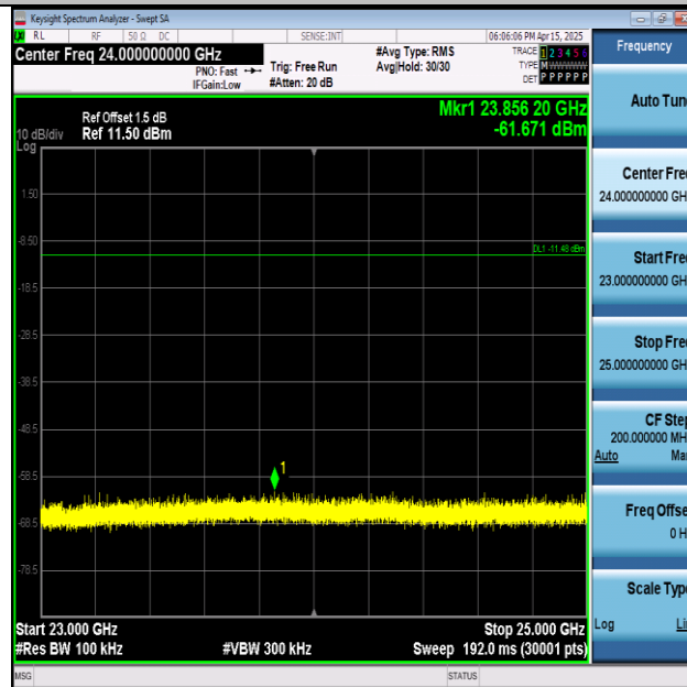
11N20SISO-Ant1-2437-23000~25000-PASS
