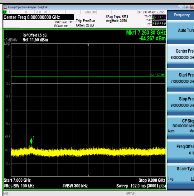
11N40SISO-Ant1-2422-7000~9000-PASS
