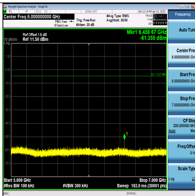
11N40SISO-Ant1-2422-5000~7000-PASS
