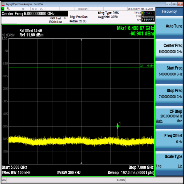
11N20SISO-Ant1-2437-5000~7000-PASS
