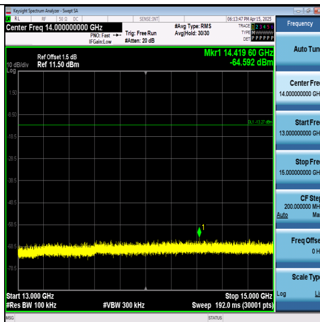
11N40SISO-Ant1-2422-13000~15000-PASS
