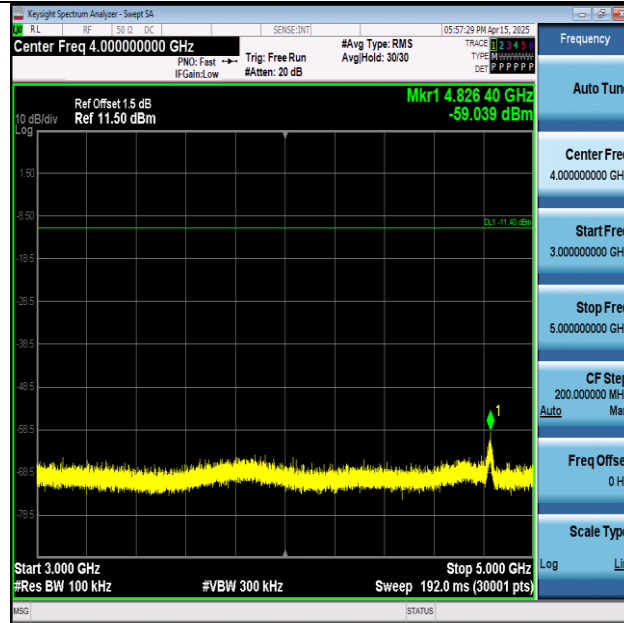
11N20SISO-Ant1-2412-3000~5000-PASS
