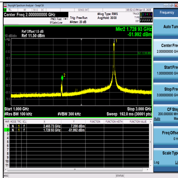
11G-Ant1-2462-1000~3000-PASS
