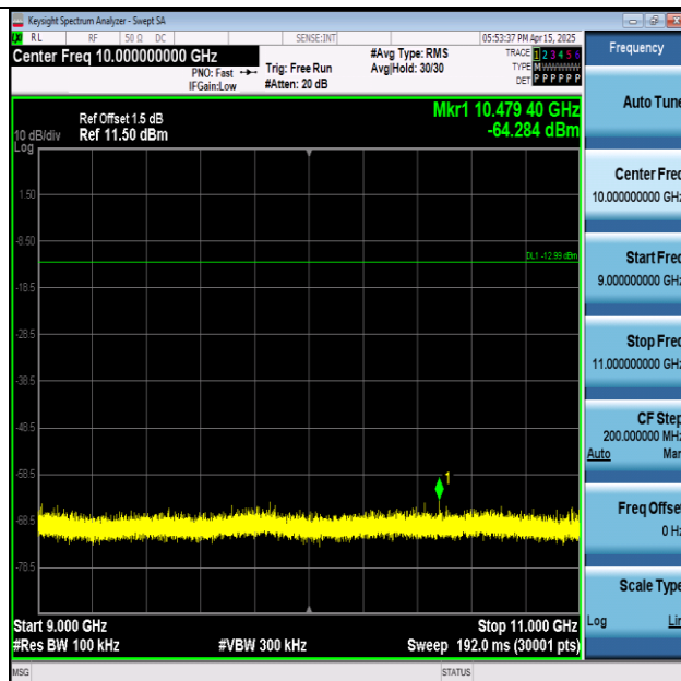
11G-Ant1-2462-9000~11000-PASS
