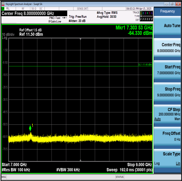
11N20SISO-Ant1-2437-7000~9000-PASS
