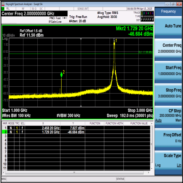
11N20SISO-Ant1-2462-1000~3000-PASS
