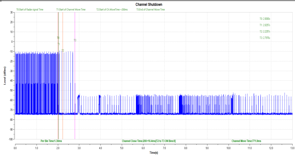
11N40SISO-5510-Type0
