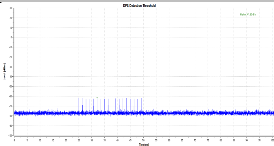
11N40SISO-5510-Type0
