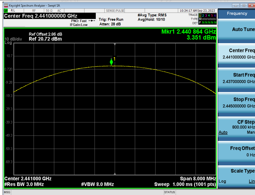
Peak_Output_Power_NVNT_ANT1_2-DH5_2441
