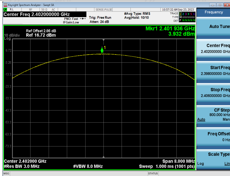
Peak_Output_Power_NVNT_ANT1_3-DH5_2402
