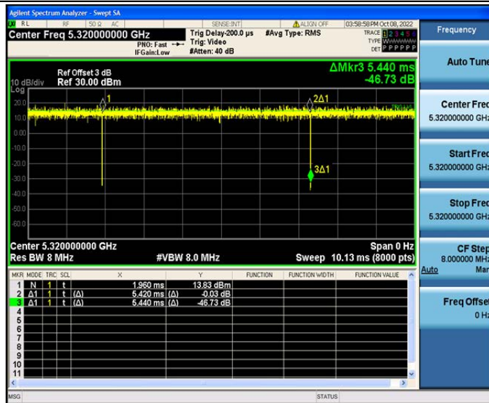
802.11ac(VHT20)_Ant2_5320
