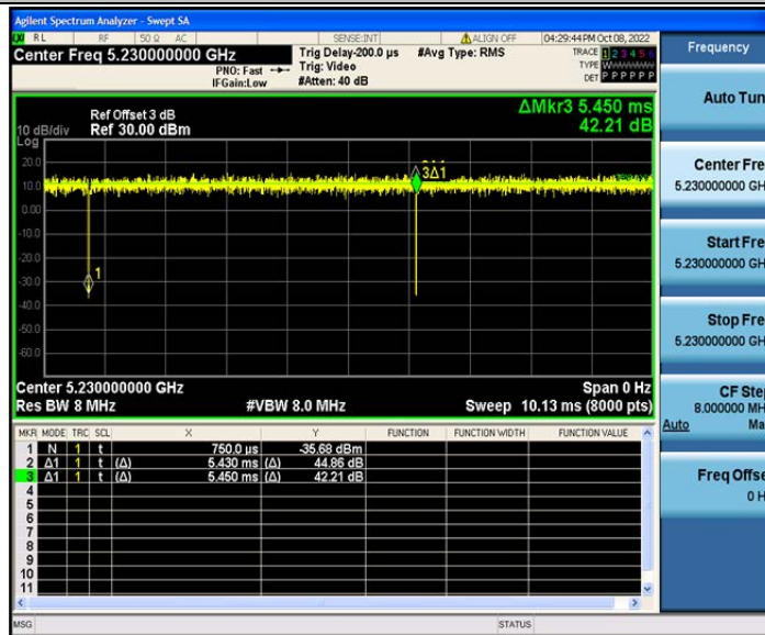
802.11ac(VHT40)_Ant2_5230
