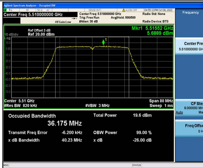
802.11ac(VHT40)_Ant2_5510
