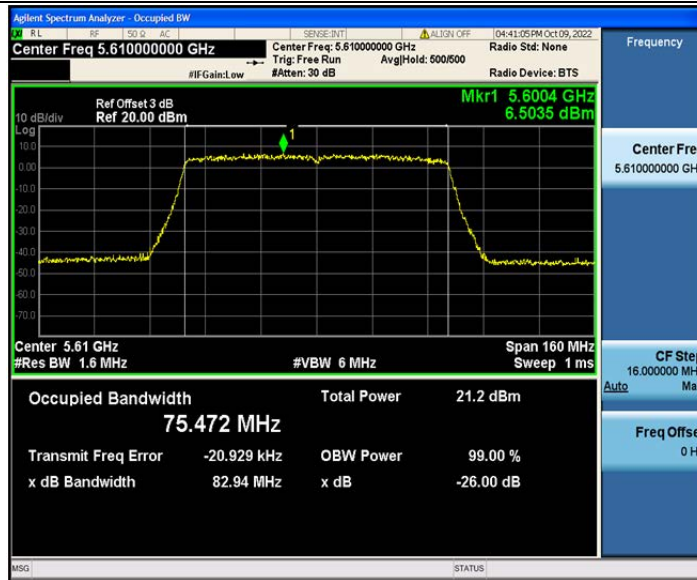
802.11ac(VHT80)_Ant2_5610
