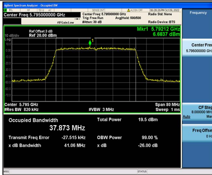
802.11ax(HE40)_Ant2_5795 484/65
