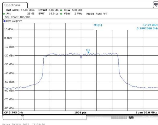
802.11ax(HE40)_Ant2_5795 26/8
