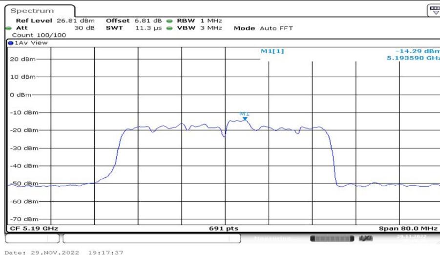
802.11ax(HE40)_Ant2_5190 52/40
