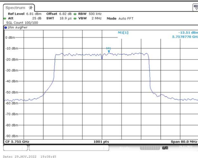
802.11ax(HE40)_Ant2_5755 52/40
