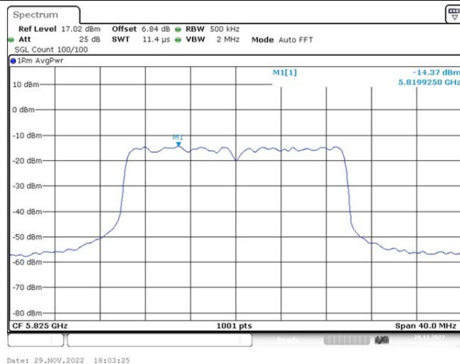
802.11ax(HE20)_Ant2_5825 106/53
