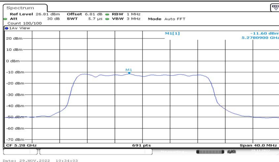
802.11ax(HE20)_Ant2_5280 106/53
