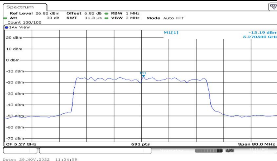
802.11ax(HE40)_Ant2_5270 26/8
