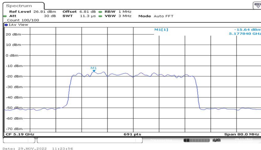
802.11ax(HE40)_Ant2_5190 106/54
