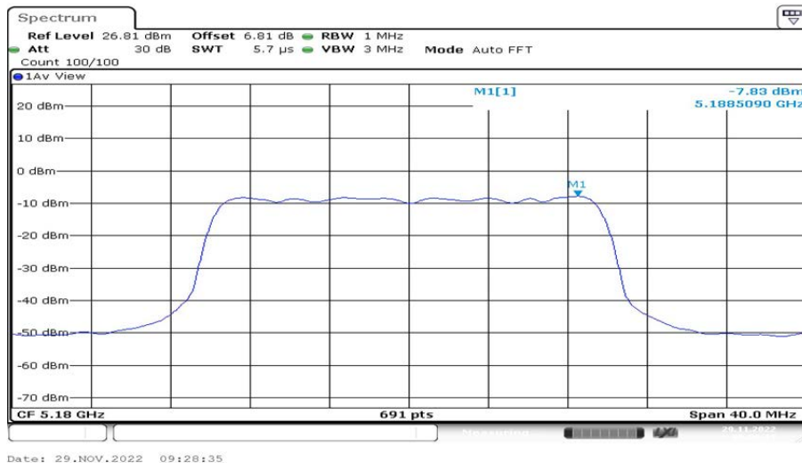
802.11ax(HE20)_Ant2_5180 106/53
