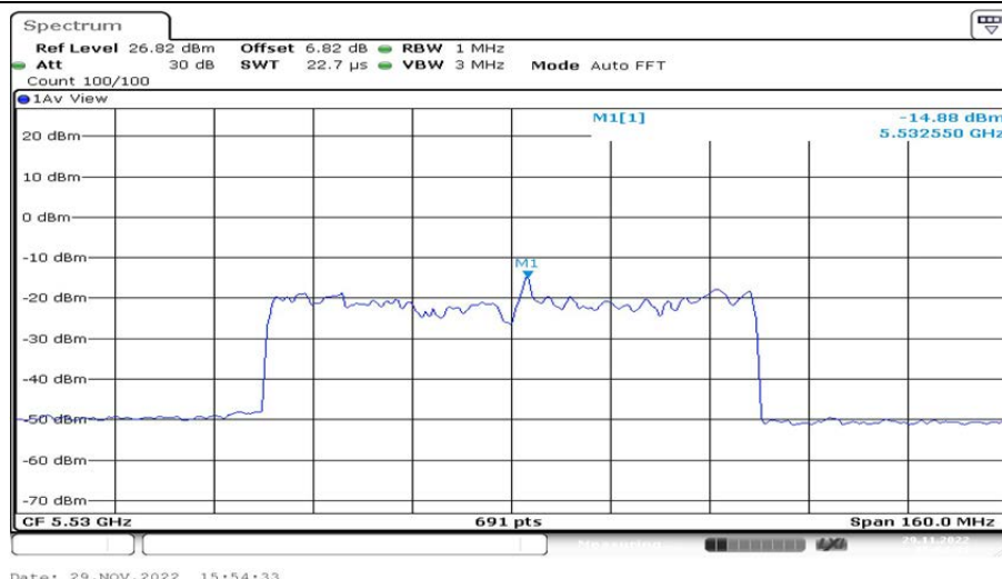
802.11ax(HE80)_Ant2_5530 26/19
