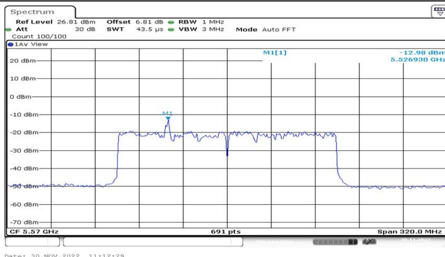
802.11ax(HE160)_Ant2_5570 52/44
