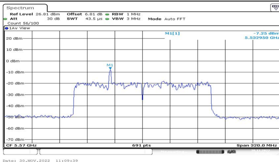
802.11ax(HE160)_Ant2_5570 26/19
