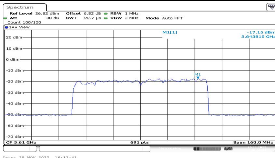
802.11ax(HE80)_Ant2_5610 26/19
