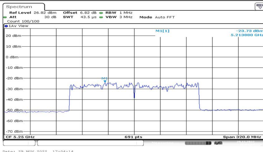
802.11ax(HE160)_Ant2_5250 484/66
