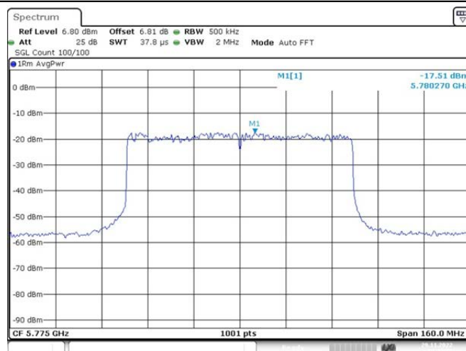
802.11ax(HE80)_Ant2_5775 26/19
