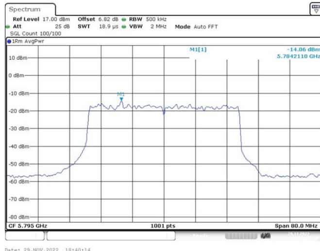
802.11ax(HE40)_Ant2_5795 106/54
