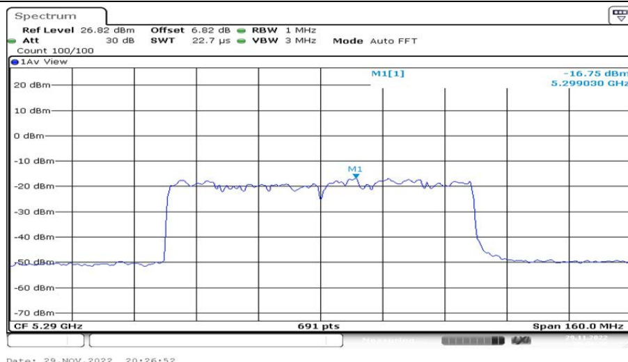
802.11ax(HE80)_Ant2_5290 106/56
