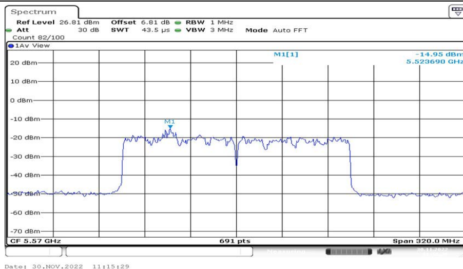
802.11ax(HE160)_Ant2_5570 106/56
