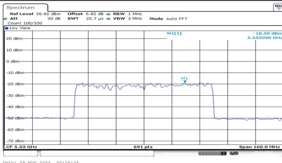
802.11ax(HE80)_Ant2_5530 106/56
