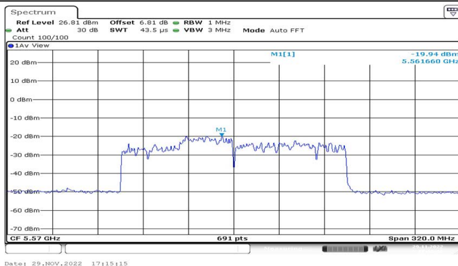
802.11ax(HE160)_Ant2_5570 484/66
