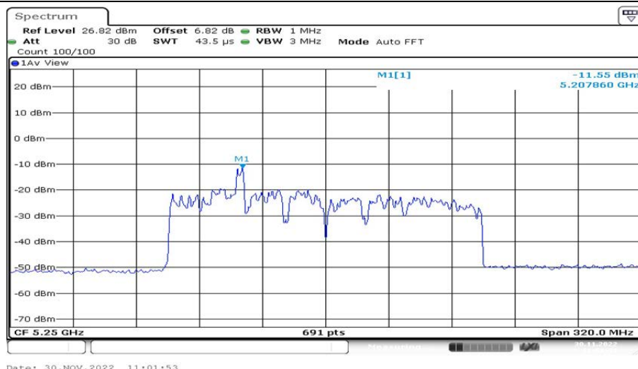
802.11ax(HE160)_Ant2_5250 52/44
