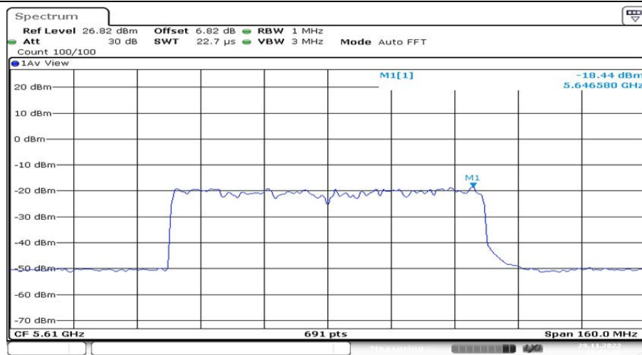
802.11ax(HE80)_Ant2_5610 484/65
