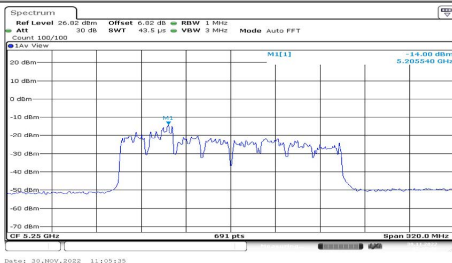
802.11ax(HE160)_Ant2_5250 106/56
