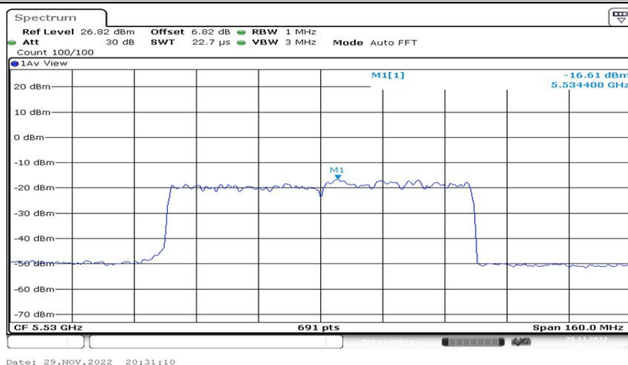
802.11ax(HE80)_Ant2_5530 52/44
