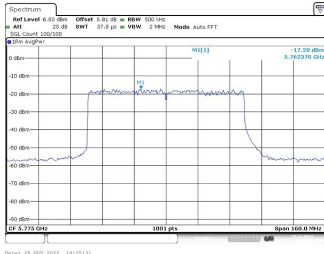
802.11ax(HE80)_Ant2_5775 106/56
