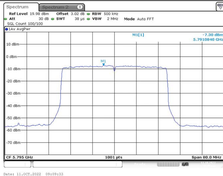
802.11ax(HE40)_Ant2_5795 484/65
