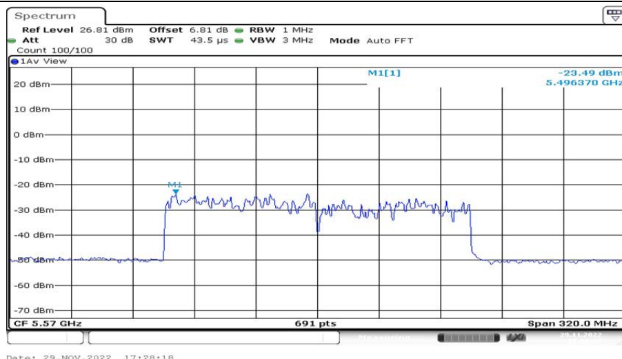
802.11ax(HE160)_Ant2_5570 996/67
