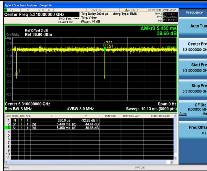
802.11n(HT40)_Ant2_5310
