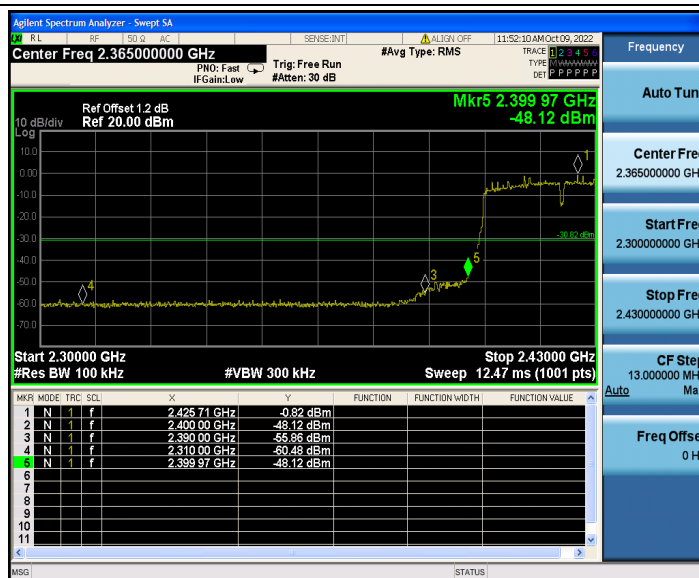
802.11n(HT40)_Ant2_Low_2422
