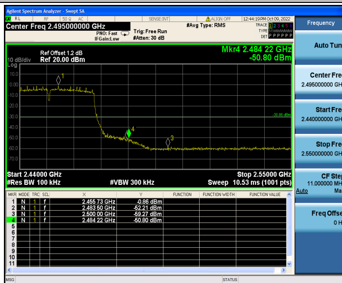
802.11n(HT40)_Ant2_High_2452
