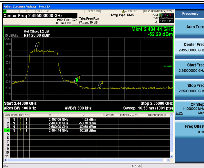
802.11ax(HE20)_Ant2_High_2462 242/61
