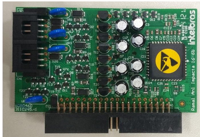
Extension analogic board
