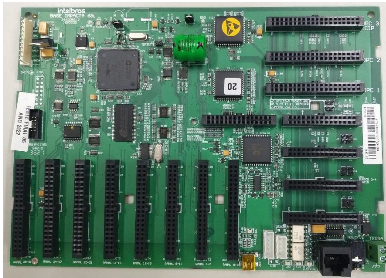
CPU board
