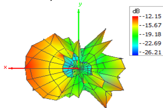
Theta = 180, Phi = 0
