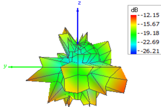
Theta = 90, Phi = 180
