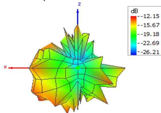
Theta = 90, Phi = 90
