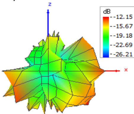
Theta = 90, Phi = 270
