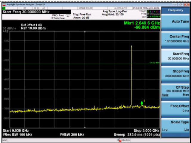
30MHz-3G
