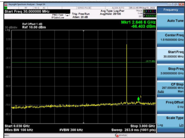
30MHz-3G
