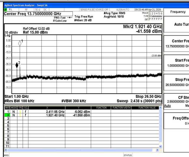
11B-Ant1-2412-1000~26500-PASS
