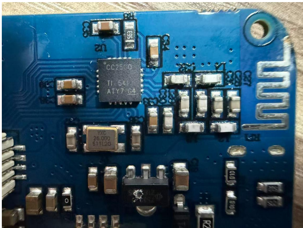
Internal Photos(IC2:CC2500)
