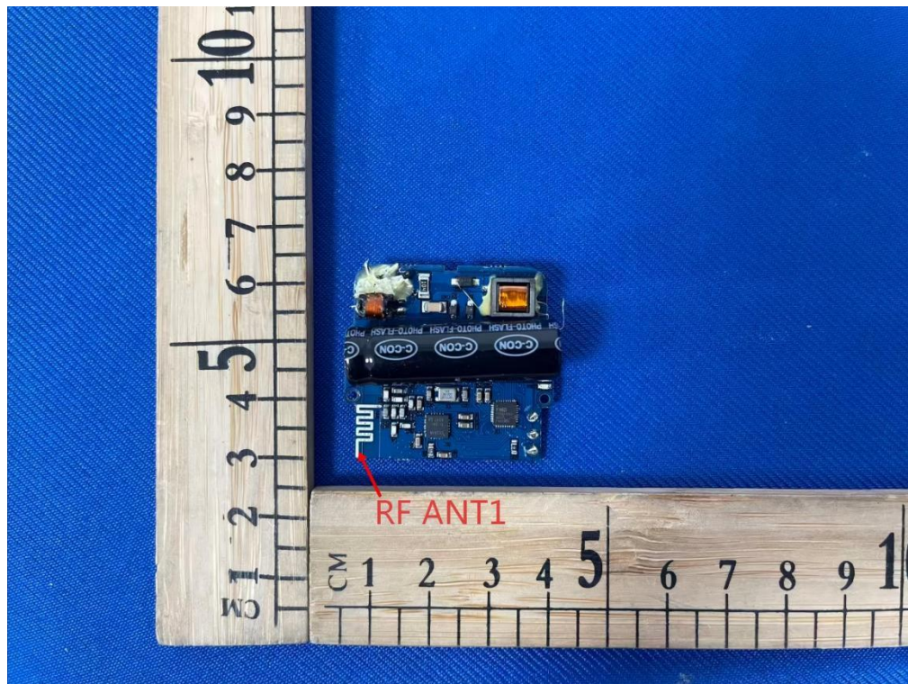
Internal Photos(IC1:CC2500)
