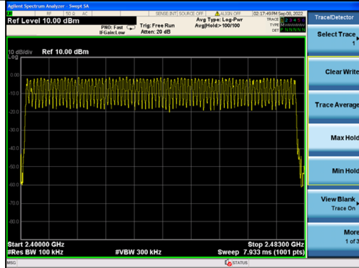
8DPSK Modulation
