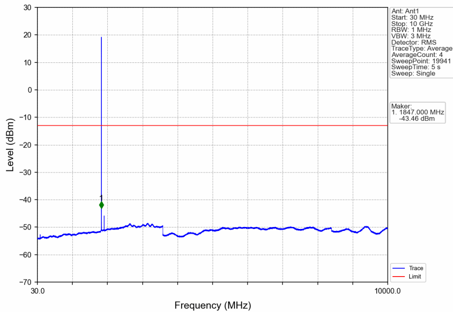
Band2_1.4MHz_16QAM_LCH_1850.7MHz_RB_1_0_NTNV
