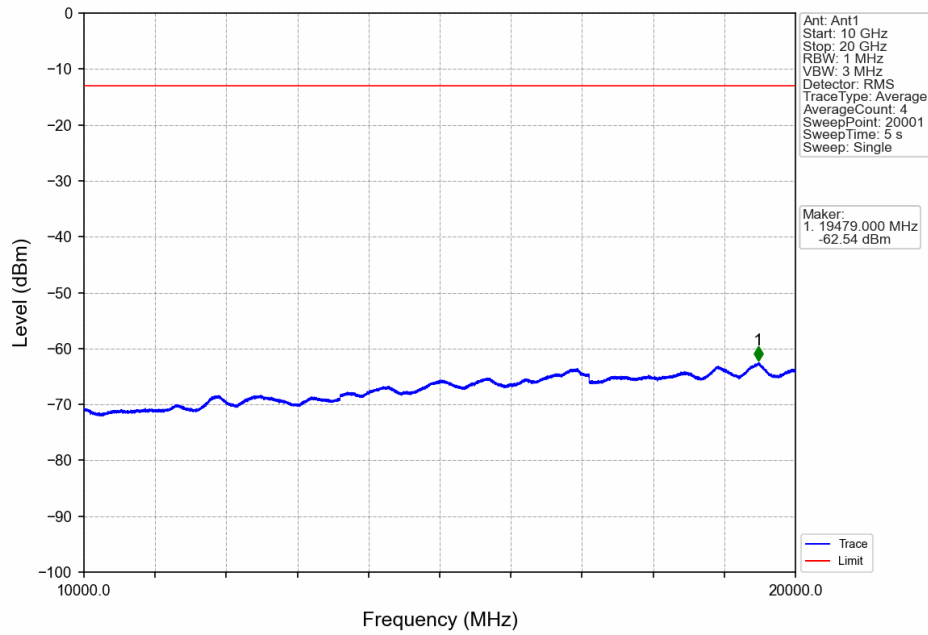
Band2_1.4MHz_QPSK_LCH_1850.7MHz_RB_6_0_NTNV
