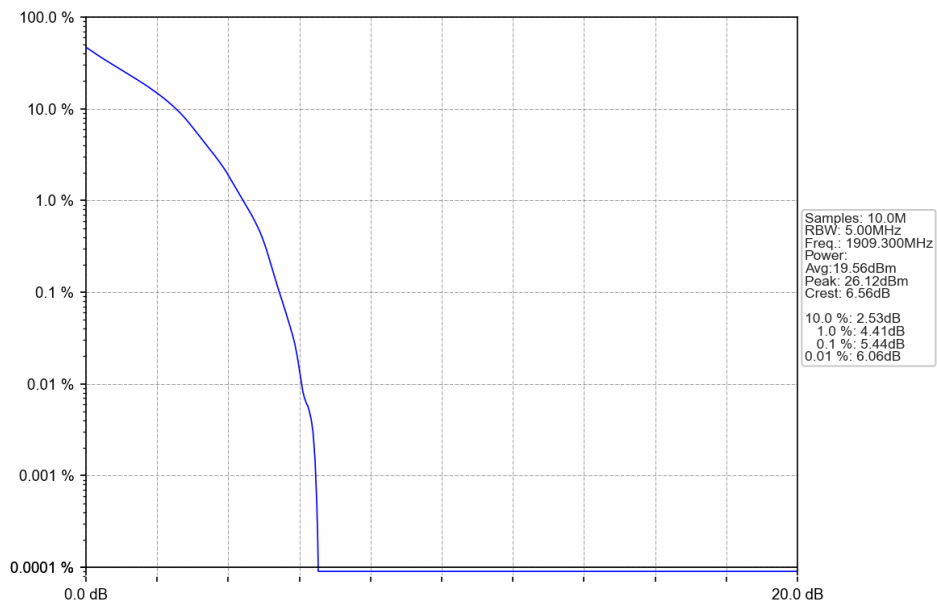
Band2_1.4MHz_QPSK_HCH_1909.3MHz_RB_6_0_NTNV
