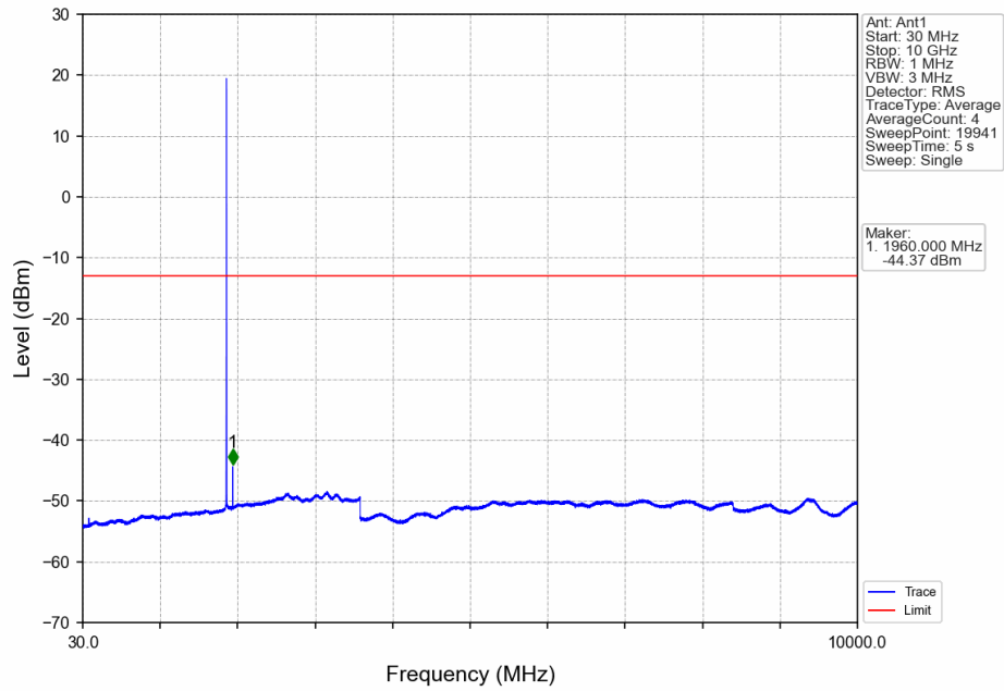
Band2_1.4MHz_16QAM_MCH_1880MHz_RB_1_0_NTNV
