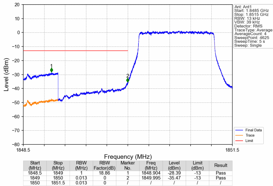
Band2_1.4MHz_16QAM_LCH_1850.7MHz_RB_6_0_NTNV
