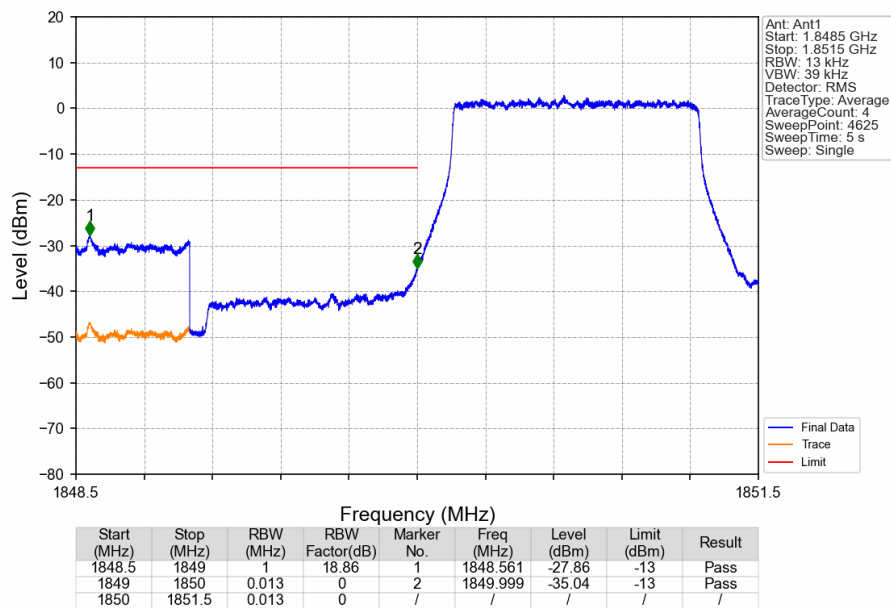
Band2_1.4MHz_QPSK_LCH_1850.7MHz_RB_6_0_NTNV
