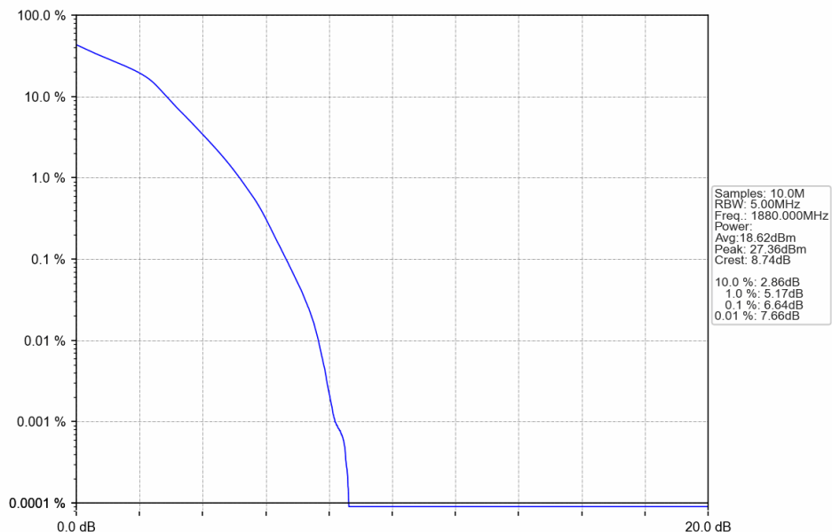
Band2_3MHz_16QAM_MCH_1880MHz_RB_15_0_NTNV
