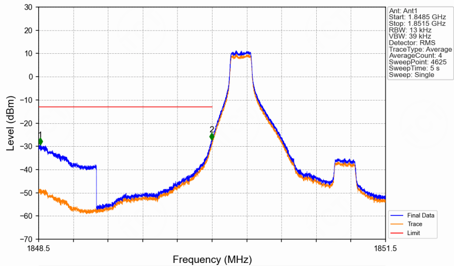
Band2_1.4MHz_16QAM_LCH_1850.7MHz_RB_1_0_NTNV
