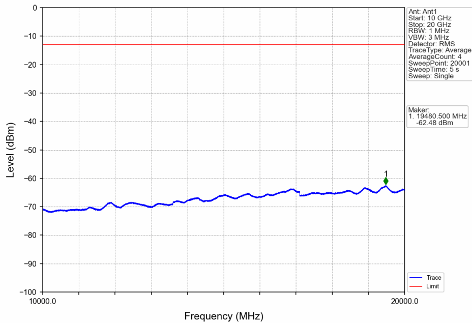
Band2_3MHz_QPSK_LCH_1851.5MHz_RB_15_0_NTNV
