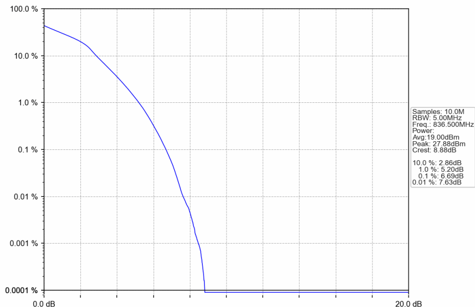
Band5_5MHz_16QAM_MCH_836.5MHz_RB_25_0_NTNV
