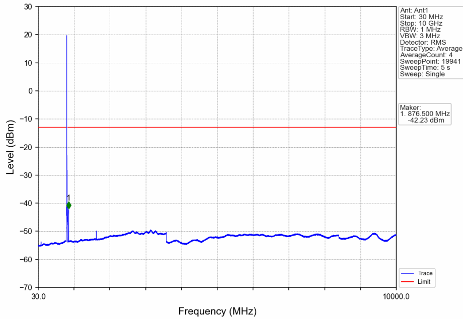
Band5_10MHz_16QAM_LCH_829MHz_RB_50_0_NTNV
