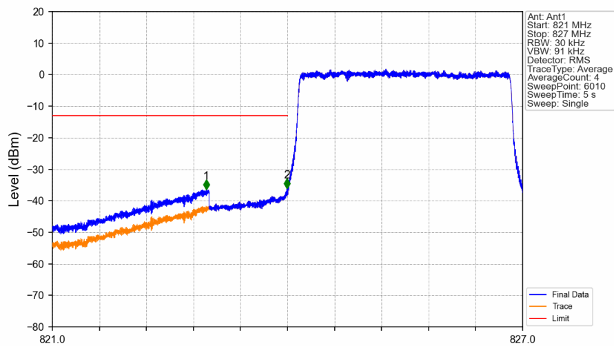
Band5_3MHz_16QAM_LCH_825.5MHz_RB_15_0_NTNV
