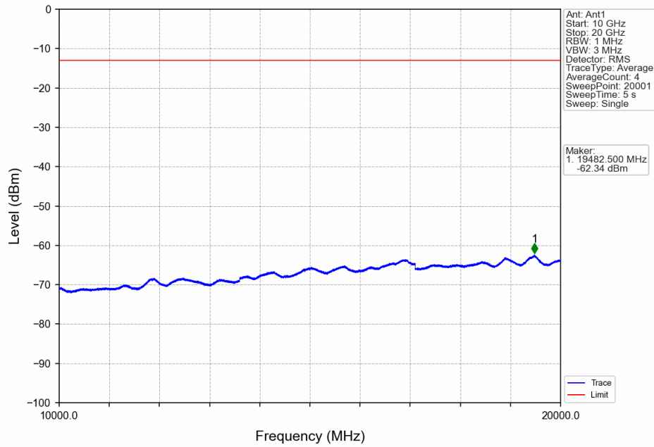
Band25_3MHz_QPSK_LCH_1851.5MHz_RB_15_0_NTNV
