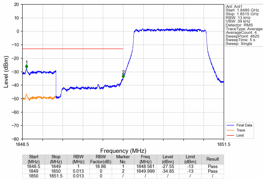
Band25_1.4MHz_QPSK_LCH_1850.7MHz_RB_6_0_NTNV
