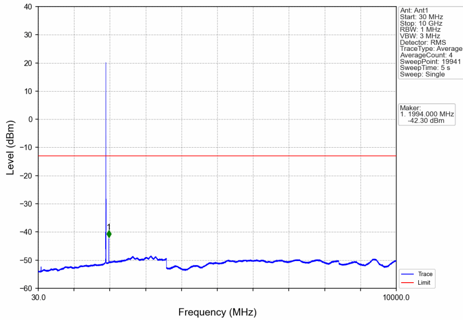
Band25_3MHz_QPSK_HCH_1913.5MHz_RB_1_0_NTNV
