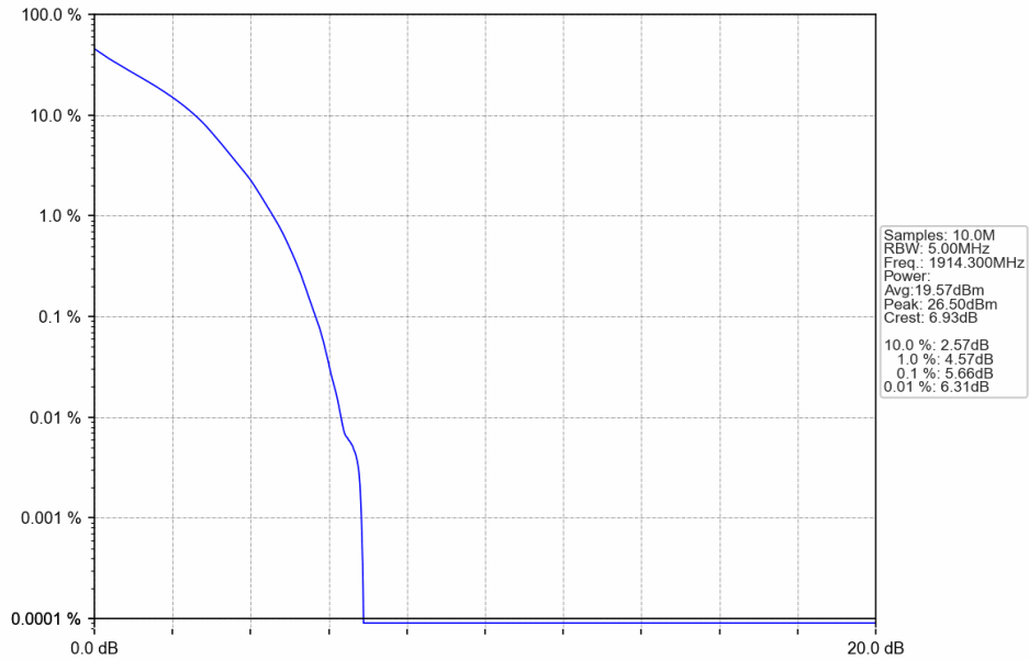
Band25_1.4MHz_QPSK_HCH_1914.3MHz_RB_6_0_NTNV
