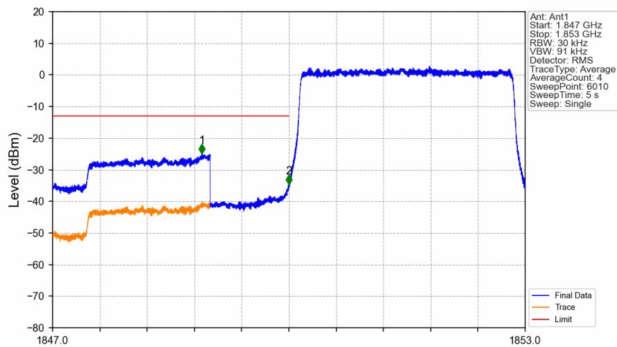
Band25_3MHz_QPSK_LCH_1851.5MHz_RB_15_0_NTNV
