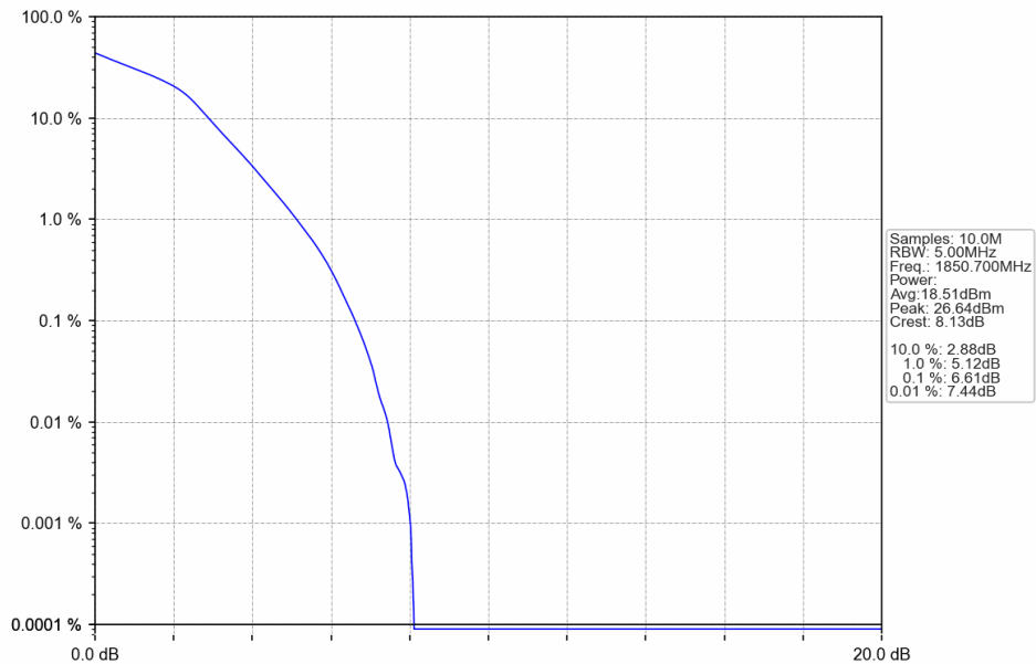
Band25_1.4MHz_16QAM_LCH_1850.7MHz_RB_6_0_NTNV
