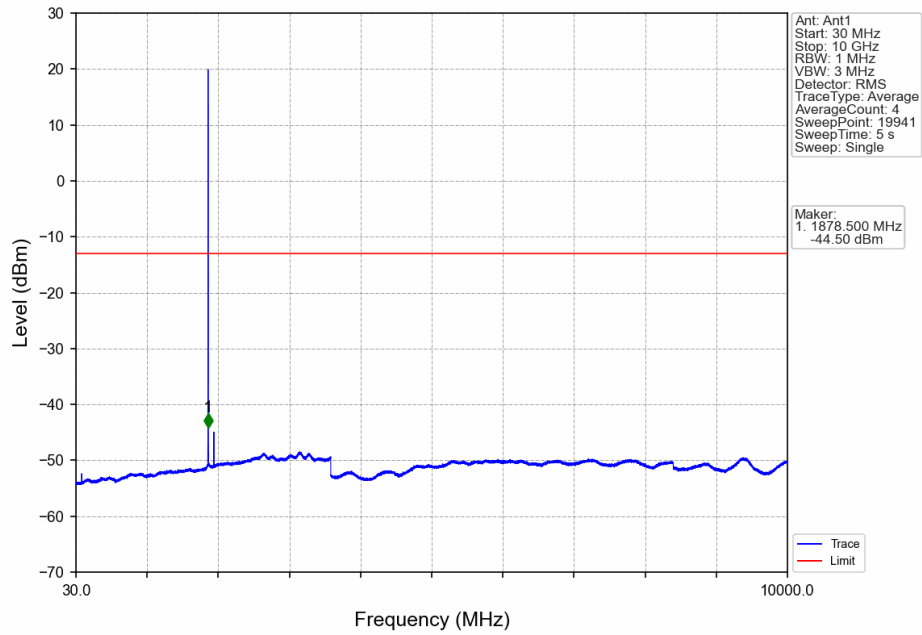
Band25_1.4MHz_16QAM_MCH_1882.5MHz_RB_1_0_NTNV
