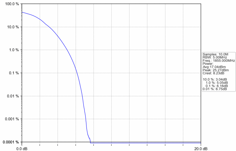
Band25_10MHz_16QAM_LCH_1855MHz_RB_50_0_NTNV
