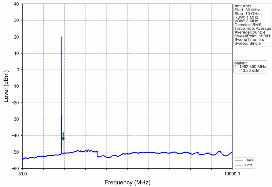
Band25_3MHz_QPSK_MCH_1882.5MHz_RB_1_0_NTNV
