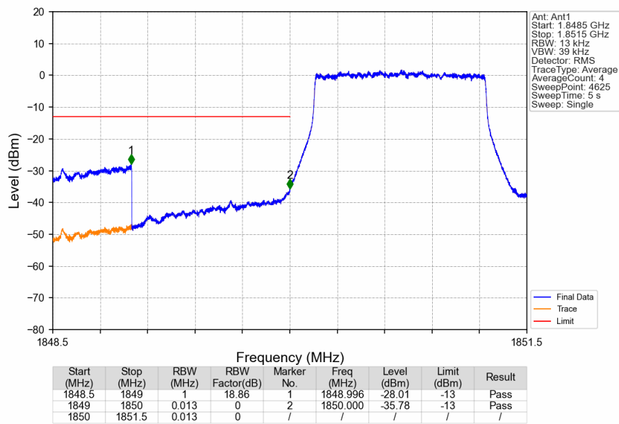
Band25_1.4MHz_16QAM_LCH_1850.7MHz_RB_6_0_NTNV
