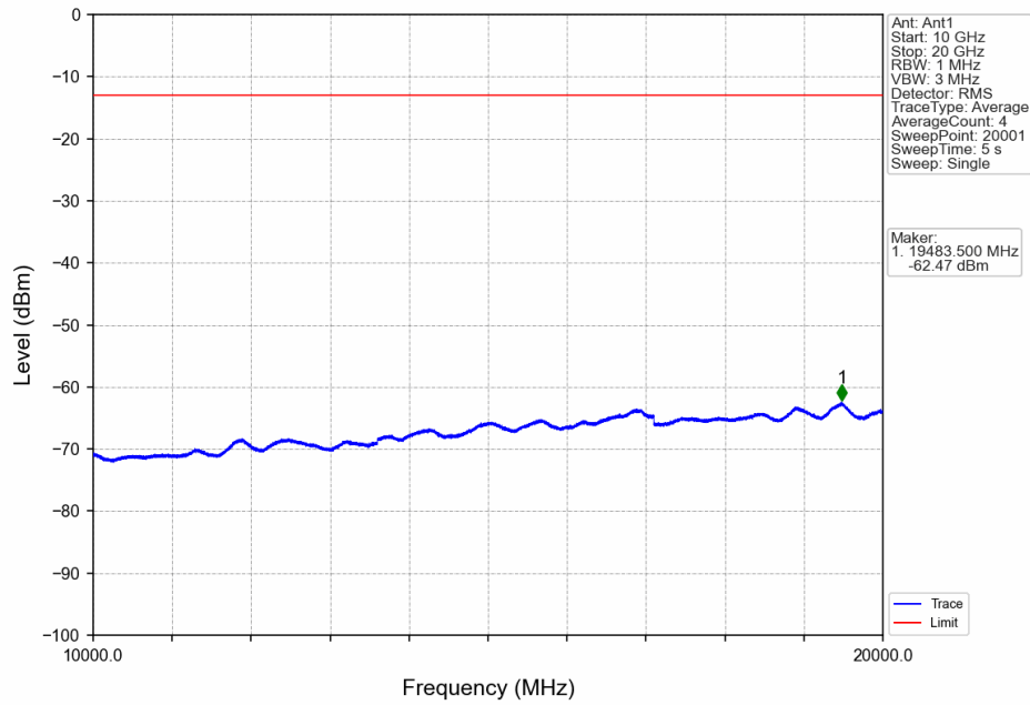
Band25_1.4MHz_16QAM_LCH_1850.7MHz_RB_6_0_NTNV
