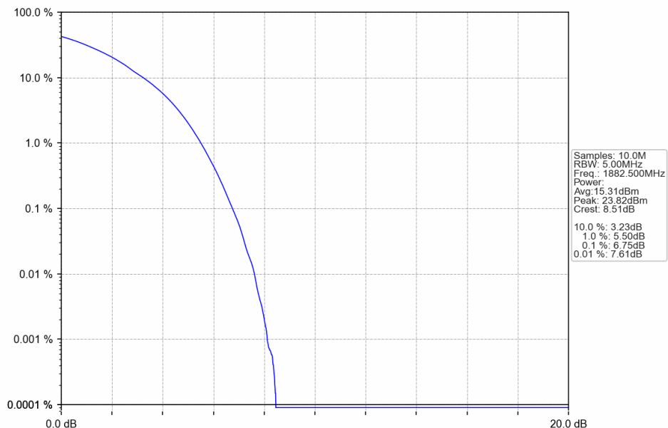
Band25_15MHz_16QAM_MCH_1882.5MHz_RB_75_0_NTNV
