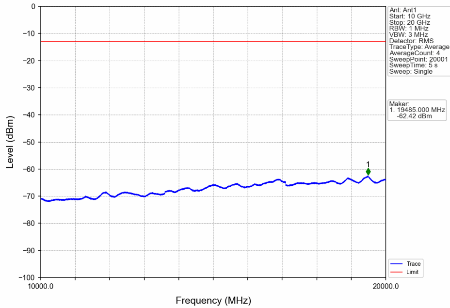
Band25_1.4MHz_QPSK_LCH_1850.7MHz_RB_6_0_NTNV
