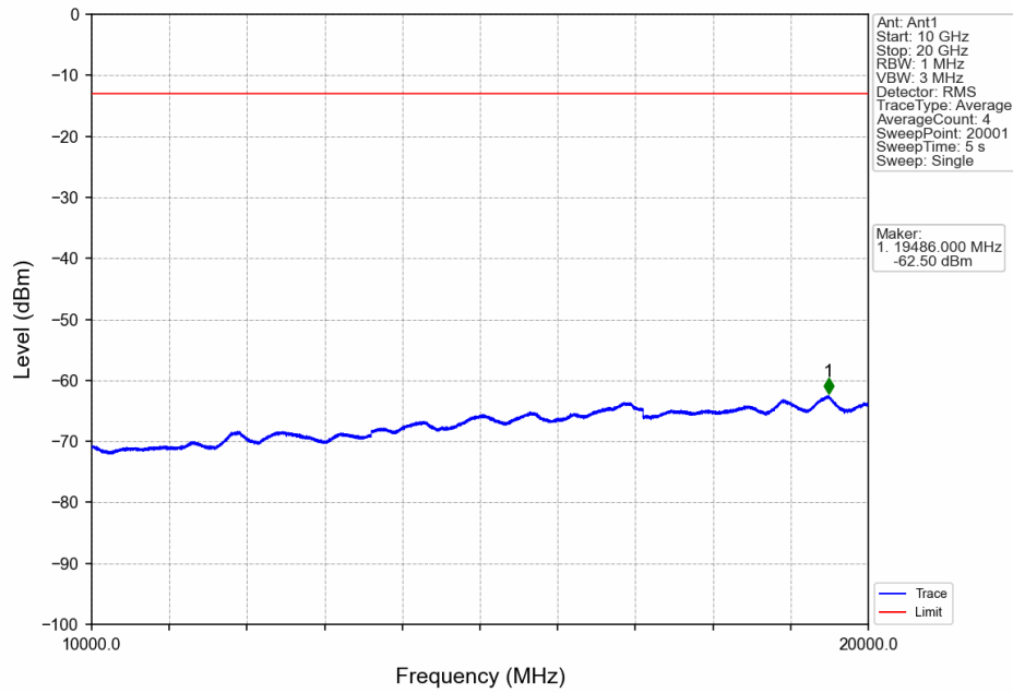
Band25_20MHz_16QAM_LCH_1860MHz_RB_100_0_NTNV
