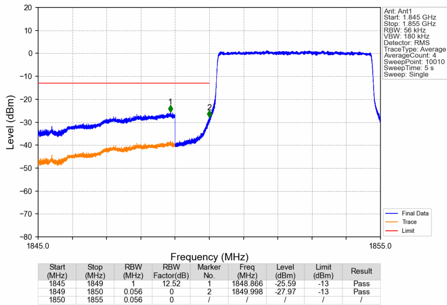
Band25_5MHz_16QAM_LCH_1852.5MHz_RB_25_0_NTNV
