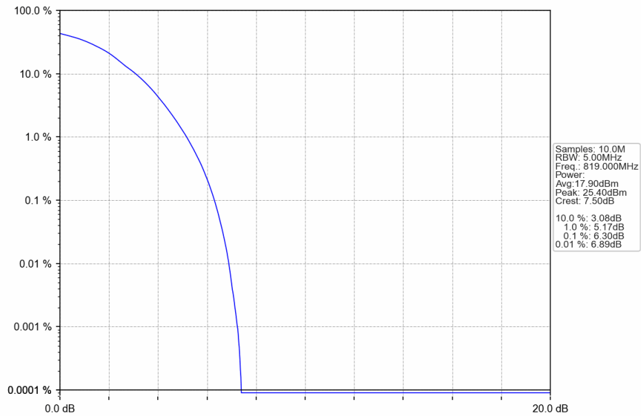
Band26a_10MHz_16QAM_HCH_819MHz_RB_50_0_NTNV
