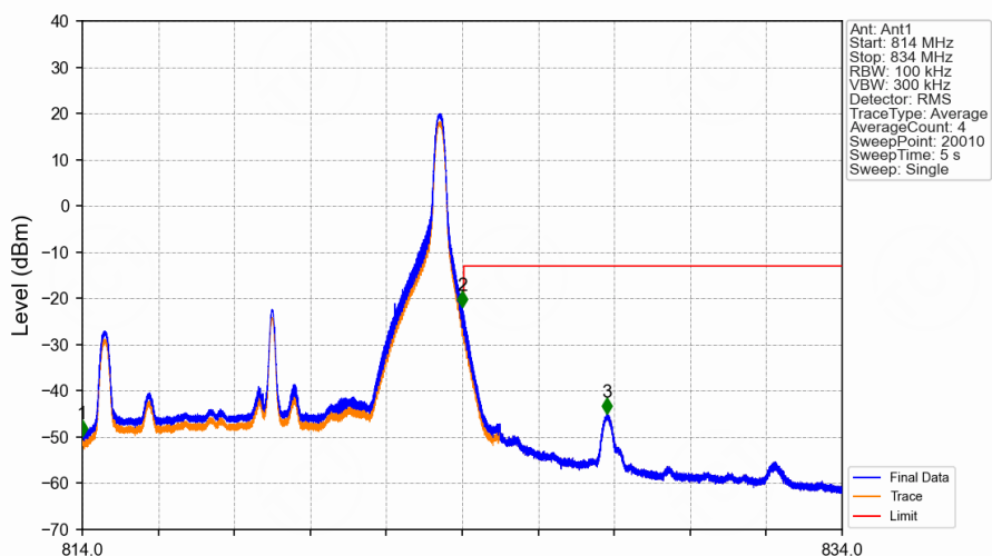
Band26a_10MHz_16QAM_HCH_819MHz_RB_1_49_NTNV
