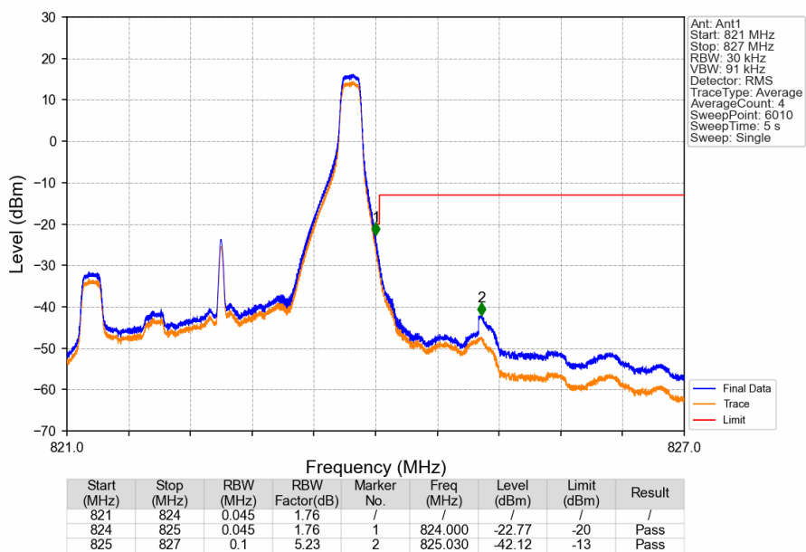
Band26a_3MHz_QPSK_HCH_822.5MHz_RB_1_14_NTNV
