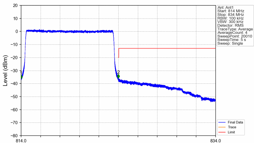
Band26a_10MHz_16QAM_HCH_819MHz_RB_50_0_NTNV
