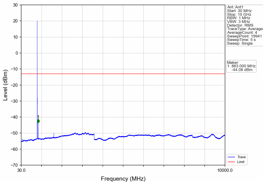
Band26a_5MHz_16QAM_LCH_816.5MHz_RB_25_0_NTNV
