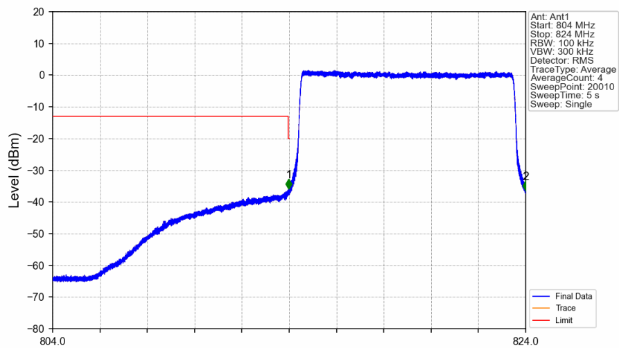
Band26a_10MHz_16QAM_LCH_819MHz_RB_50_0_NTNV
