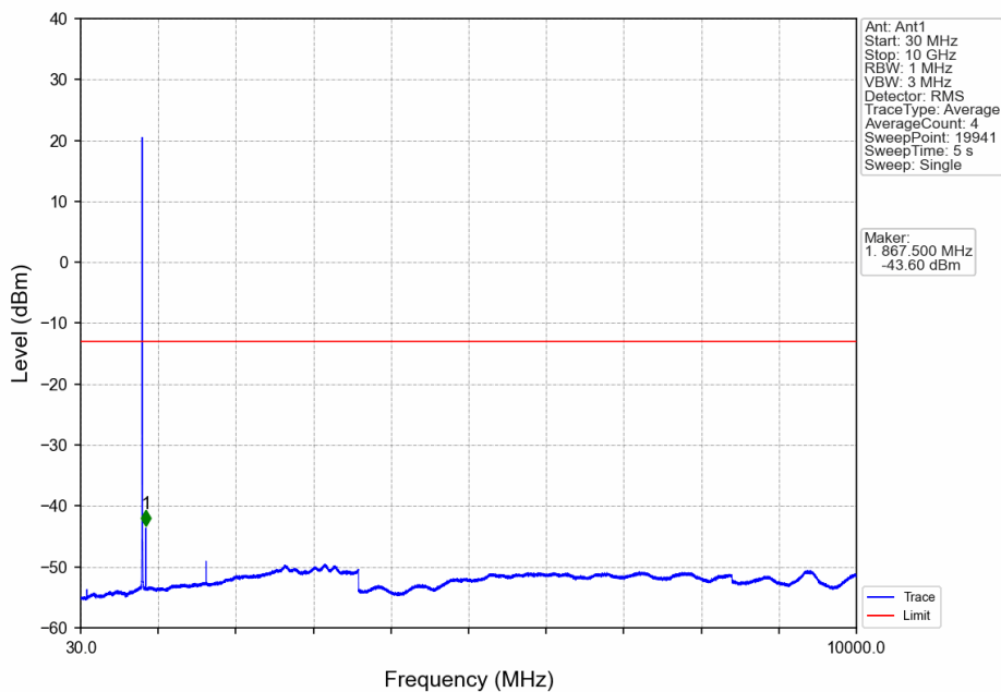
Band26a_3MHz_QPSK_HCH_822.5MHz_RB_1_14_NTNV
