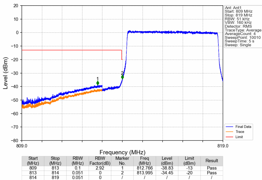
Band26a_5MHz_16QAM_LCH_816.5MHz_RB_25_0_NTNV
