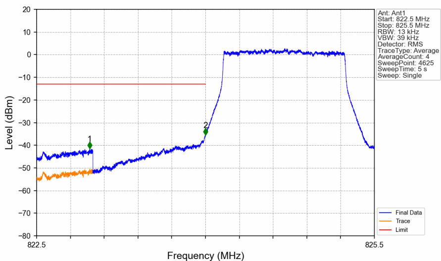
Band26b 1.4MHz 16QAM LCH 824.7MHz RB 6 0 NTN
