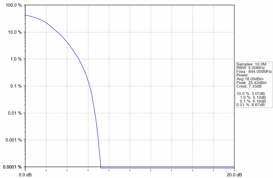
Band26b 10MHz 16QAM HCH 844MHz RB 50 0 NTN
