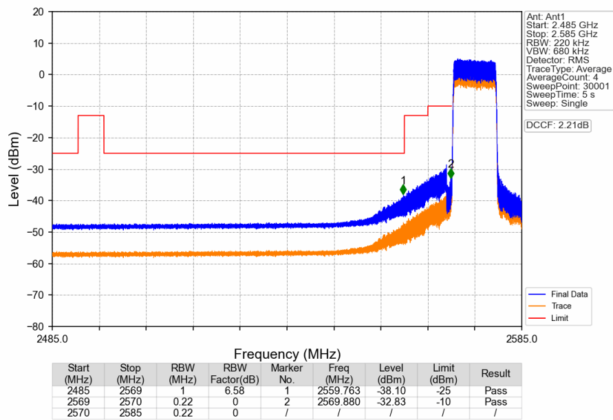
Band38_10MHz_16QAM_LCH_2575MHz_RB_50_0_NTNV
