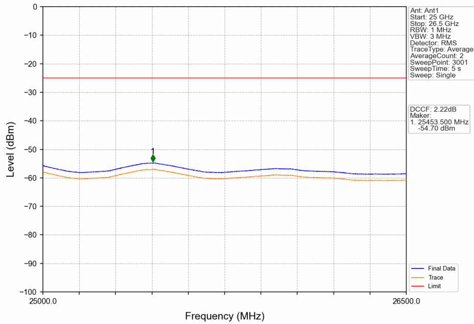
Band38_15MHz_QPSK_HCH_2612.5MHz_RB_1_74_NTNV
