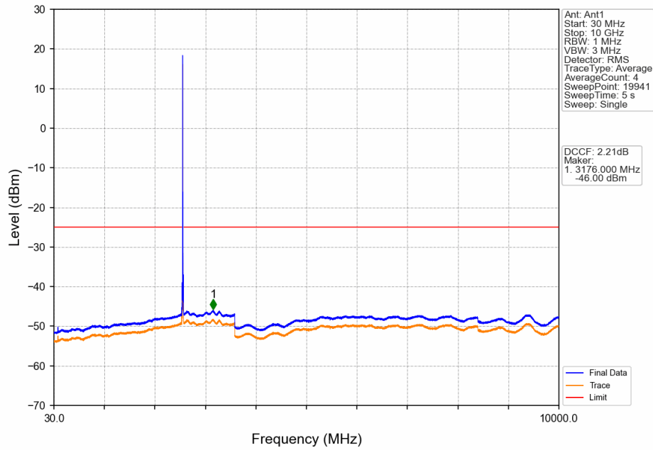
Band38_10MHz_16QAM_LCH_2575MHz_RB_1_0_NTNV
