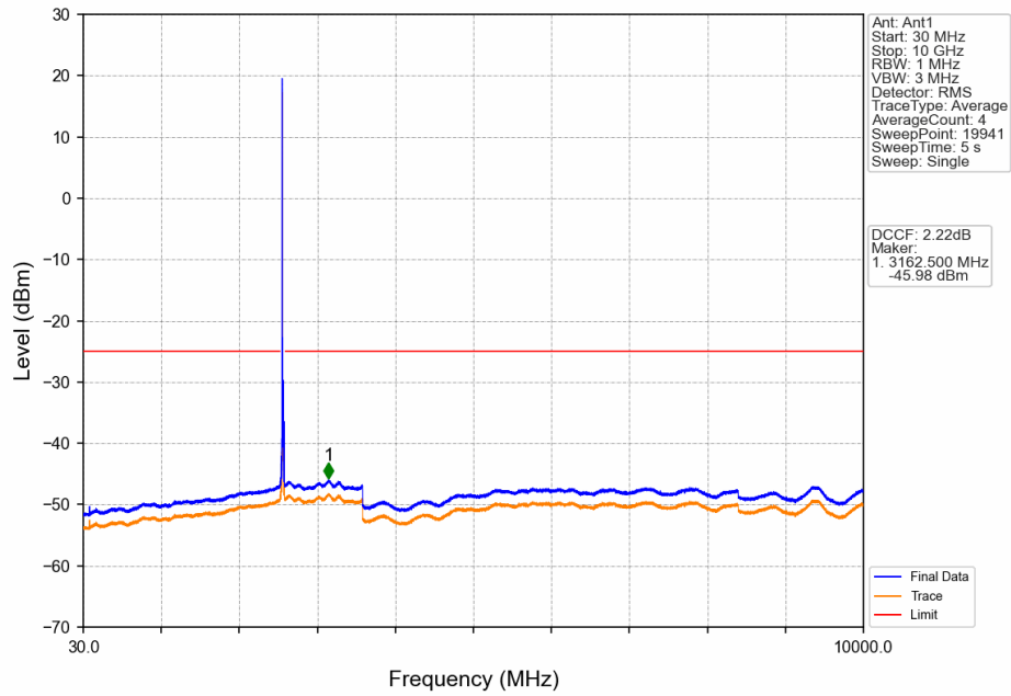
Band38_15MHz_16QAM_LCH_2577.5MHz_RB_1_0_NTNV
