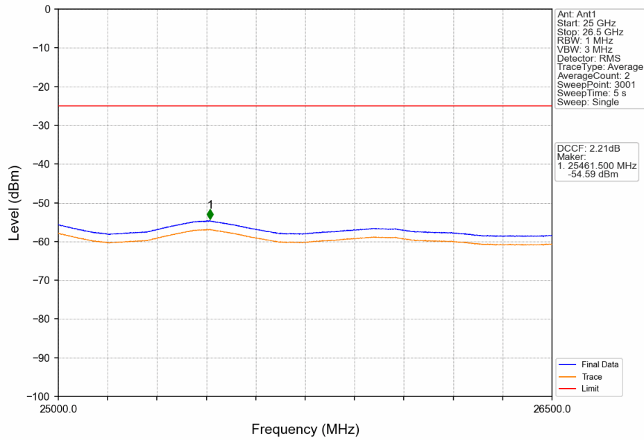
Band38_10MHz_16QAM_LCH_2575MHz_RB_50_0_NTNV
