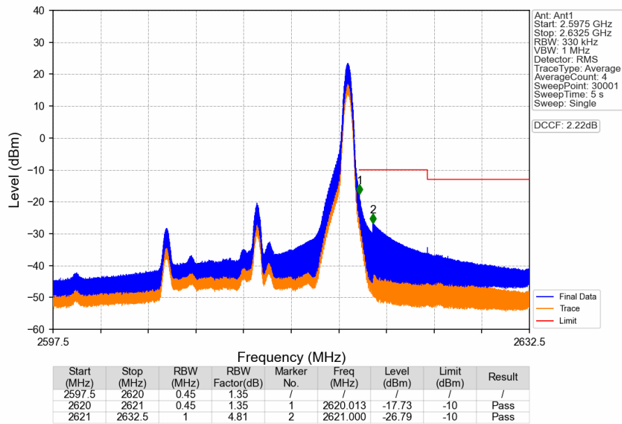
Band38_15MHz_QPSK_HCH_2612.5MHz_RB_1_74_NTNV
