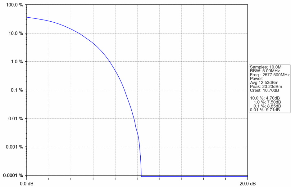
Band38_15MHz_16QAM_LCH_2577.5MHz_RB_75_0_NTNV
