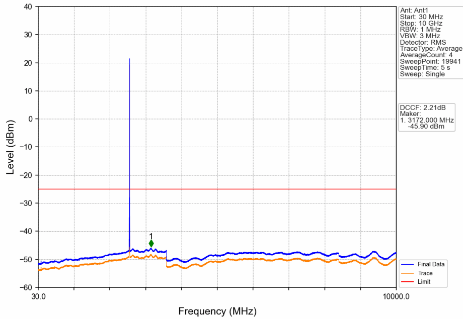
Band38_5MHz_16QAM_LCH_2572.5MHz_RB_1_0_NTNV
