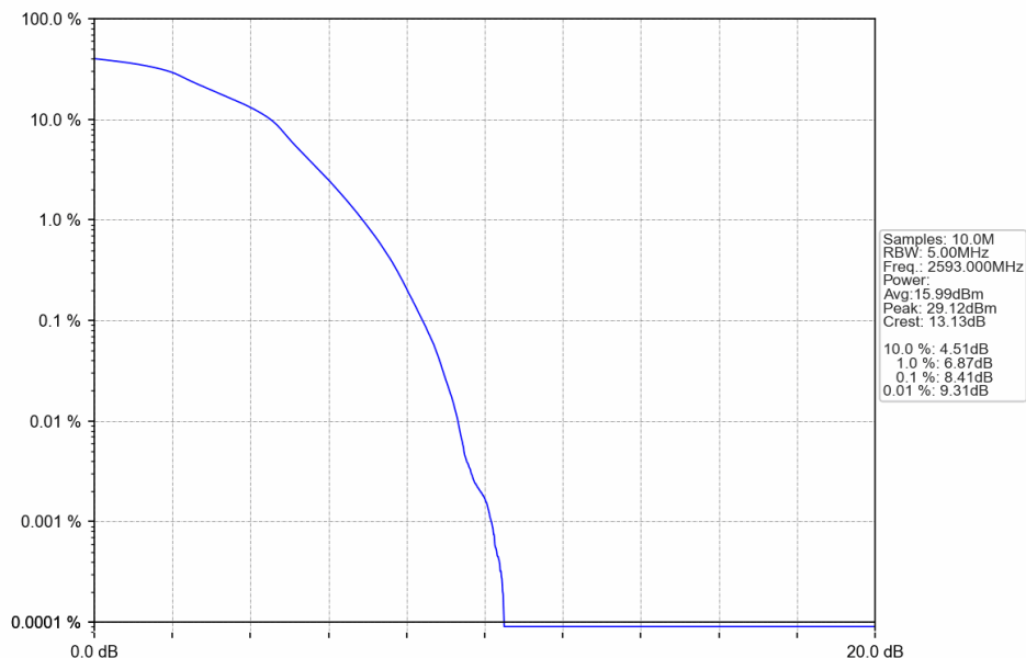
Band41_5MHz_16QAM_MCH_2593MHz_RB_25_0_NTNV
