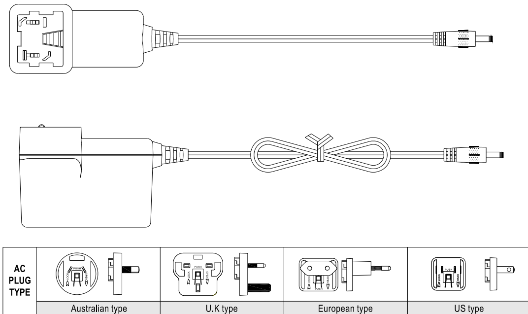
Figure 2: Power adaptor
