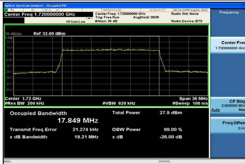
Band4-20MHz-16QAM-20050-100RB#0-17.849
