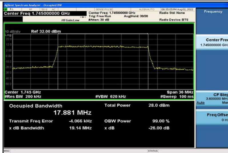
Band4-20MHz-16QAM-20300-100RB#0-17.881
