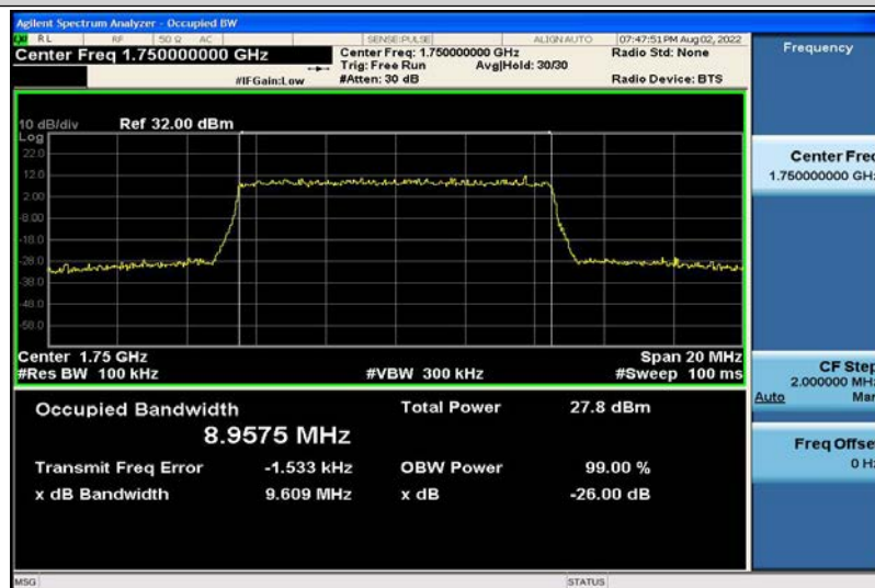
Band4-10MHz-16QAM-20350-50RB#0-8.9575
