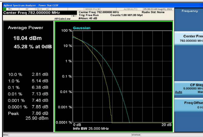
Band13-10MHz-16QAM-23230-50RB#0
