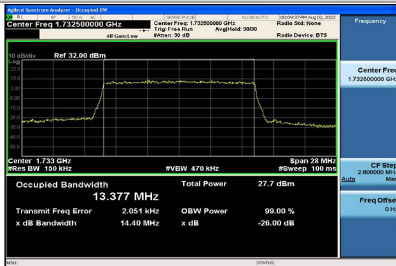
Band4-15MHz-QPSK-20175-75RB#0-13.377
