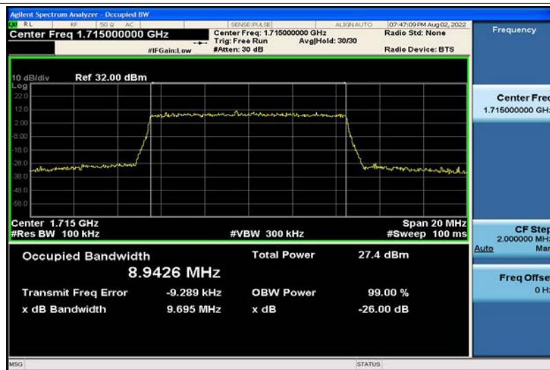
Band4-10MHz-16QAM-20000-50RB#0-8.9426
