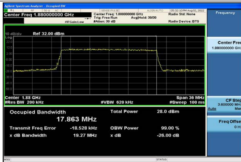
Band2-20MHz-QPSK-18900-100RB#0-17.863
