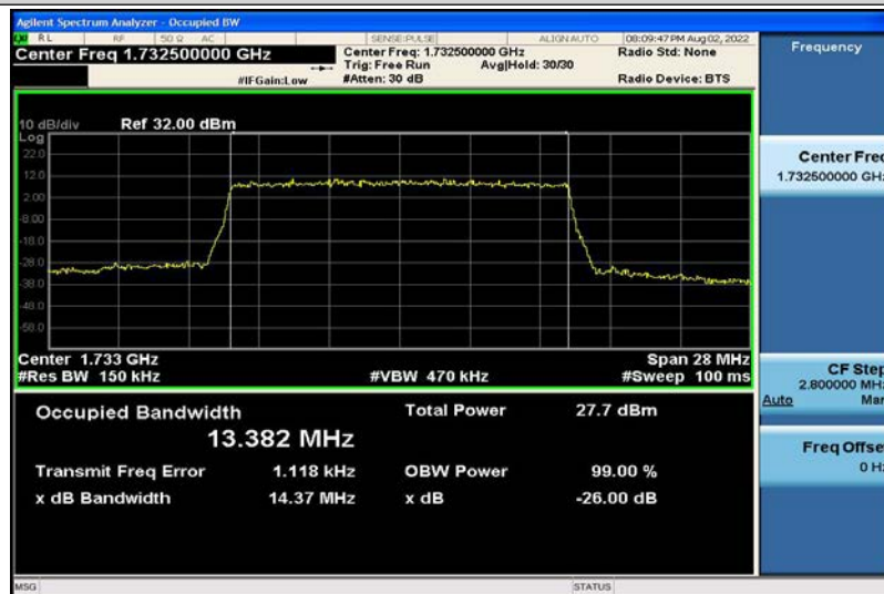
Band4-15MHz-16QAM-20175-75RB#0-13.382
