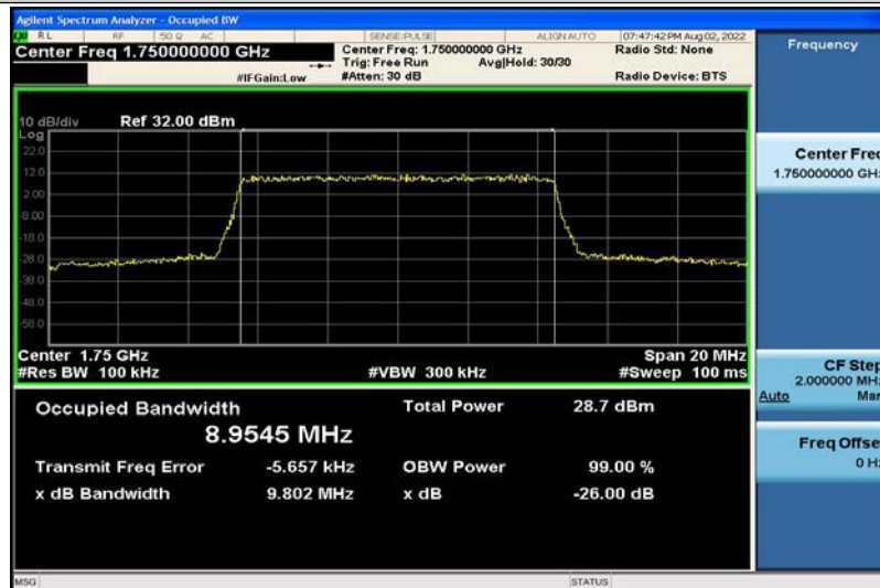
Band4-10MHz-QPSK-20350-50RB#0-8.9545
