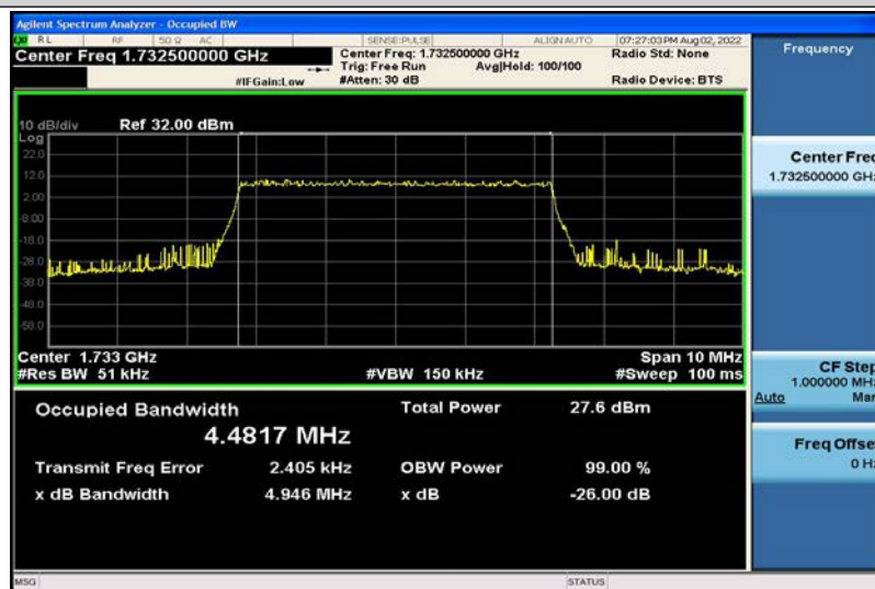
Band4-5MHz-16QAM-20175-25RB#0-4.4817
