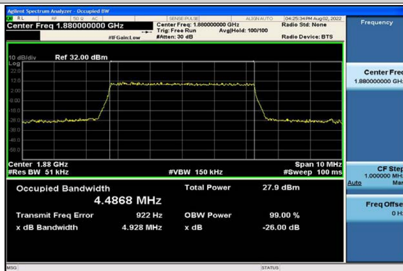
Band2-5MHz-16QAM-18900-25RB#0-4.4868
