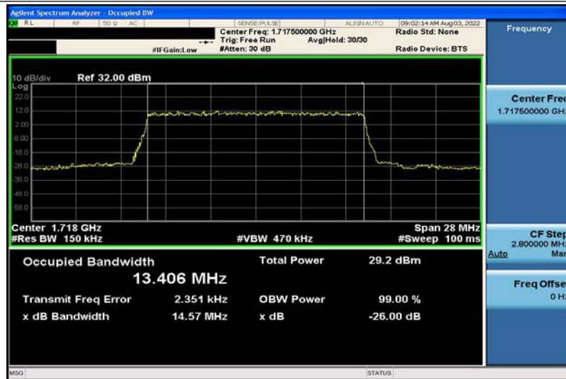
Band4-15MHz-QPSK-20025-75RB#0-13.406
