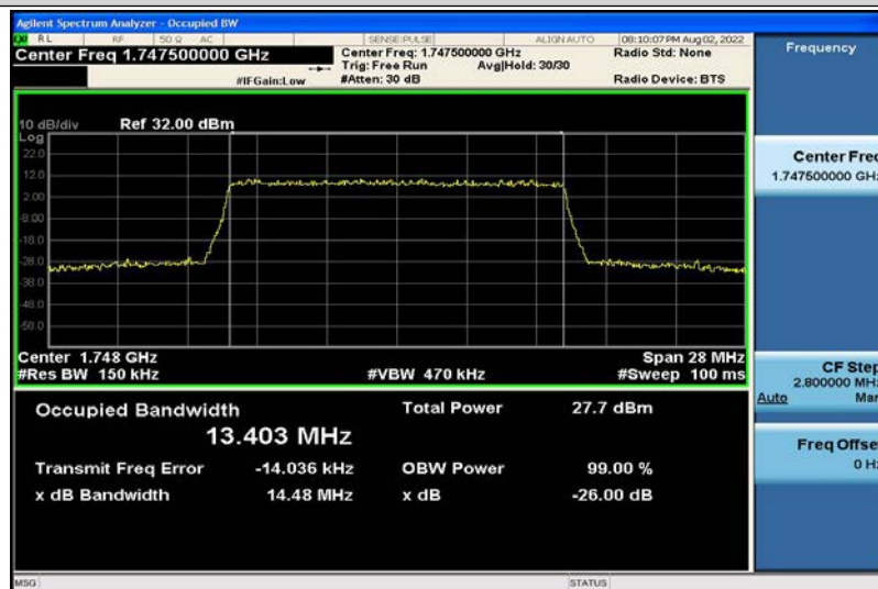
Band4-15MHz-16QAM-20325-75RB#0-13.403
