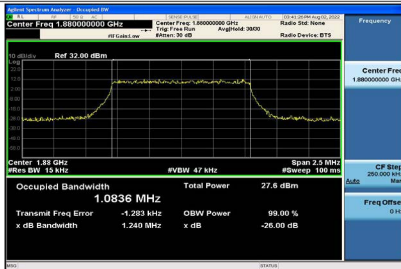
Band2-1.4MHz-QPSK-18900-6RB#0-1.0836
