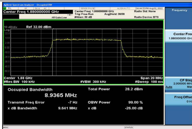
Band2-10MHz-16QAM-18900-50RB#0-8.9365
