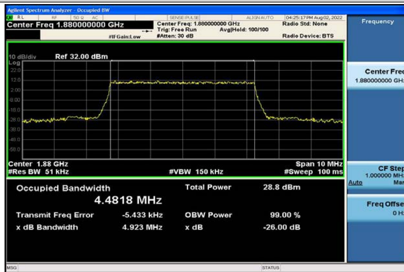
Band2-5MHz-QPSK-18900-25RB#0-4.4818
