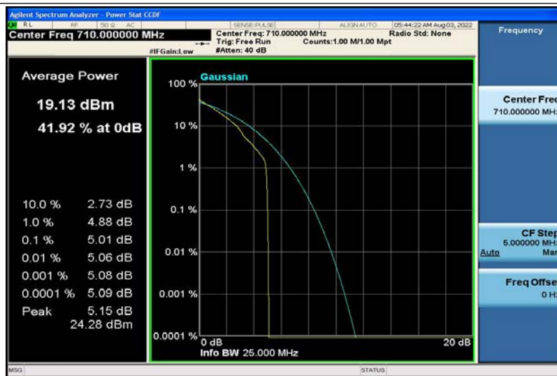
Band17-10MHz-QPSK-23790-1RB#0
