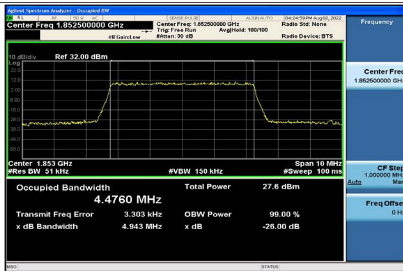
Band2-5MHz-16QAM-18625-25RB#0-4.4760
