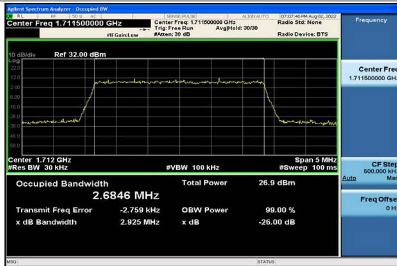
Band4-3MHz-16QAM-19965-15RB#0-2.6846
