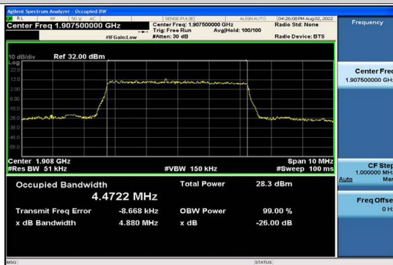
Band2-5MHz-16QAM-19175-25RB#0-4.4722
