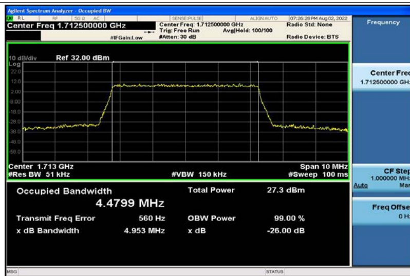
Band4-5MHz-16QAM-19975-25RB#0-4.4799
