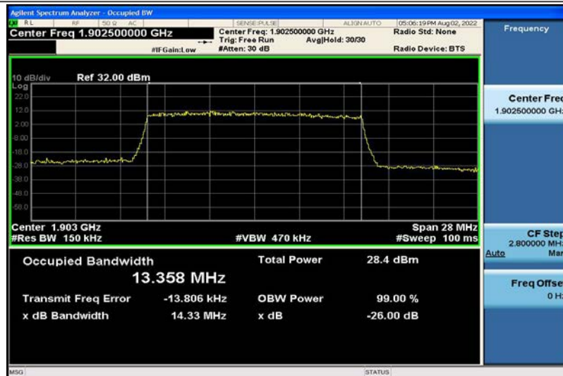
Band2-15MHz-16QAM-19125-75RB#0-13.358
