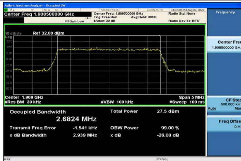
Band2-3MHz-16QAM-19185-15RB#0-2.6824
