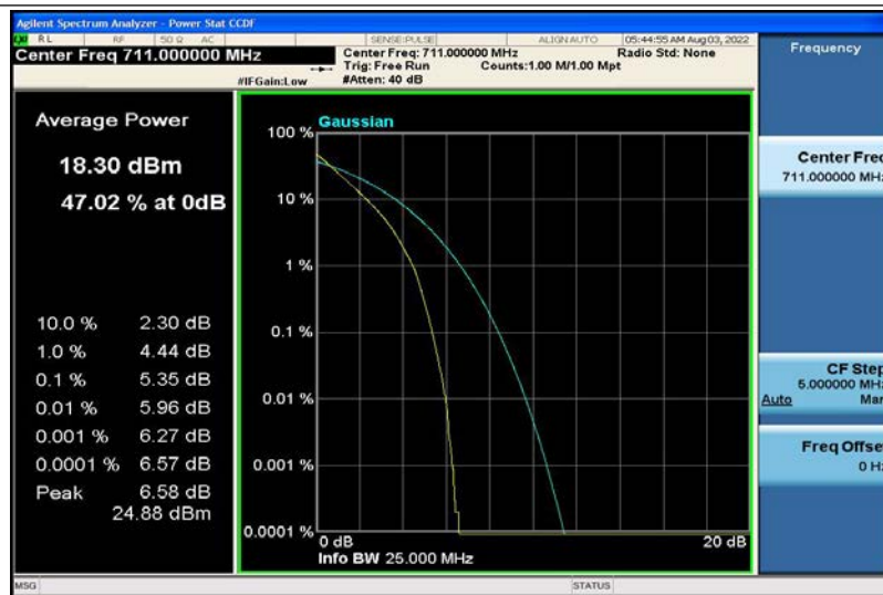
Band17-10MHz-QPSK-23800-50RB#0
