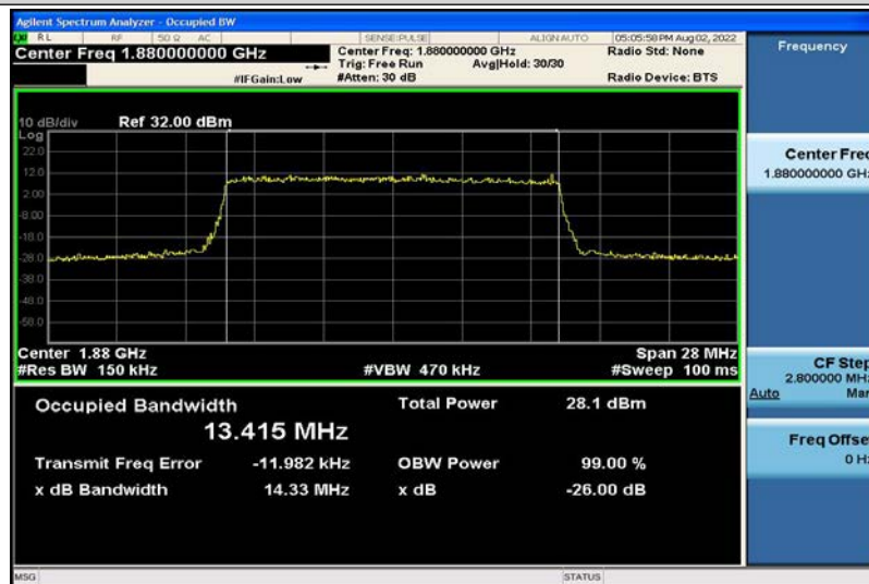
Band2-15MHz-16QAM-18900-75RB#0-13.415
