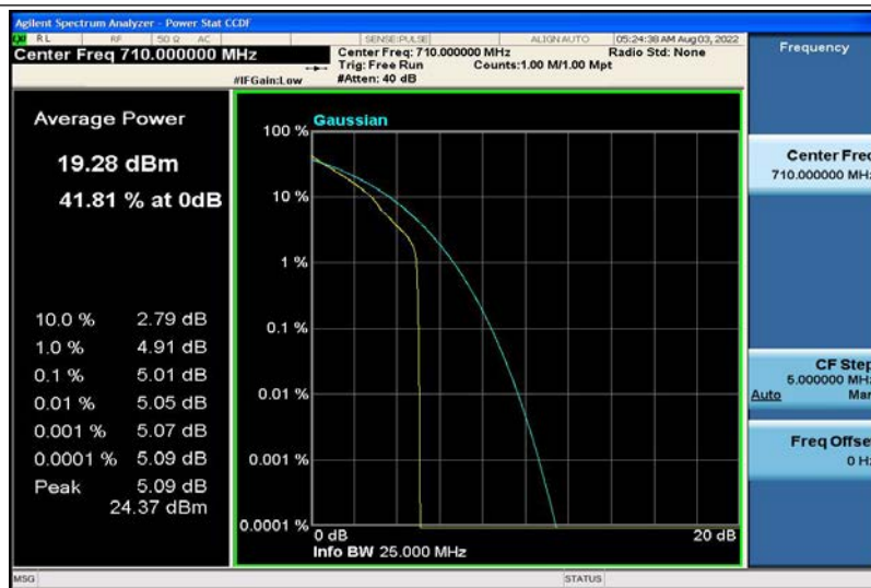
Band17-5MHz-QPSK-23790-1RB#0
