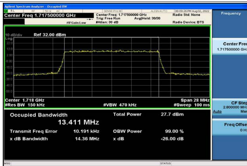
Band4-15MHz-16QAM-20025-75RB#0-13.411
