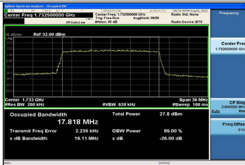
Band4-20MHz-QPSK-20175-100RB#0-17.818
