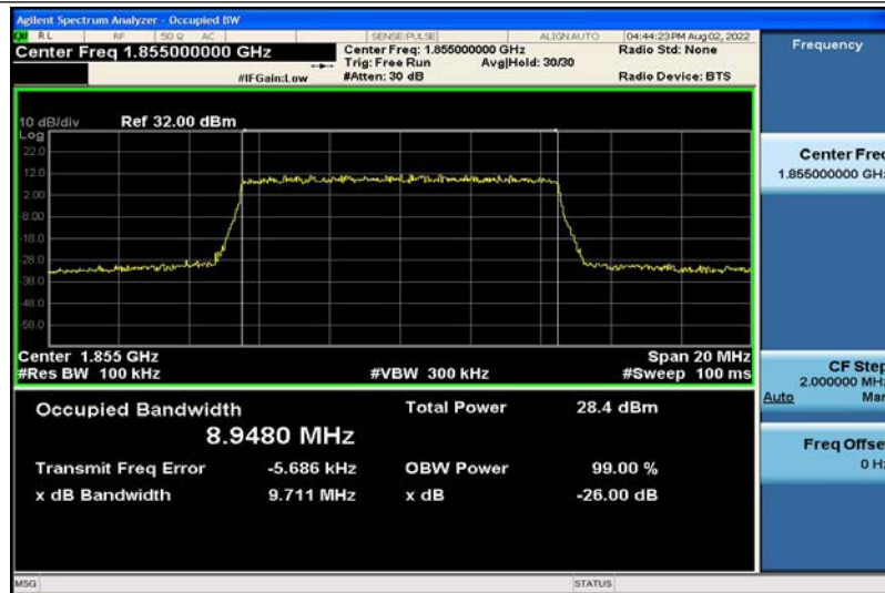
Band2-10MHz-QPSK-18650-50RB#0-8.9480
