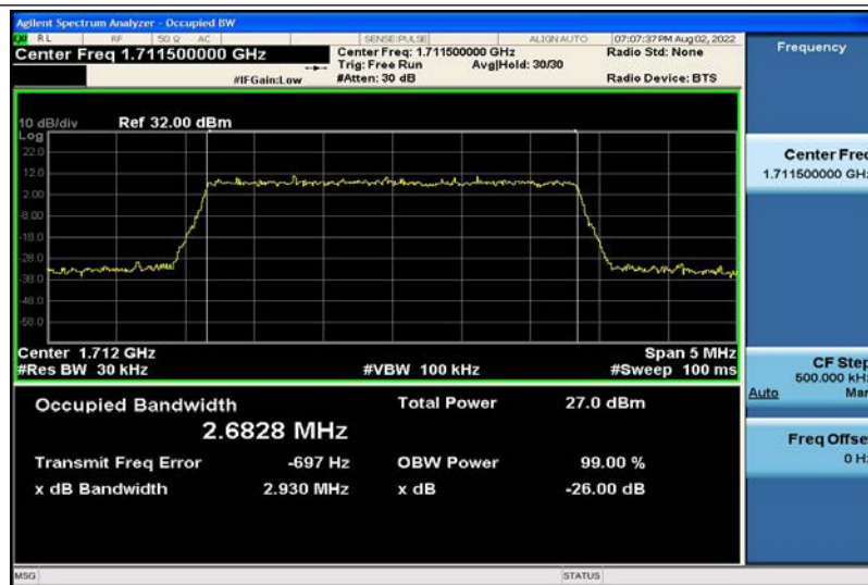
Band4-3MHz-QPSK-19965-15RB#0-2.6828
