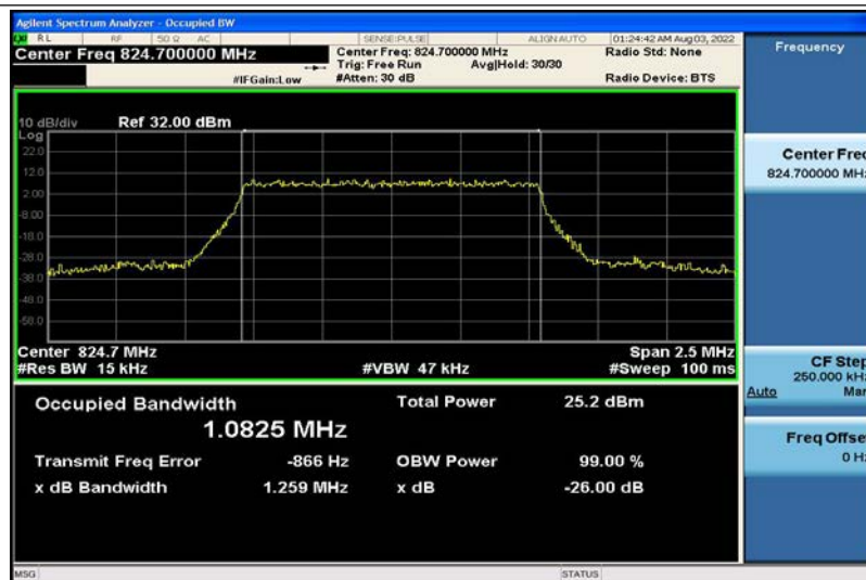
Band5-1.4MHz-16QAM-20407-6RB#0-1.0825
