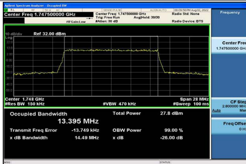
Band4-15MHz-QPSK-20325-75RB#0-13.395
