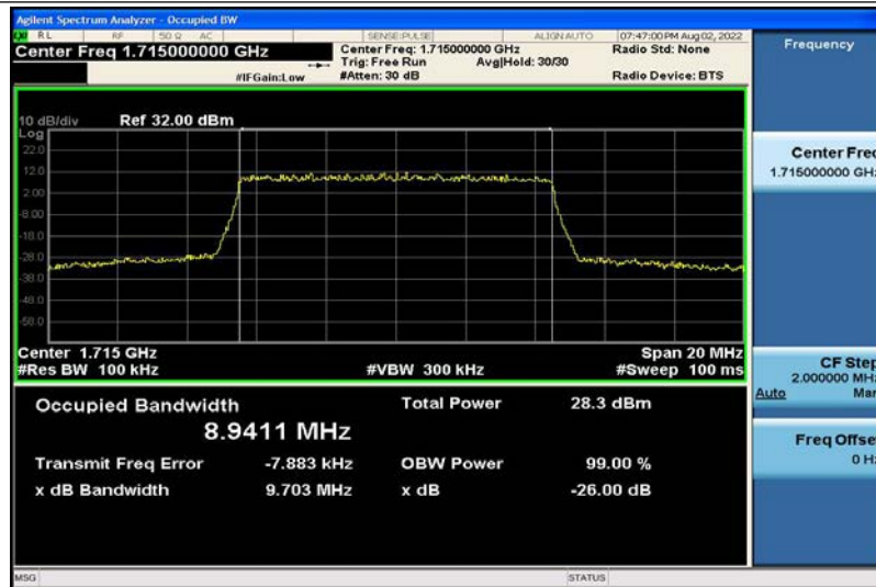
Band4-10MHz-QPSK-20000-50RB#0-8.9411
