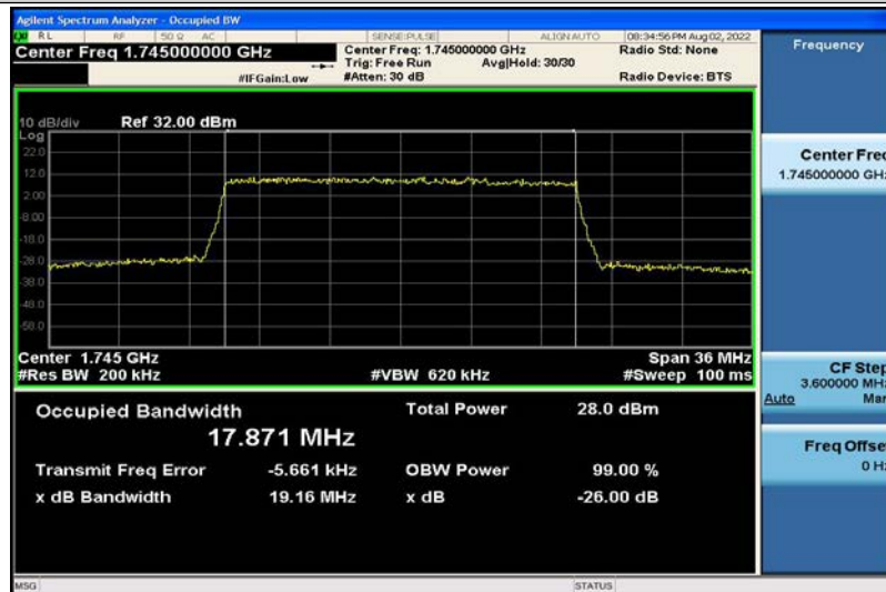
Band4-20MHz-QPSK-20300-100RB#0-17.871
