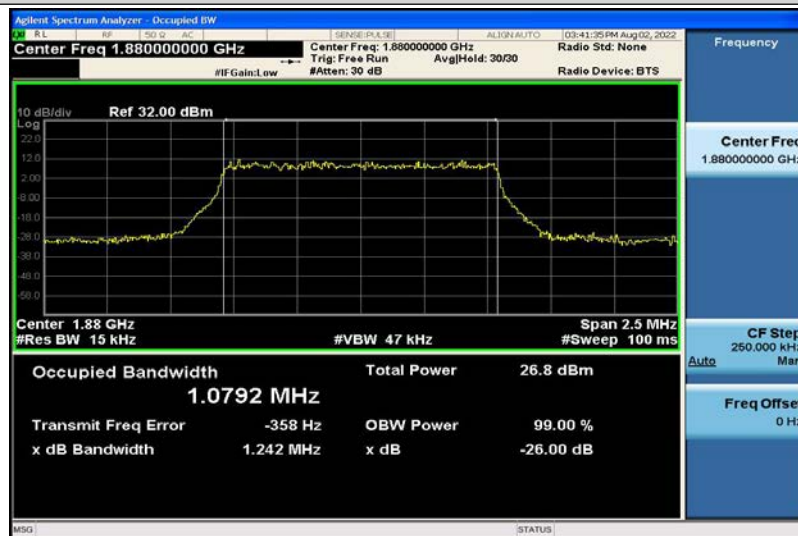
Band2-1.4MHz-16QAM-18900-6RB#0-1.0792
