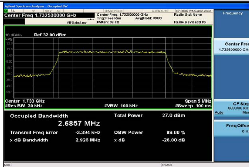
Band4-3MHz-16QAM-20175-15RB#0-2.6857
