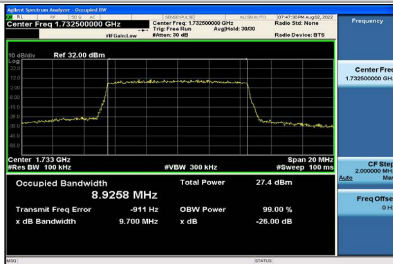
Band4-10MHz-16QAM-20175-50RB#0-8.9258
