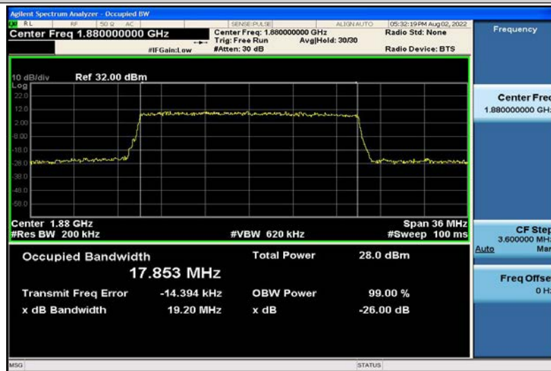
Band2-20MHz-16QAM-18900-100RB#0-17.853
