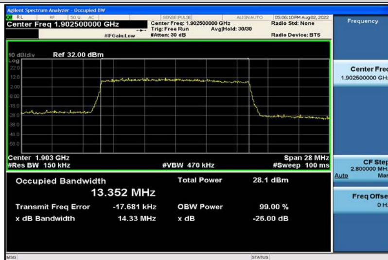
Band2-15MHz-QPSK-19125-75RB#0-13.352
