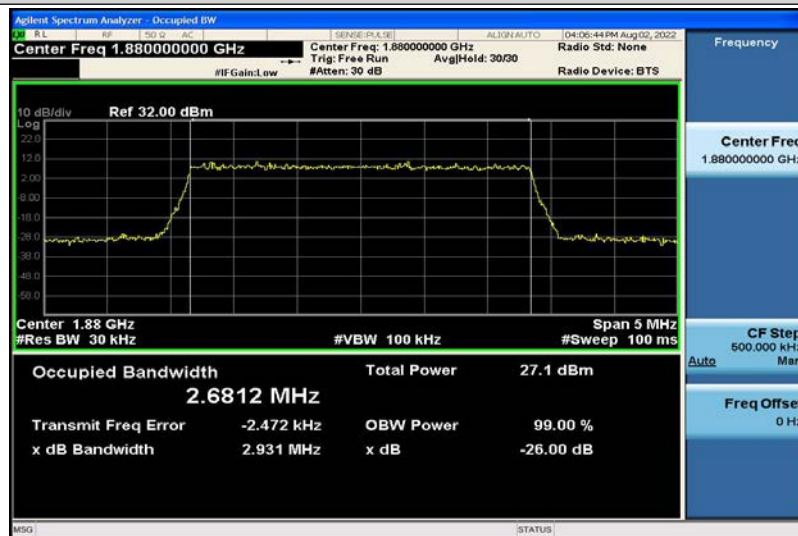
Band2-3MHz-16QAM-18900-15RB#0-2.6812
