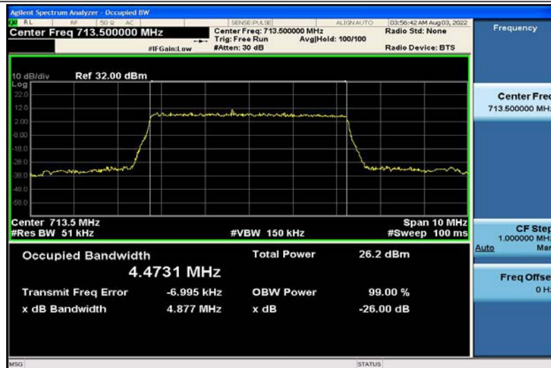
Band12-5MHz-16QAM-23155-25RB#0-4.4731
