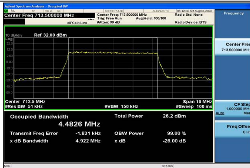
Band17-5MHz-16QAM-23825-25RB#0-4.4826
