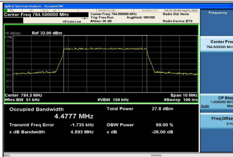
Band13-5MHz-QPSK-23255-25RB#0-4.4777
