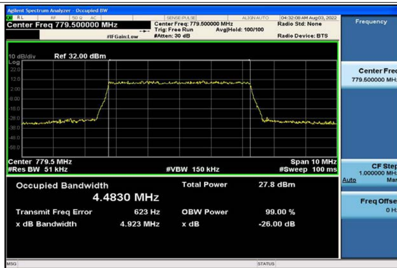
Band13-5MHz-QPSK-23205-25RB#0-4.4830
