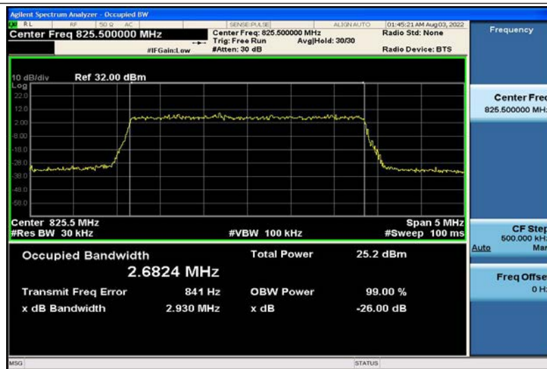
Band5-3MHz-16QAM-20415-15RB#0-2.6824
