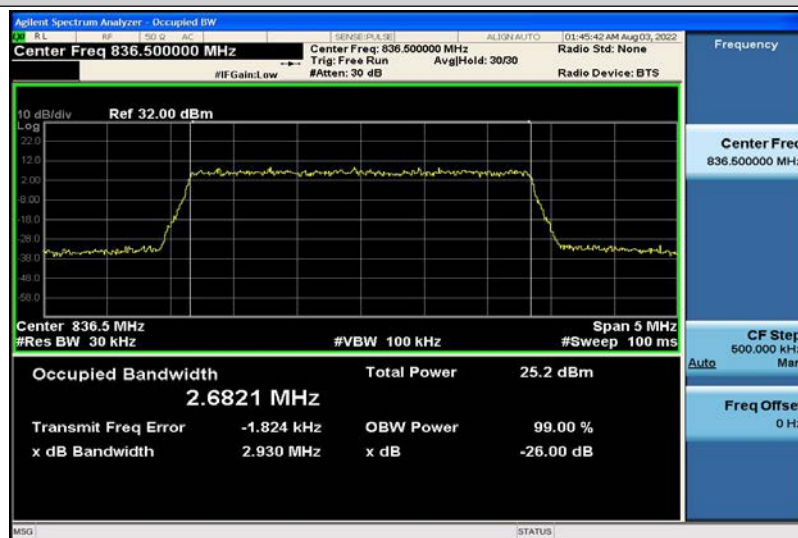
Band5-3MHz-16QAM-20525-15RB#0-2.6821
