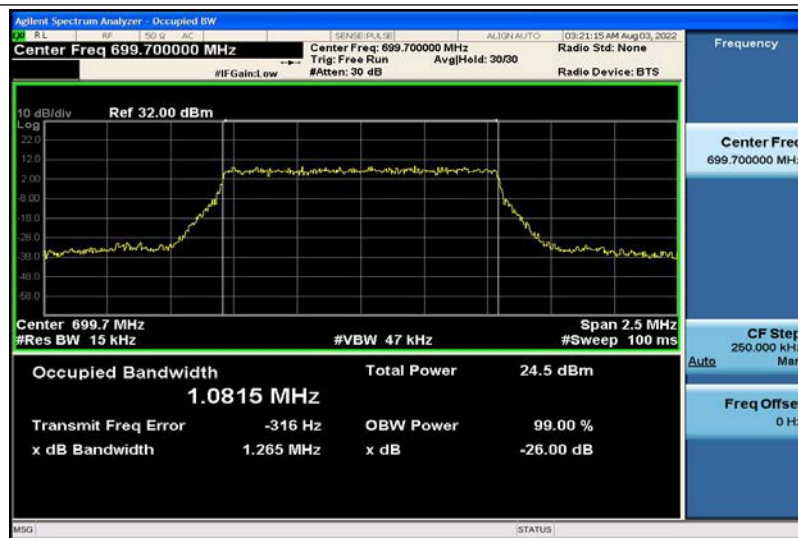
Band12-1.4MHz-16QAM-23017-6RB#0-1.0815
