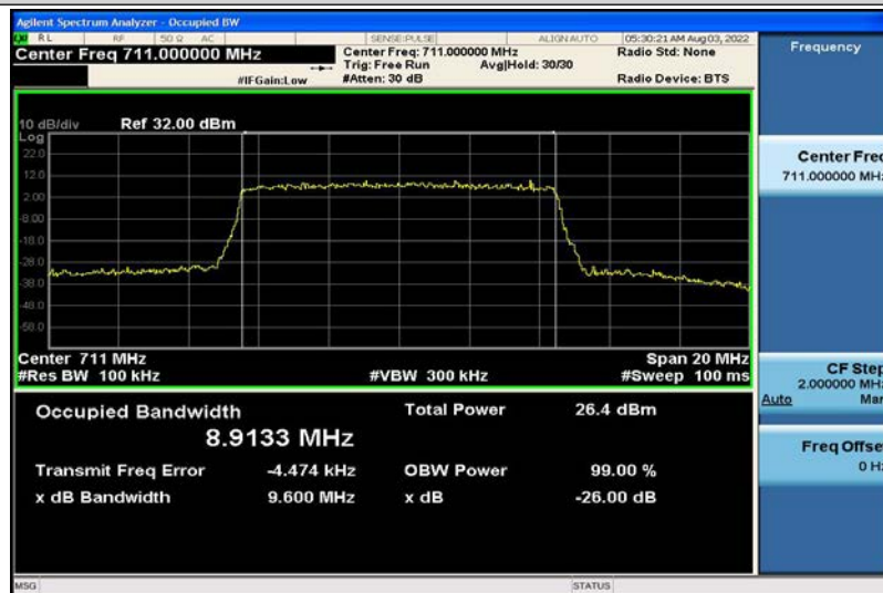
Band17-10MHz-16QAM-23800-50RB#0-8.9133
