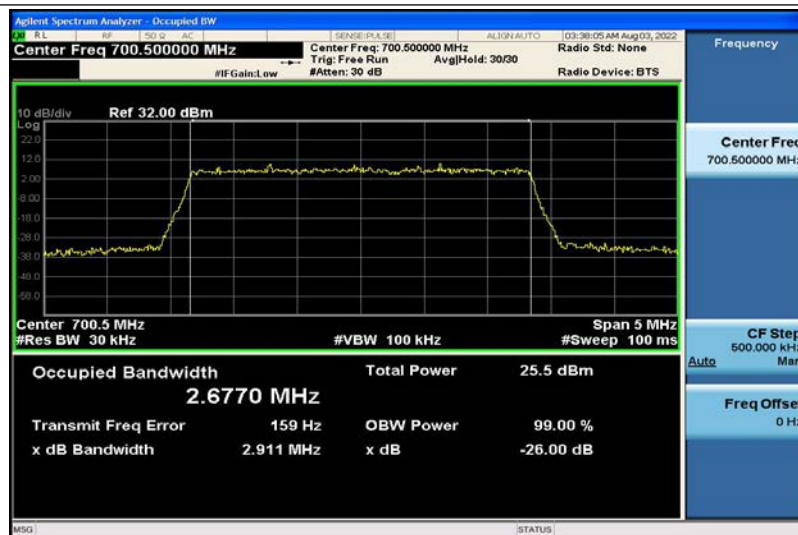
Band12-3MHz-QPSK-23025-15RB#0-2.6770
