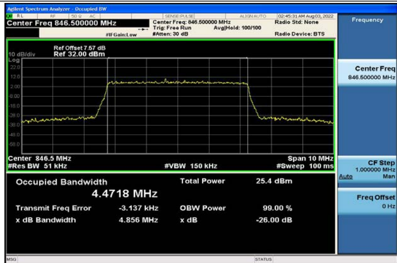
Band5-5MHz-16QAM-20625-25RB#0-4.4718
