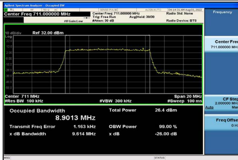
Band12-10MHz-16QAM-23130-50RB#0-8.9013
