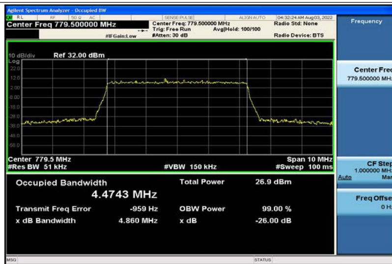
Band13-5MHz-16QAM-23205-25RB#0-4.4743
