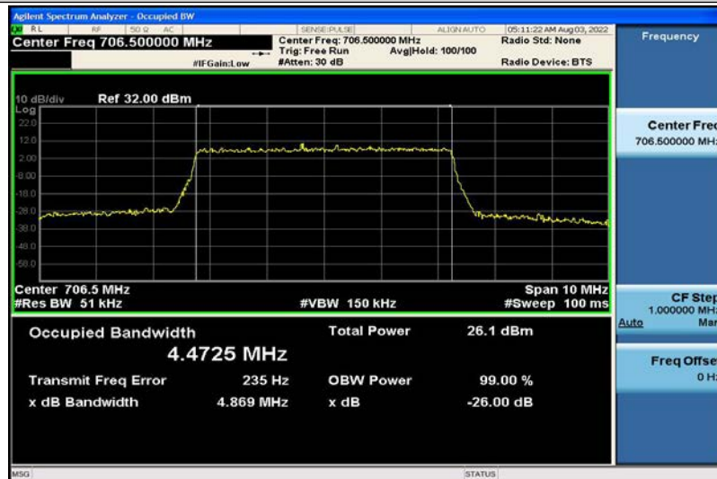
Band17-5MHz-16QAM-23755-25RB#0-4.4725
