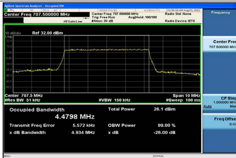
Band12-5MHz-16QAM-23095-25RB#0-4.4798
