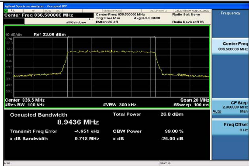
Band5-10MHz-QPSK-20525-50RB#0-8.9436
