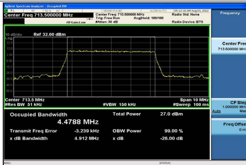
Band17-5MHz-QPSK-23825-25RB#0-4.4788
