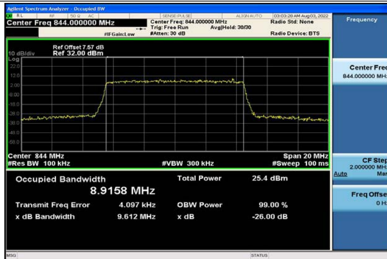
Band5-10MHz-16QAM-20600-50RB#0-8.9158
