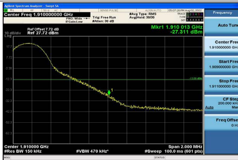
Band2-15MHz-QPSK-19125-1RB#74
