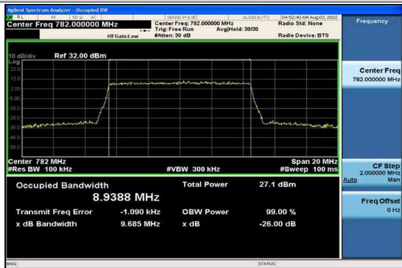
Band13-10MHz-16QAM-23230-50RB#0-8.9388
