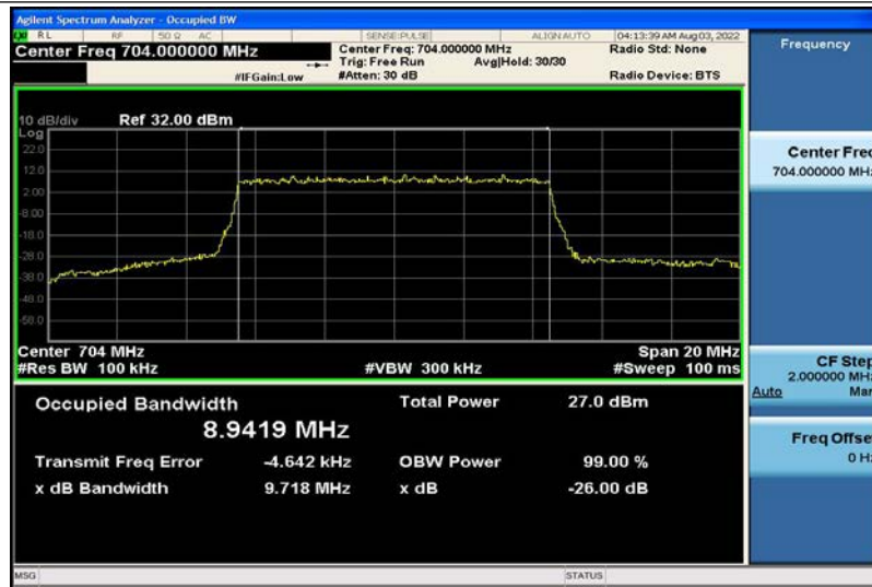
Band12-10MHz-QPSK-23060-50RB#0-8.9419
