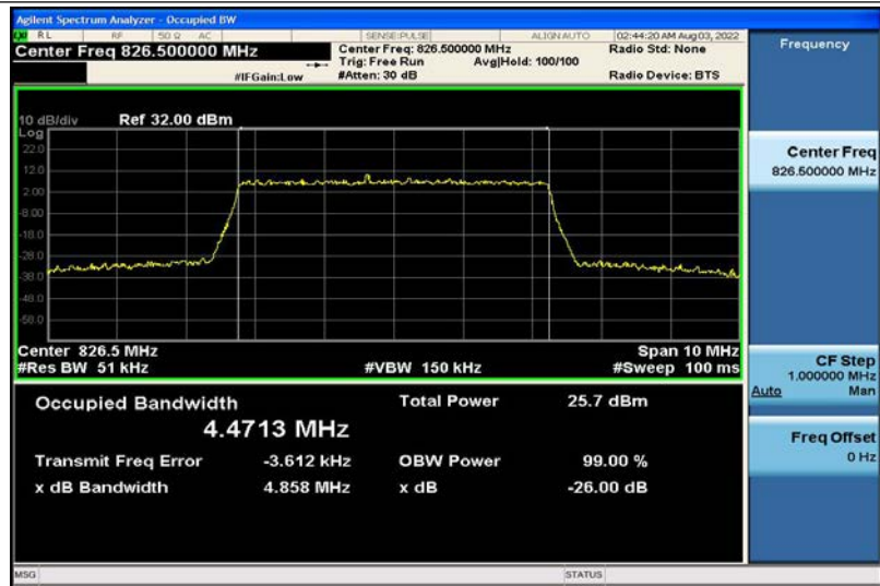
Band5-5MHz-16QAM-20425-25RB#0-4.4713
