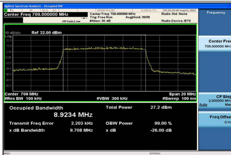
Band17-10MHz-QPSK-23780-50RB#0-8.9234
