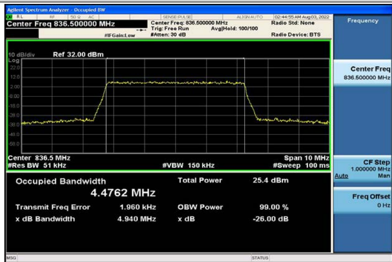
Band5-5MHz-16QAM-20525-25RB#0-4.4762
