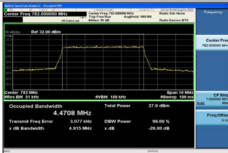
Band13-5MHz-QPSK-23230-25RB#0-4.4708
