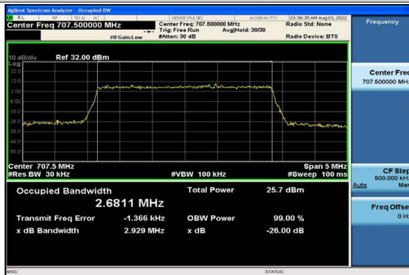
Band12-3MHz-16QAM-23095-15RB#0-2.6811
