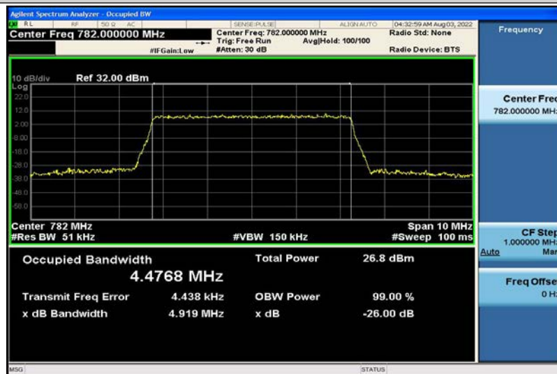
Band13-5MHz-16QAM-23230-25RB#0-4.4768
