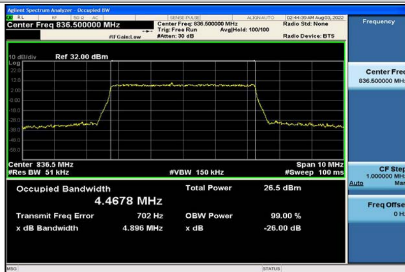
Band5-5MHz-QPSK-20525-25RB#0-4.4678
