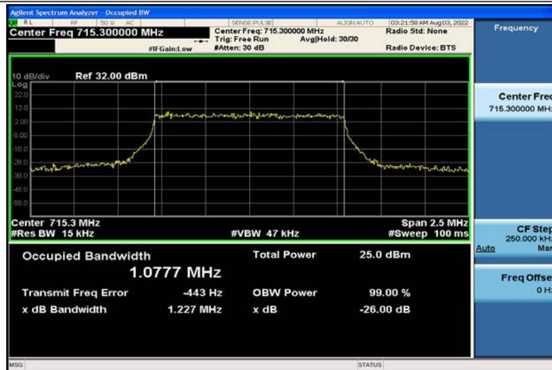
Band12-1.4MHz-16QAM-23173-6RB#0-1.0777
