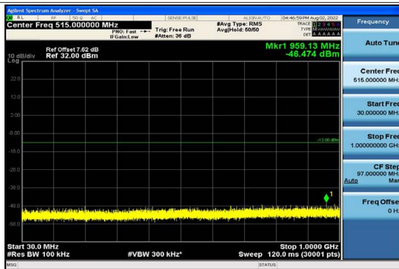
Band2-10MHz-QPSK-18650-1RB#0-30~1000MHz
