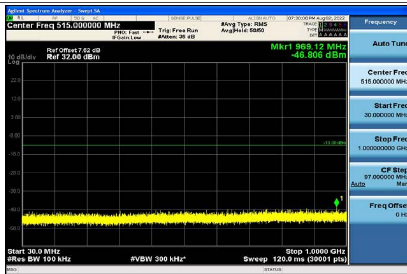
Band4-5MHz-16QAM-19975-1RB#0-30~1000MHz
