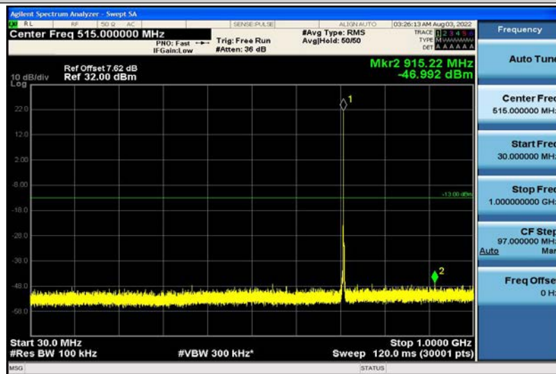
Band12-1.4MHz-QPSK-23173-1RB#0-30~1000MHz
