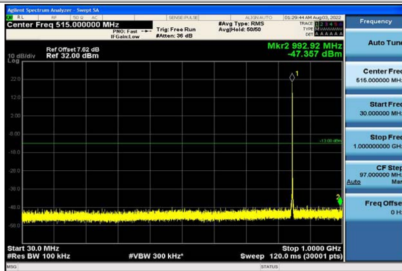
Band5-1.4MHz-QPSK-20643-1RB#0-30~1000MHz
