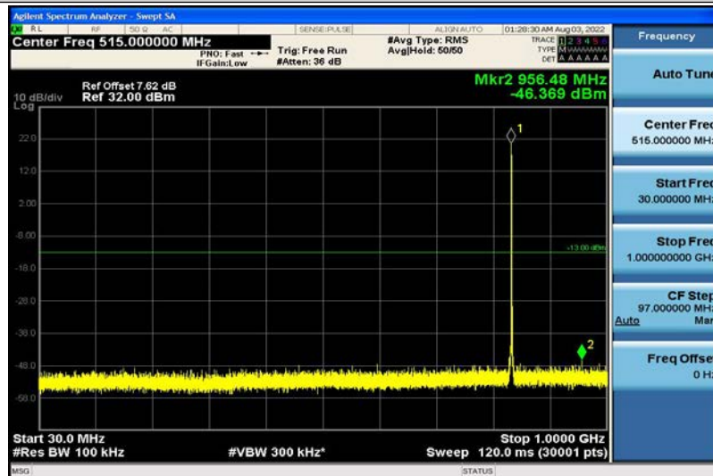
Band5-1.4MHz-QPSK-20525-1RB#0-30~1000MHz
