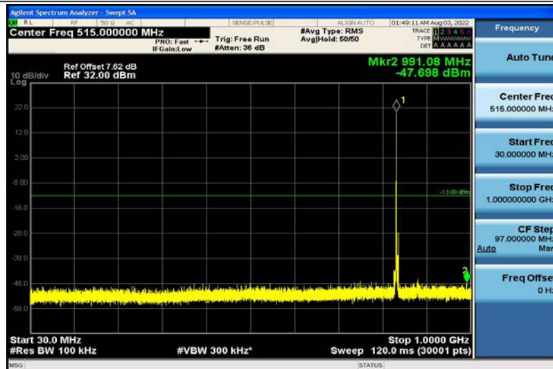
Band5-3MHz-QPSK-20525-1RB#0-30~1000MHz
