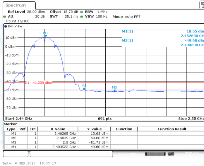
11B_Ant2_High_2462_Peak
