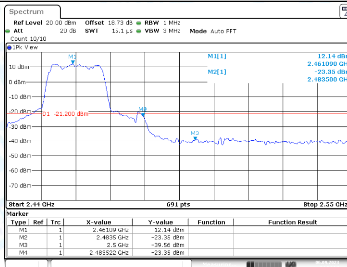
11N20MIMO_Ant2_High_2462_Peak
