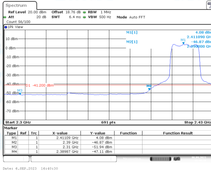
11G_Ant2_Low_2412_Peak
