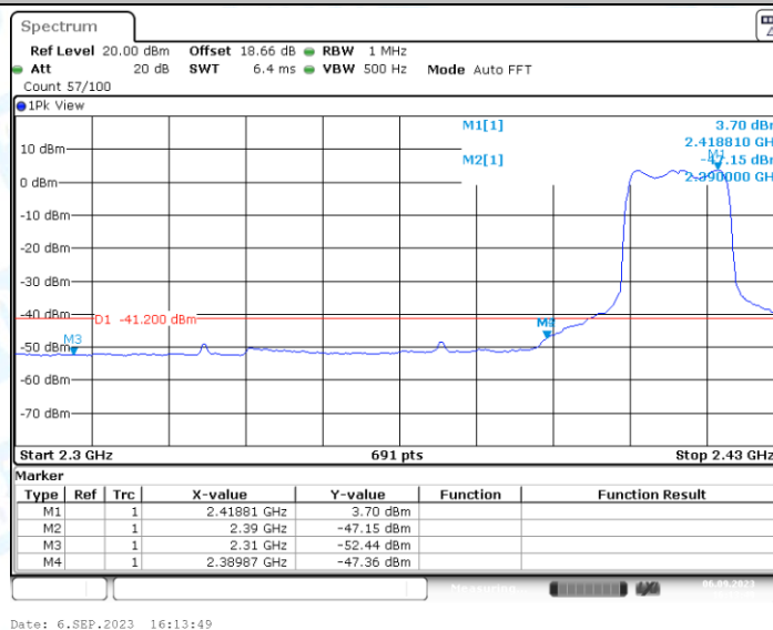
11G_Ant1_Low_2412_Peak
