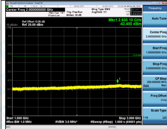
Band2_10MHz_QPSK_18900_50RB#0_1000~3000_1000~3000
