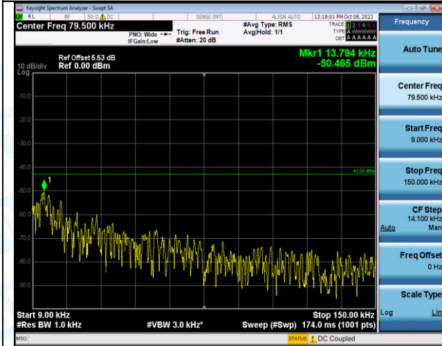
Band2_15MHz_16QAM_18900_1RB#74_0.009~0.15_0.00 9~0.15
