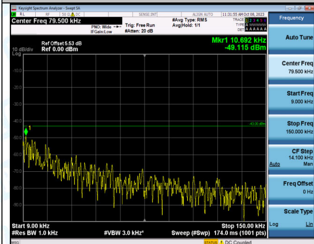
Band2_10MHz_QPSK_19150_50RB#0_0.009~0.15_0.009~0.15
