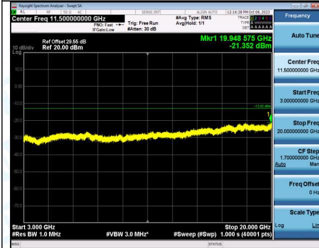
Band2_15MHz_16QAM_18900_1RB#0_3000~20000_300 0~20000
