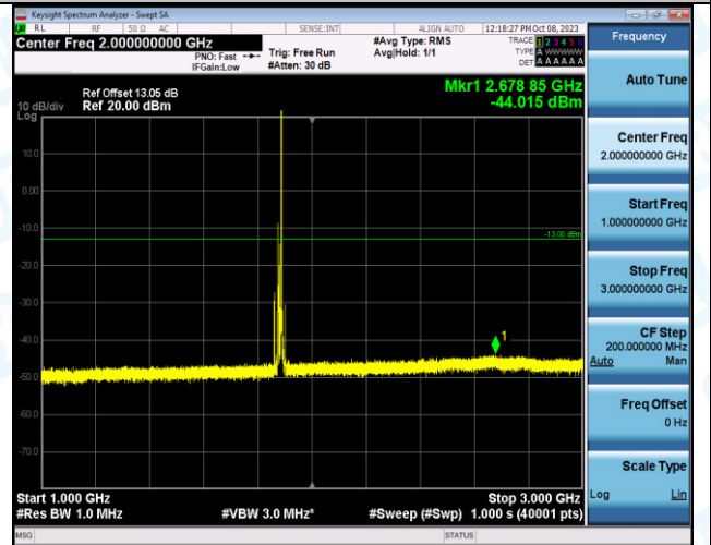
Band2_15MHz_16QAM_18900_1RB#74_1000~3000_100 0~3000
