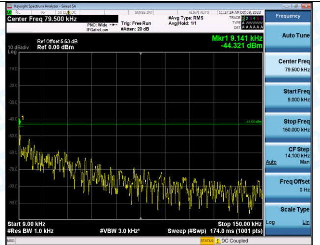
Band2_10MHz_16QAM_19150_1RB#49_0.009~0.15_0.00 9~0.15
