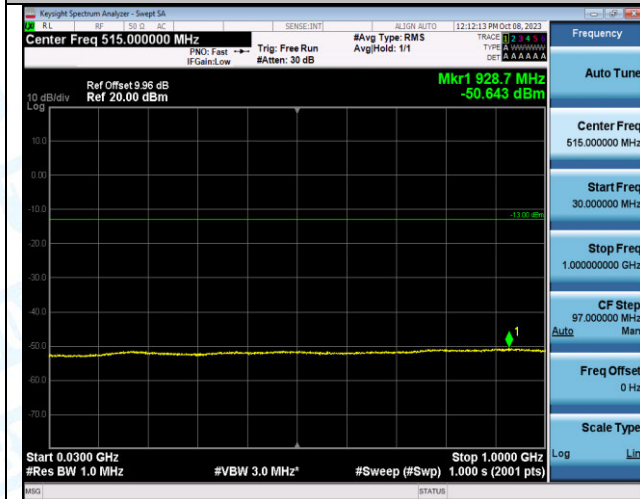
Band2_15MHz_16QAM_18675_1RB#74_30~1000_30~10 00
