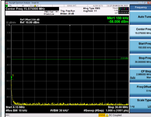
Band2_10MHz_16QAM_19150_1RB#49_0.15~30_0.15~3 0
