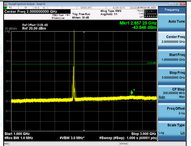
Band2_15MHz_16QAM_18675_1RB#74_1000~3000_100 0~3000
