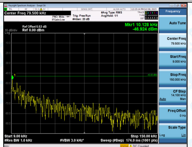
Band2_15MHz_QPSK_18900_1RB#0_0.009~0.15_0.009~0.15 0.15
