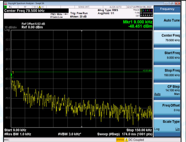
Band2_15MHz_QPSK_18900_1RB#74_0.009~0.15_0.009 ~0.15
