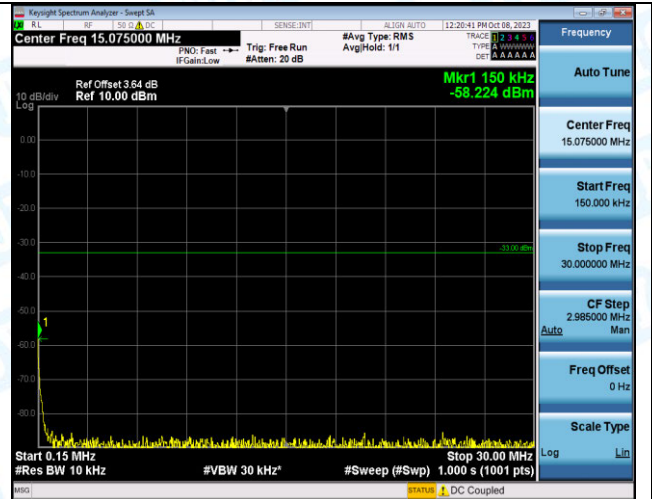
Band2_15MHz_16QAM_19125_1RB#0_0.15~30_0.15~30
