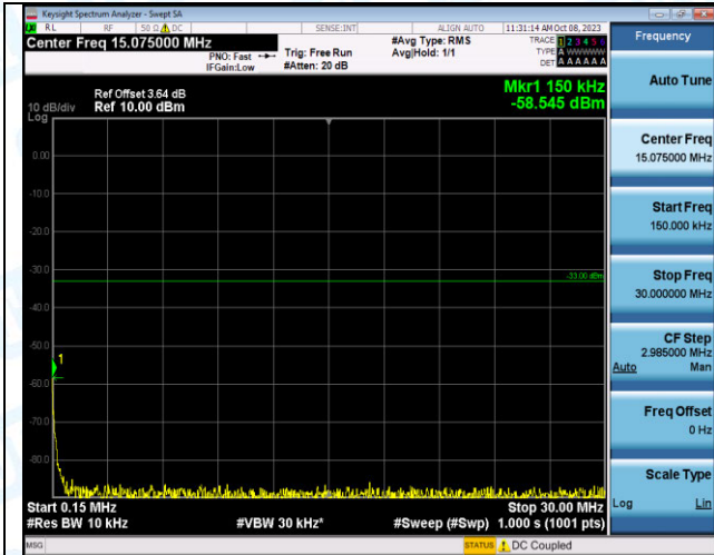
Band2_10MHz_QPSK_18900_50RB#0_0.15~30_0.15~30
