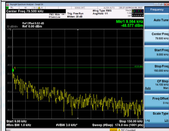
Band4_10MHz_QPSK_20000_1RB#49_0.009~0.15_0.009~0.15
