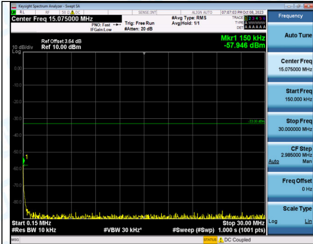
Band4_10MHz_16QAM_20175_1RB#49_0.15~30_0.15~3
