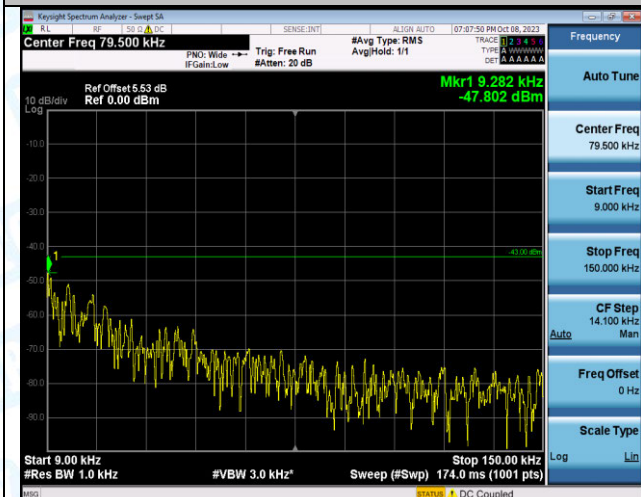
Band4_10MHz_QPSK_20350_1RB#0_0.009~0.15_0.009~
