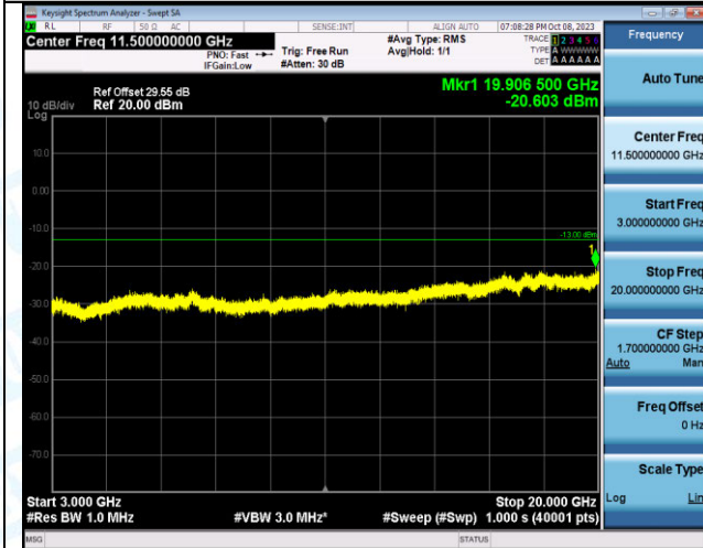
Band4_10MHz_QPSK_20350_1RB#0_3000~20000_3000~20000
