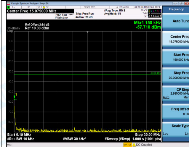
Band4_5MHz_16QAM_20375_25RB#0_0.15~30_0.15~30
