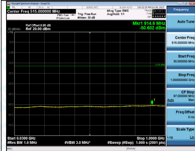
Band4_10MHz_QPSK_20000_1RB#0_30~1000_30~1000
