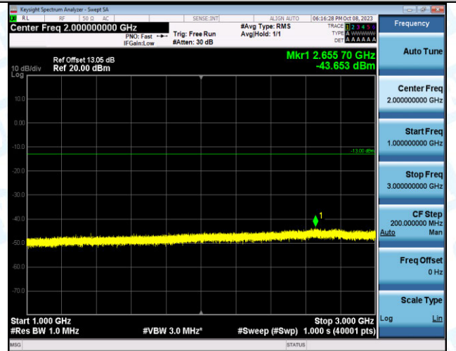
Band4_10MHz_QPSK_20175_1RB#0_1000~3000_1000~3000
