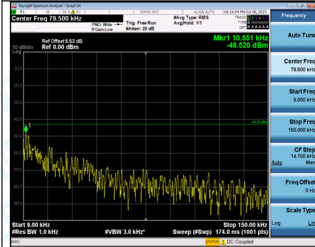
Band4_10MHz_QPSK_20175_1RB#0_0.009~0.15_0.009~0.15
