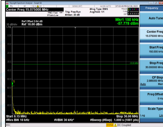
Band4_10MHz_16QAM_20175_1RB#0_0.15~30_0.15~30
