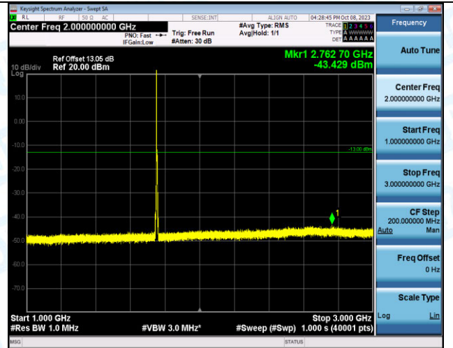
Band4_5MHz_QPSK_20375_1RB#0_1000~3000_1000~3000
