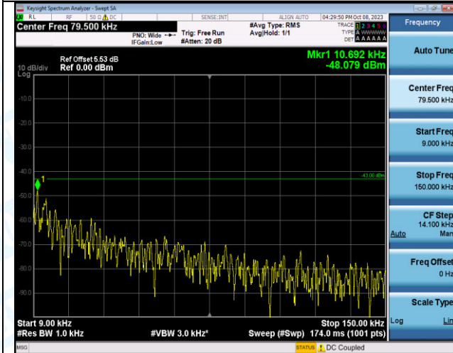
Band4_5MHz_QPSK_20375_25RB#0_0.009~0.15_0.009~0.15
