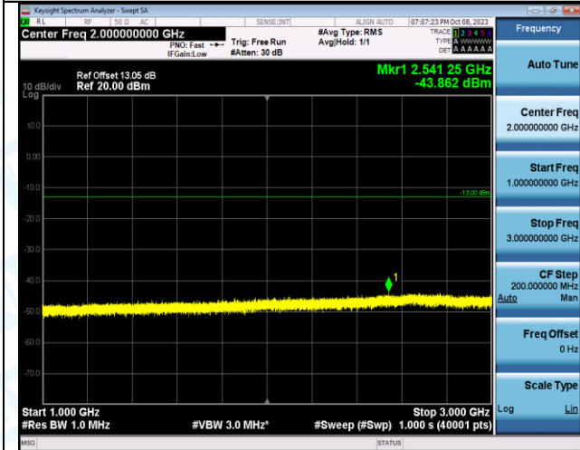
Band4_10MHz_16QAM_20175_1RB#49_1000~3000_100
