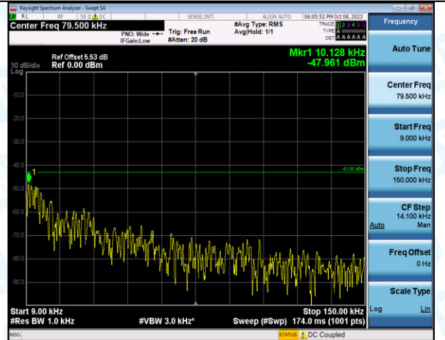
Band4_10MHz_16QAM_20000_1RB#49_0.009~0.15_0.009~0.15 9~0.15
