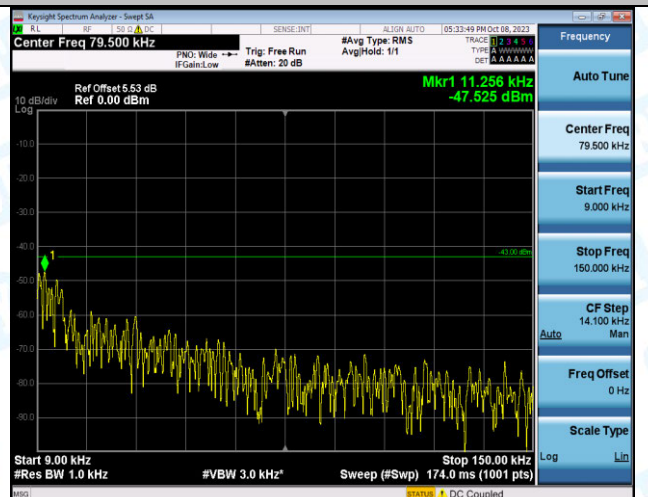
Band4_10MHz_16QAM_20000_1RB#0_0.009~0.15_0.009~0.15
