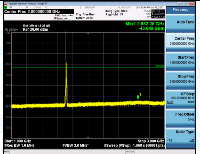
Band4_10MHz_QPSK_20000_1RB#0_1000~3000_1000~3000
