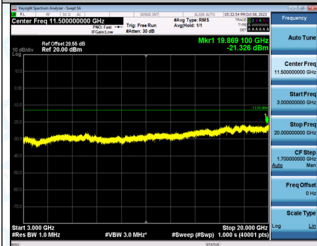
Band4_10MHz_QPSK_20000_1RB#0_3000~20000_3000~20000
