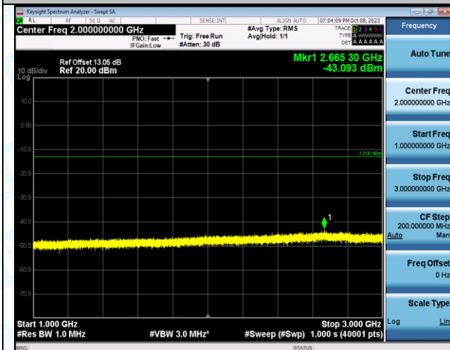
Band4_10MHz_16QAM_20175_1RB#0_1000~3000_1000 ~3000
