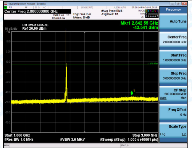
Band4_10MHz_QPSK_20350_1RB#0_1000~3000_1000~3000
