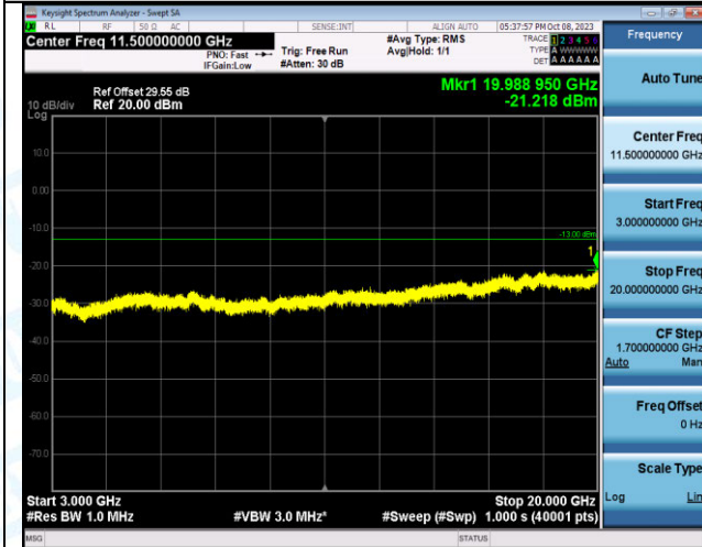
Band4_10MHz_QPSK_20000_1RB#49_3000~20000_3000~20000 0~20000
