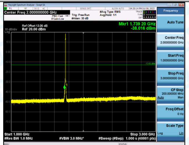
Band4_5MHz_QPSK_20375_25RB#0_1000~3000_1000~3000
