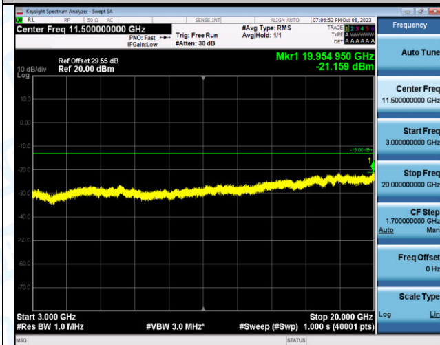
Band4_10MHz_QPSK_20175_1RB#49_3000~20000_3000~20000 0~20000
