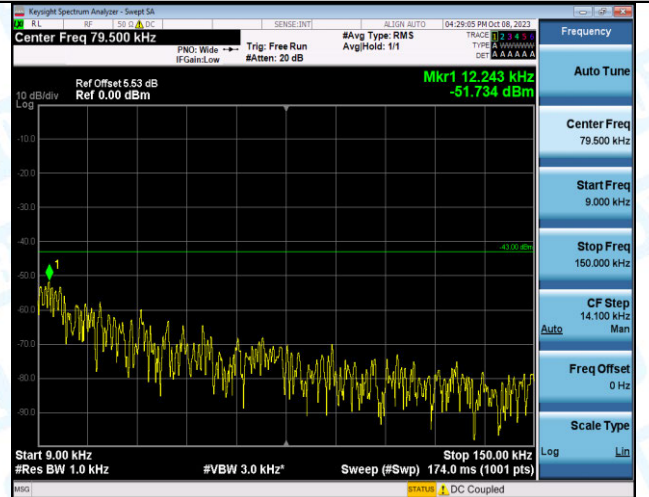
Band4_5MHz_16QAM_20375_1RB#0_0.009~0.15_0.009~0.15
