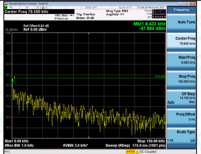
Band4_10MHz_16QAM_20350_1RB#0_0.009~0.15_0.009~0.15
