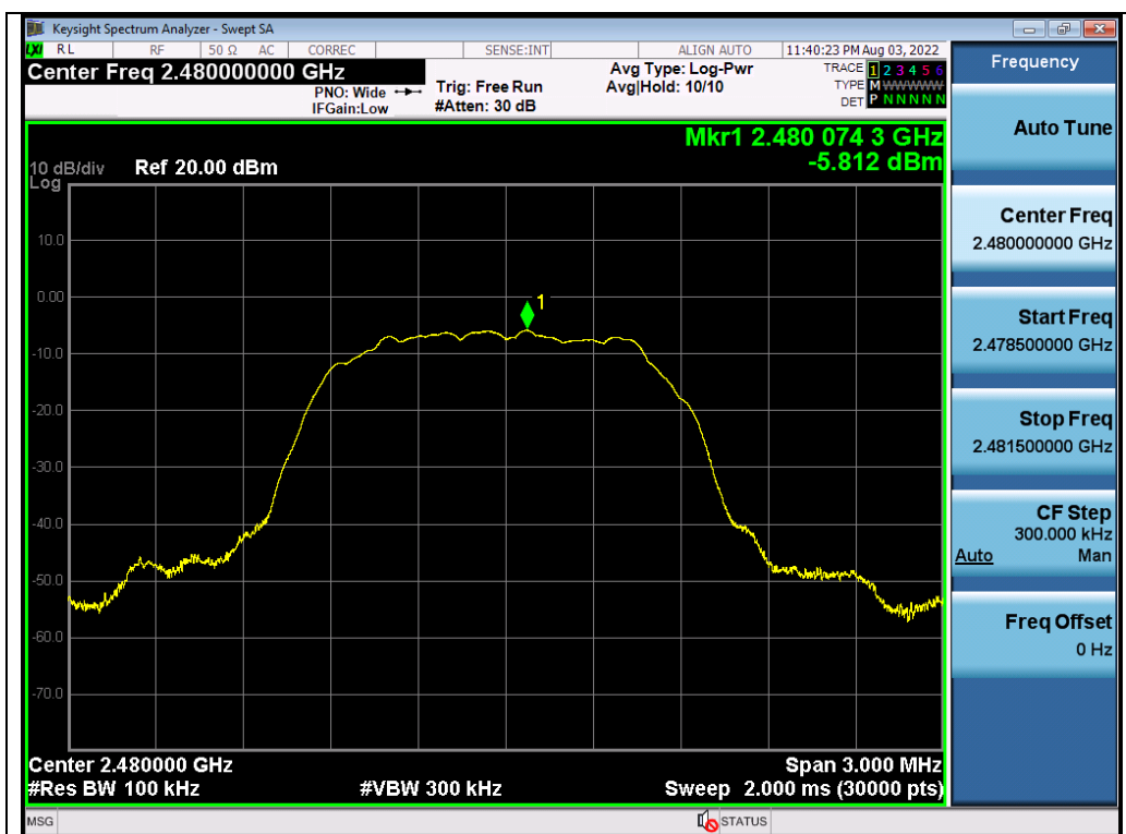
Test Graph EDR ANT1 2480 3Mbps Reference Level
