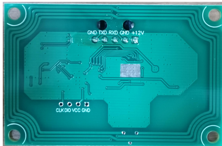
Antenna-Layer View
