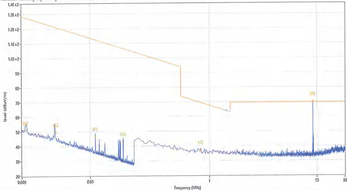
REmission Test case_FCC_Part 15C_FCC TX 9kHz-30MHz (QI&PMA)-1
