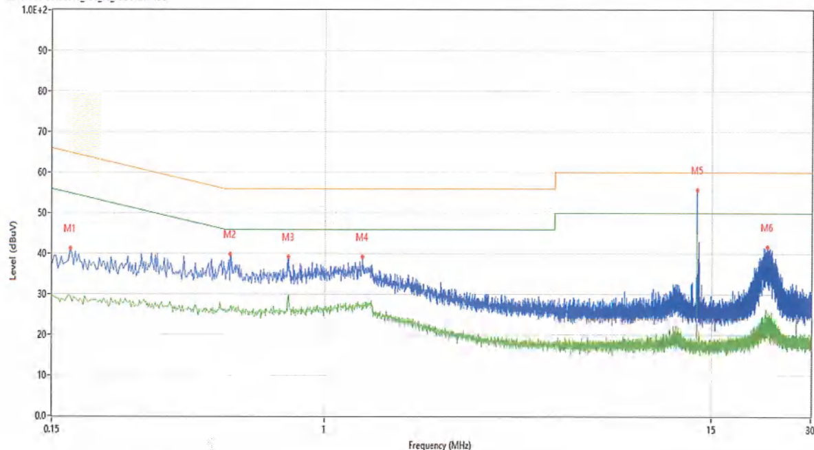
C Emission Test case_FCC_CE_FCC PART 15C
