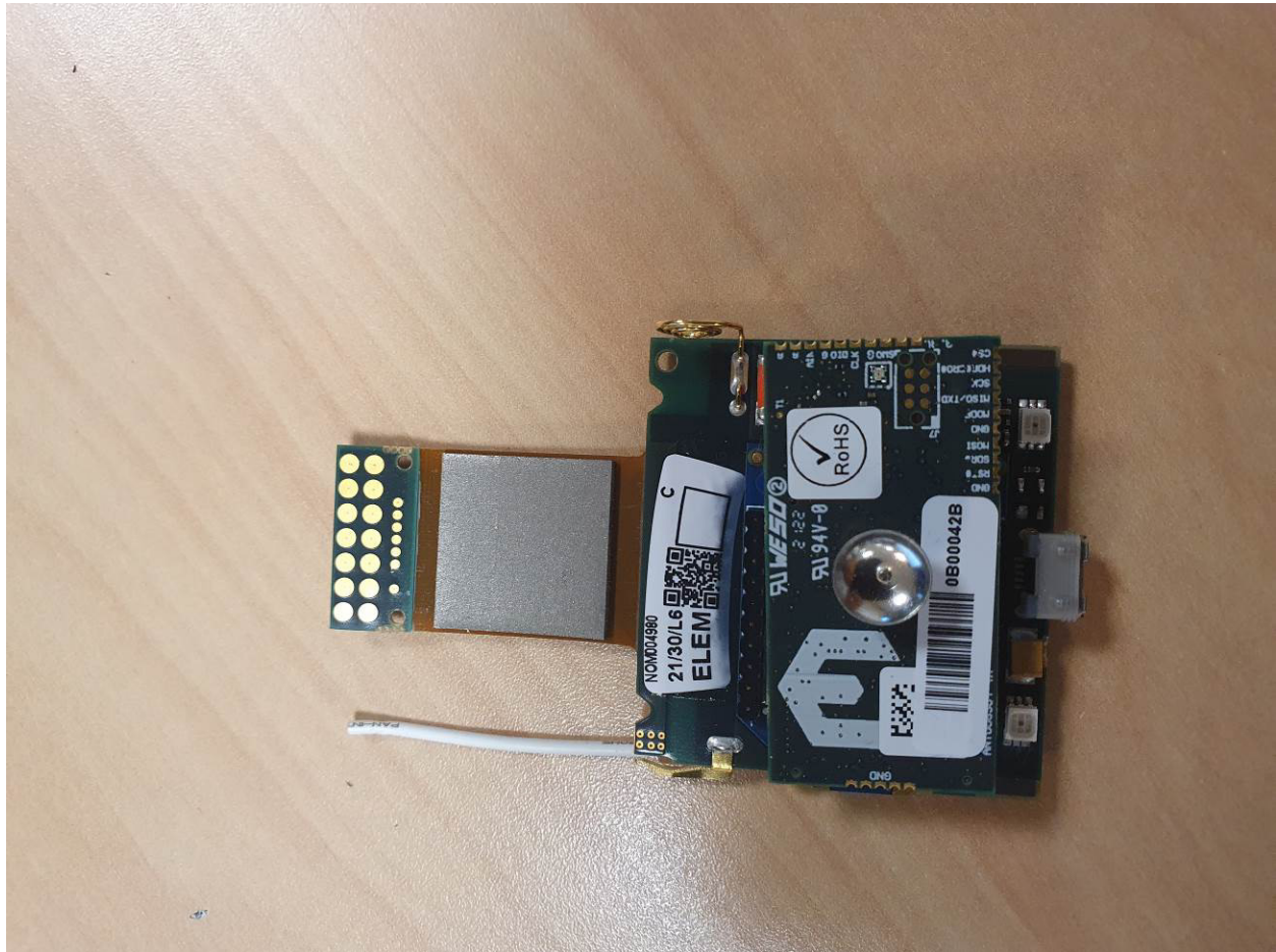
Figure 9. PCBA removed from plastic housing, Top View
