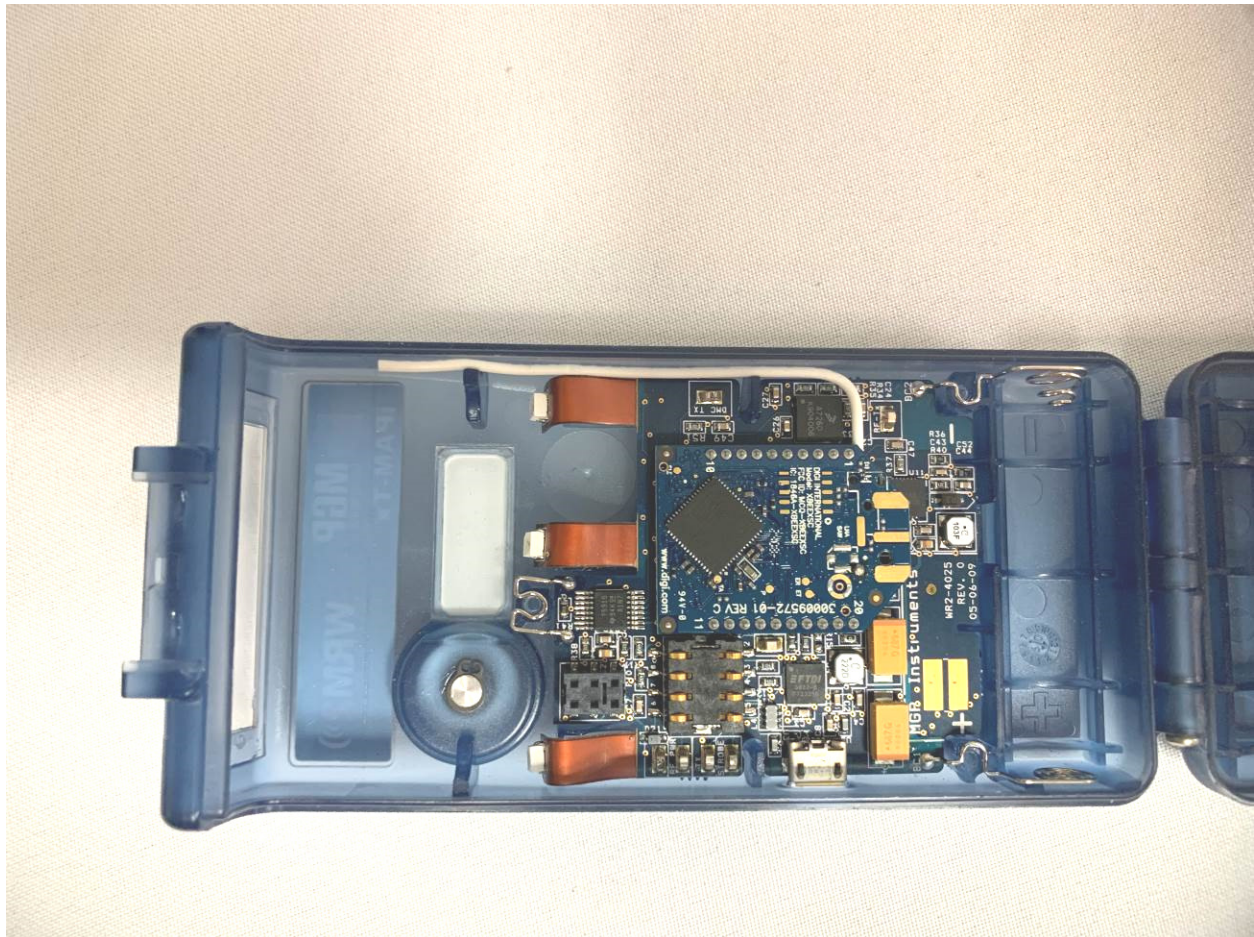
Figure 2. Paper labels removed, Top View
