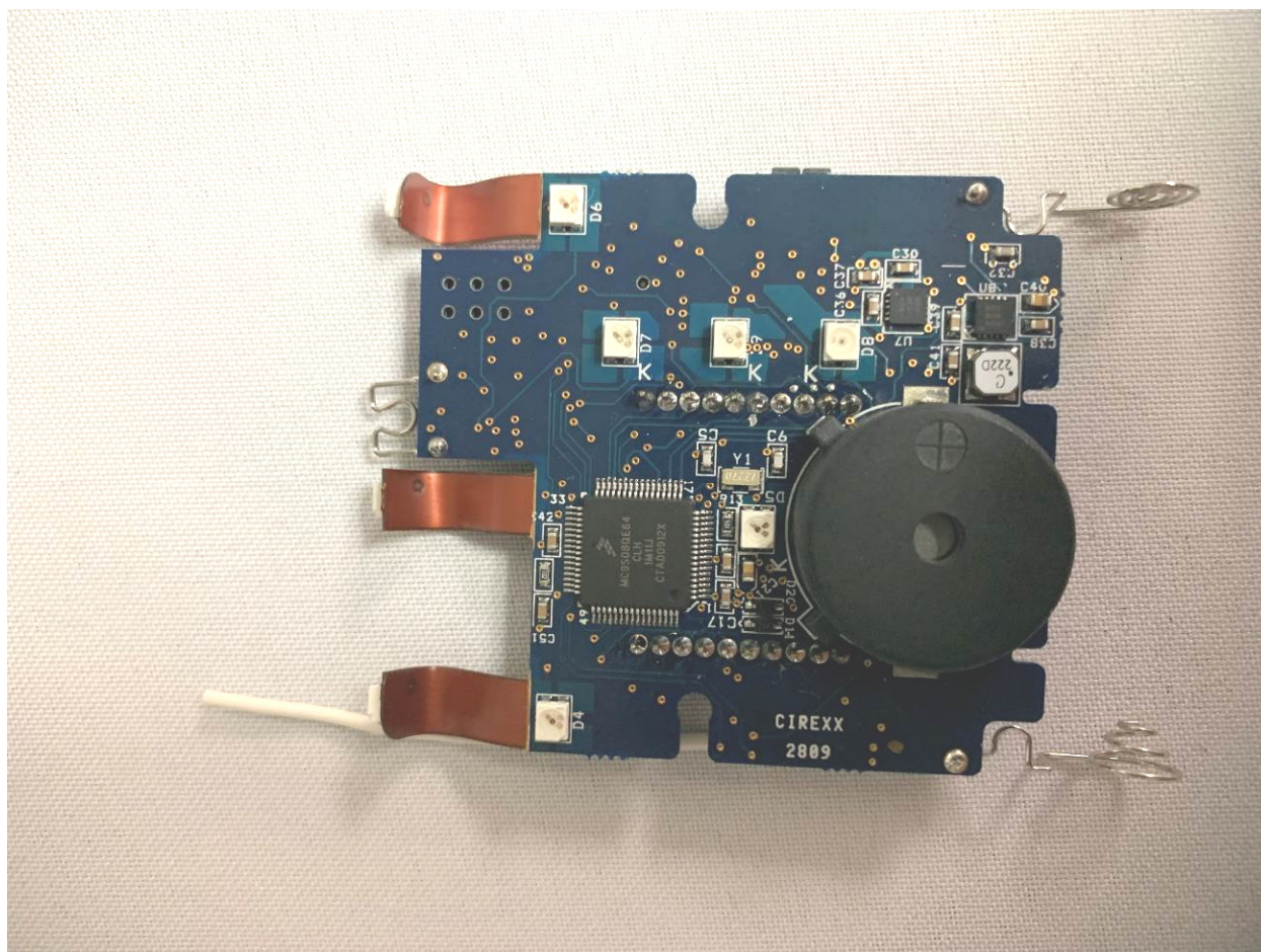
Figure 4. PCBA, Bottom View
