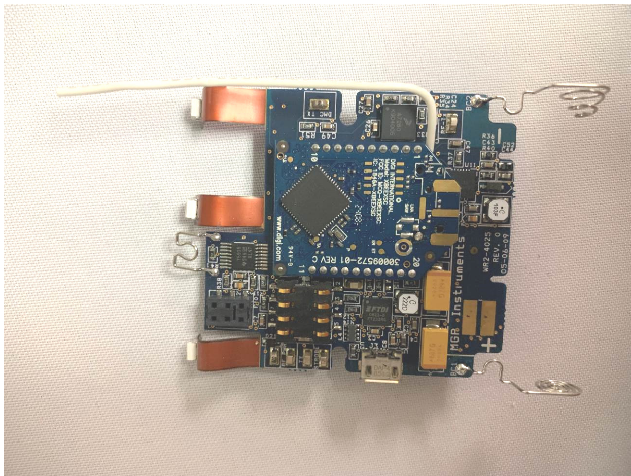
Figure 3. PCBA removed from plastic housing, Top View
