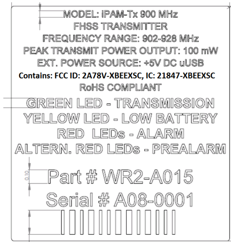
Figure 1. Sample Label for DMC-2000 iPAM Transmitter Module, Part # WR2-A015
