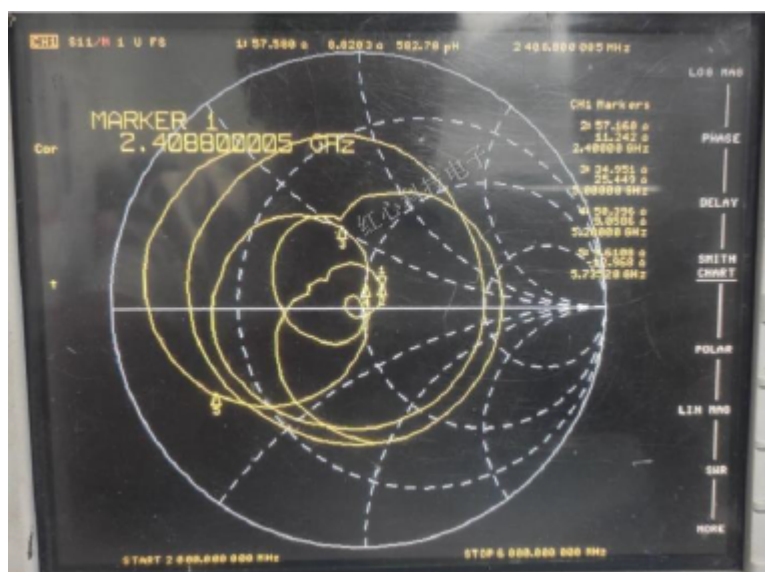
Smith Chart
