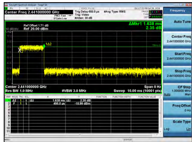
Burst(2DH3)
