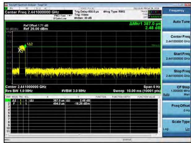
Burst(2DH1)
