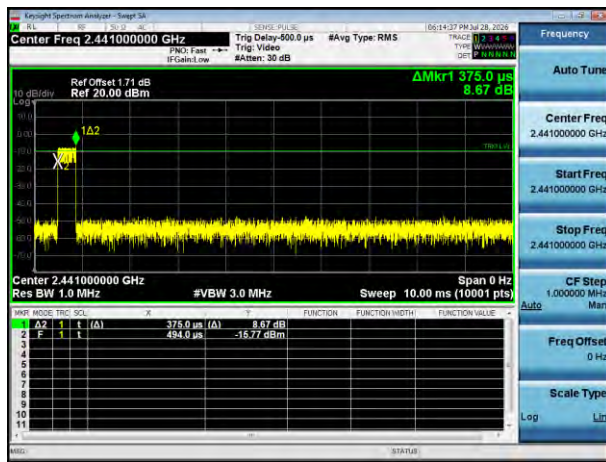
Burst(DH1)
